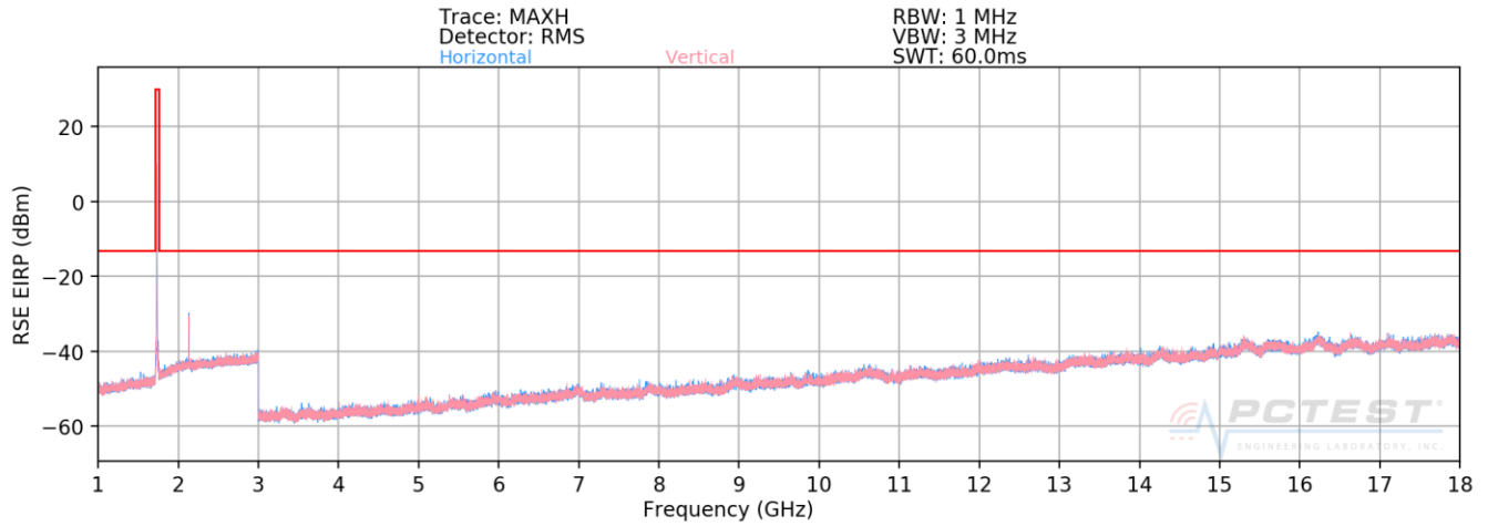
Plot 7-46. Radiated Spurious Emissions above 1GHz (AWS WCDMA Mode – Ch. 1413)
