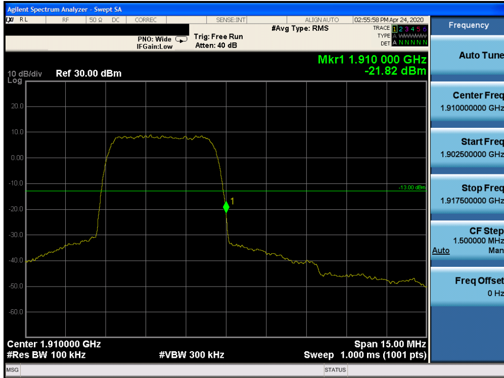
Plot 7-39. Band Edge Plot (PCS WCDMA Mode - High Channel)
