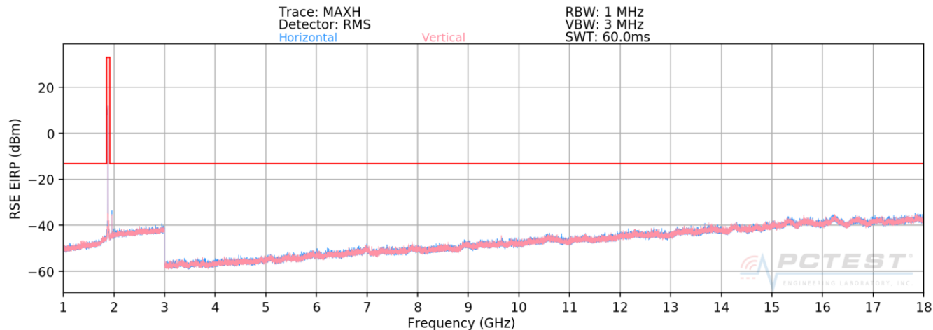
Plot 7-47. Radiated Spurious Plot Emissions 1GHz (PCS WCDMA Mode – Ch. 9400)
