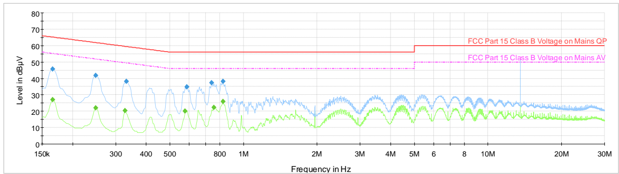
Plot 7-13. AC Line-Conducted Test Plot (N, with WCP + AC/DC Adapter)
