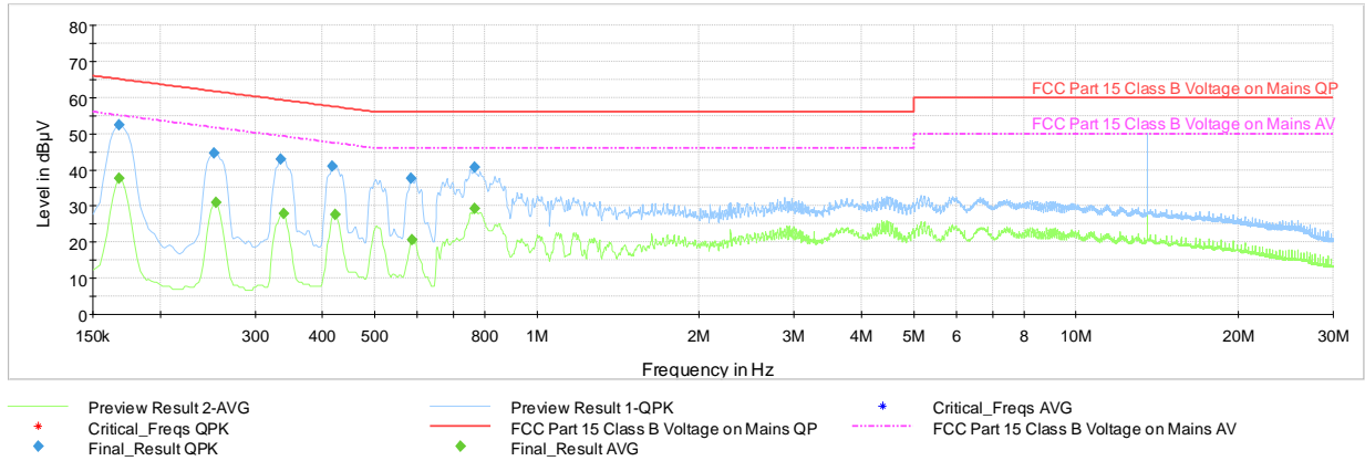
Plot 7-12. AC Line-Conducted Test Plot (L1, with WCP + AC/DC Adapter)
