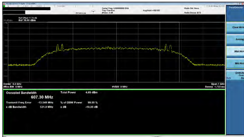
Plot 7-26. ISED Occupied Bandwidth (Ch. 5, Config 1/Payload 125)
