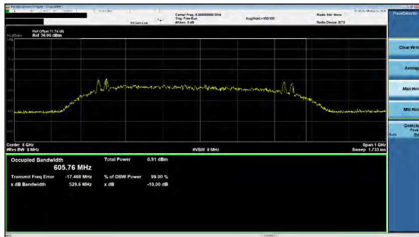
Plot 7-32. ISED Occupied Bandwidth (Ch. 9, Config 0/Payload 65)
