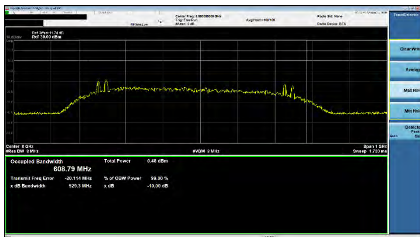
Plot 7-35. ISED Occupied Bandwidth (Ch. 9, Config 1/Payload 85)
