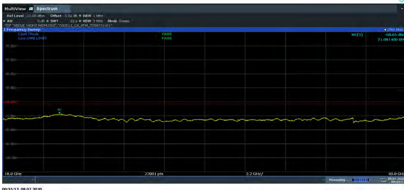
Plot 7-110. Radiated Spurious Emission 18-40GHz (Ch. 9, Config 3, Payload 125 Ant. Pol. V)
