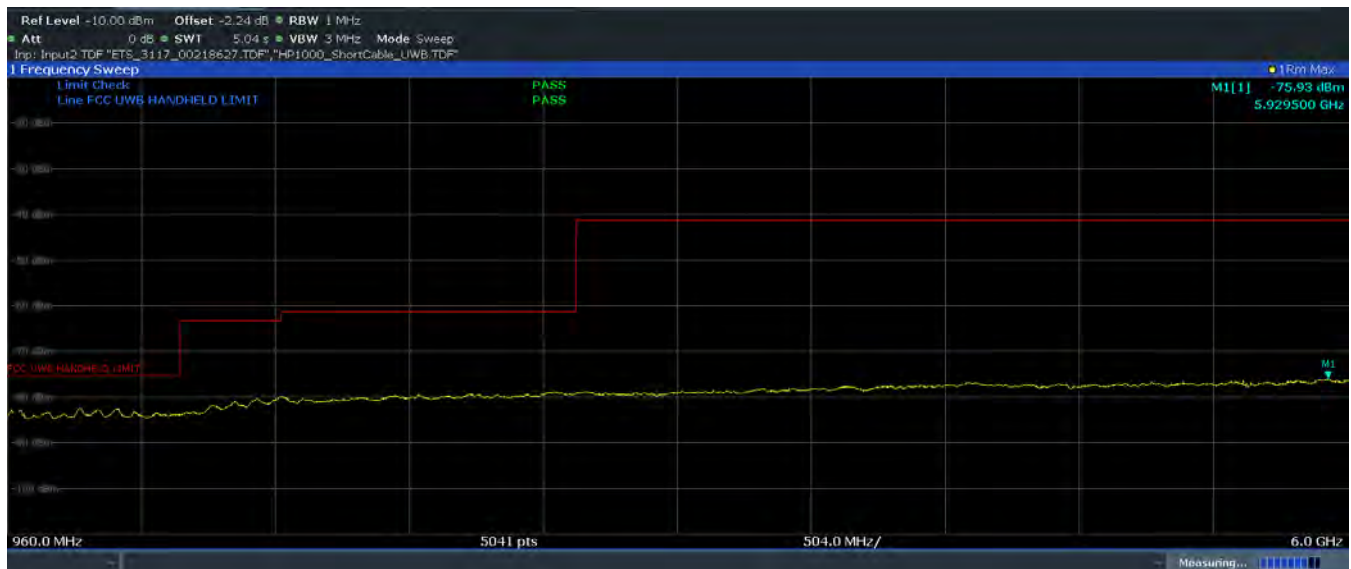
Plot 7-87. FCC Radiated Spurious Emission 960-6000MHz (Ch. 5, Config 3, Payload 125 Ant. Pol. H)
