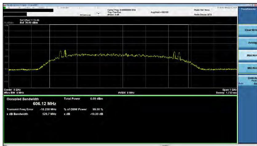
Plot 7-33. ISED Occupied Bandwidth (Ch. 9, Config 0/Payload 125)
