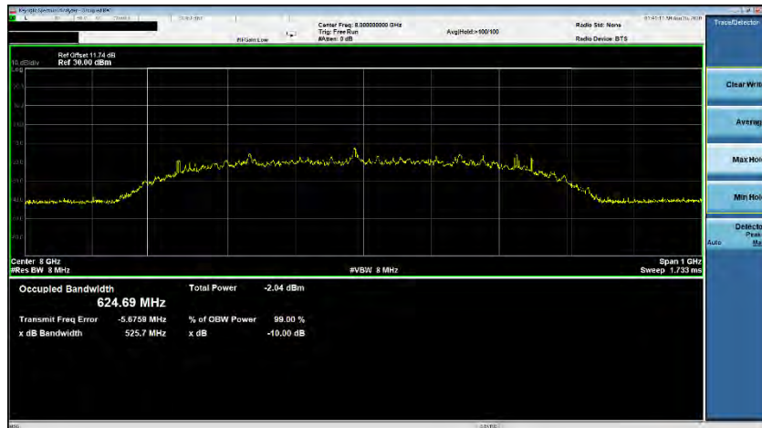
Plot 7-38. ISED Occupied Bandwidth (Ch. 9, Config 3/Payload 125)
