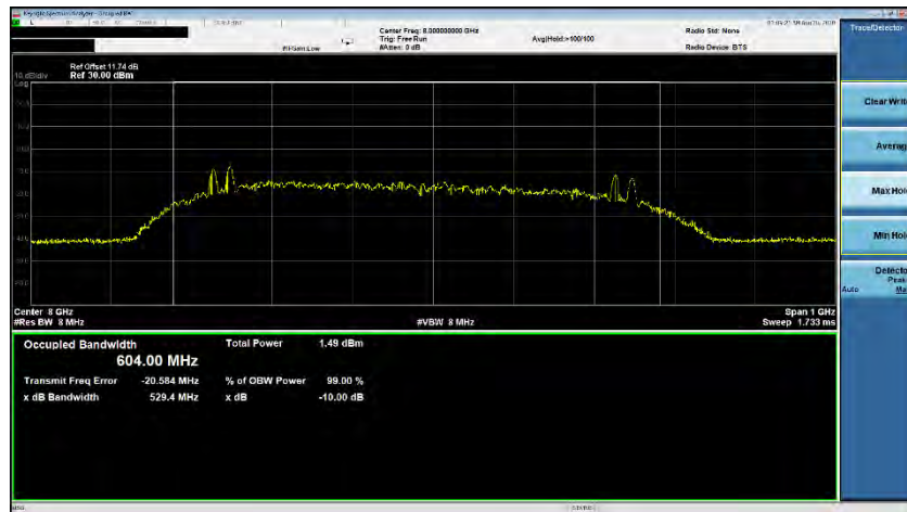
Plot 7-31. ISED Occupied Bandwidth (Ch. 9, Config 0/Payload 25)
