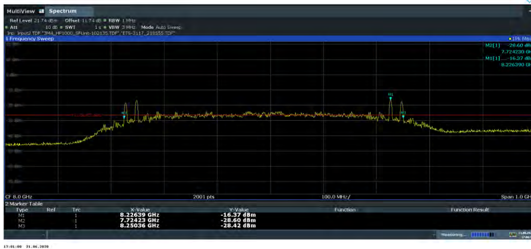
Plot 7-15. 10dBc Bandwidth (Ch. 9, Config 1/Payload 85)
