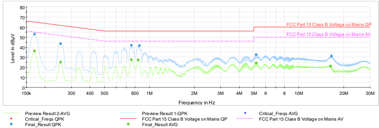
Plot 7-113. AC Line Conducted (Ch. 5, Config 3, Payload 125 L1, with AC/DC Adapter)
