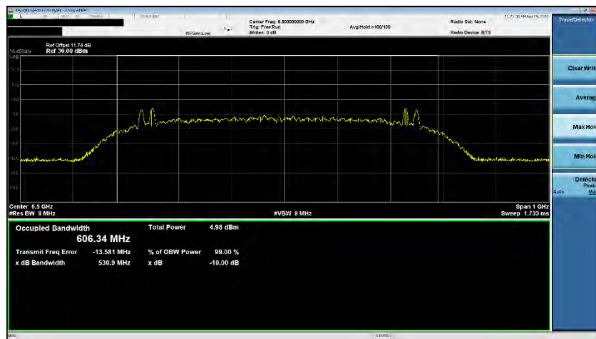
Plot 7-22. ISED Occupied Bandwidth (Ch. 5, Config 0/Payload 65)
