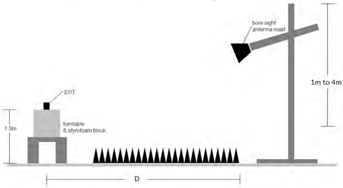
Figure 7-5. Radiated Test Setup - Above 960MHz
