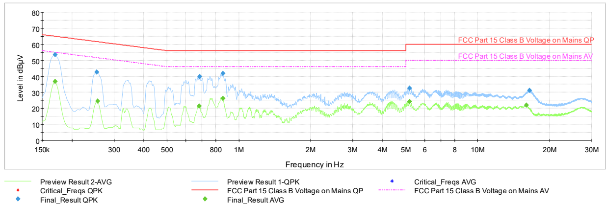
Plot 7-115. AC Line Conducted (Ch. 9, Config 3, Payload 125 L1, with AC/DC Adapter)
