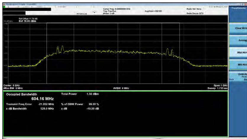
Plot 7-34. ISED Occupied Bandwidth (Ch. 9, Config 1/Payload 45)
