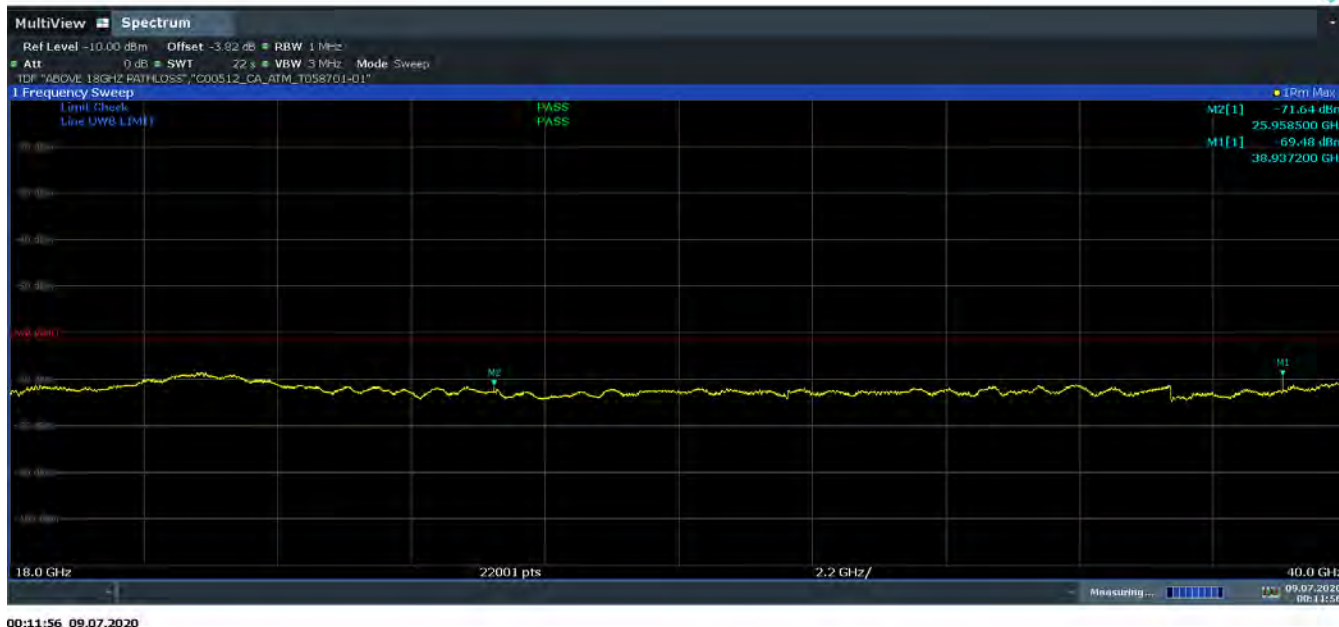
Plot 7-108. Radiated Spurious Emission 18-40GHz (Ch. 5, Config 3, Payload 125 Ant. Pol. V)
