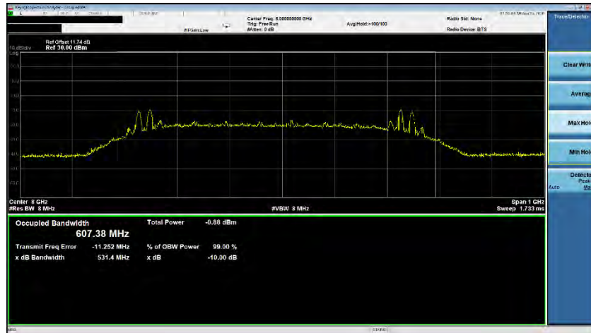
Plot 7-40. ISD Occupied Bandwidth (Ch. 9, Config 5/Payload 0)
