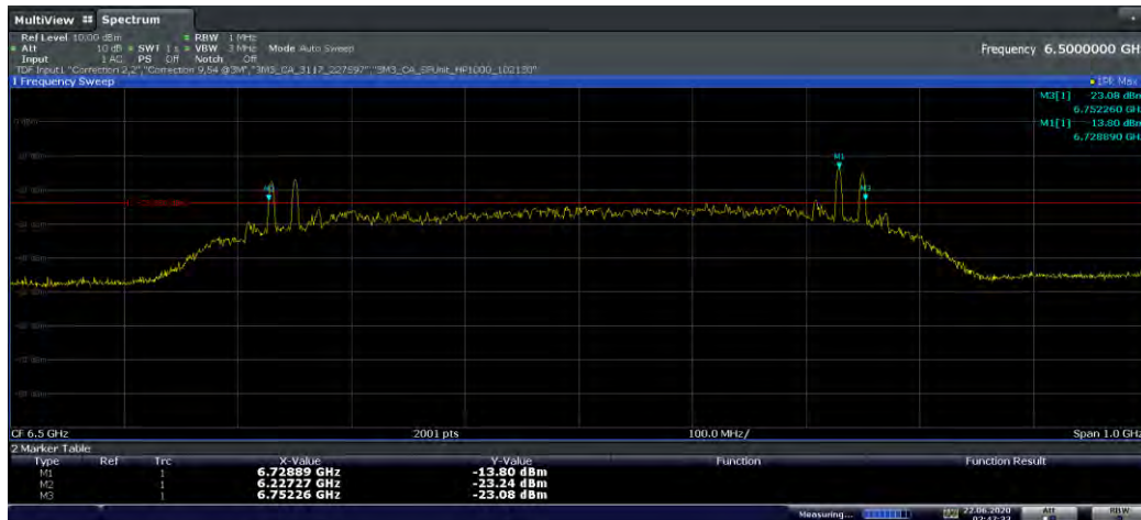
Plot 7-4. 10dBc Bandwidth (Ch. 5, Config 1/Payload 45)
