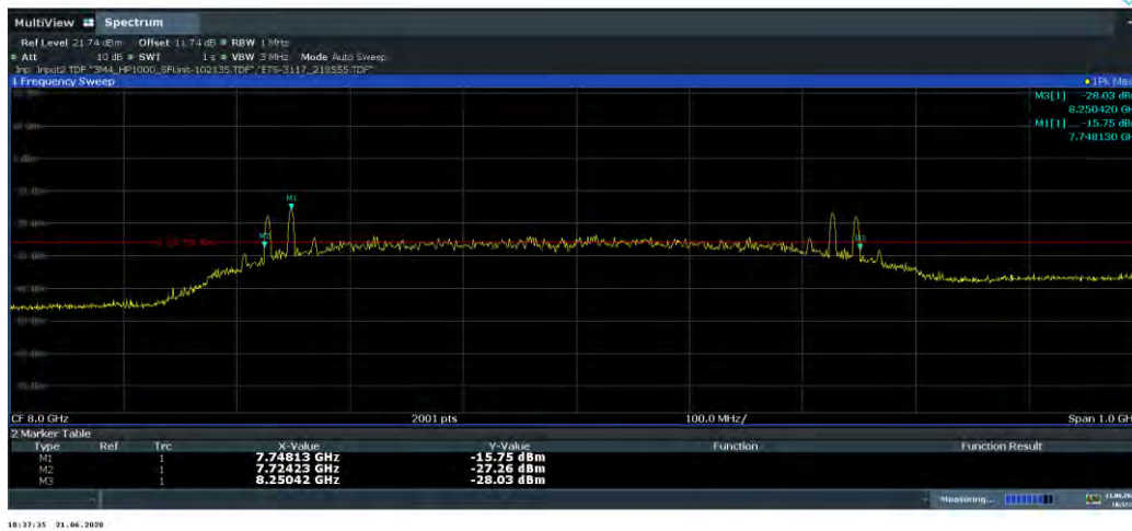
Plot 7-11. 10dBc Bandwidth (Ch. 9, Config 0/Payload 25)
