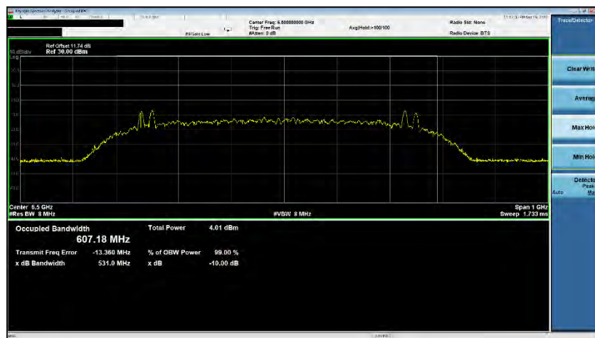
Plot 7-23. ISED Occupied Bandwidth (Ch. 5, Config 0/Payload 125)
