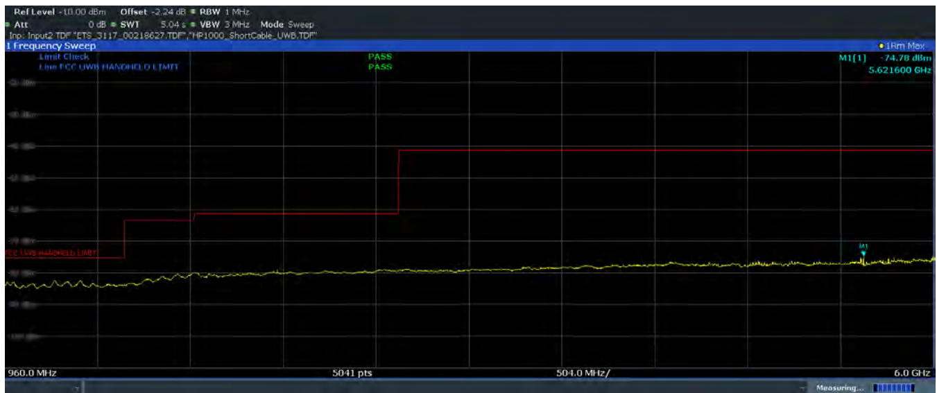
Plot 7-88. FCC Radiated Spurious Emissions 960-6000MHz (Ch. 5, Config 3, Payload 125 Ant. Pol. V)
