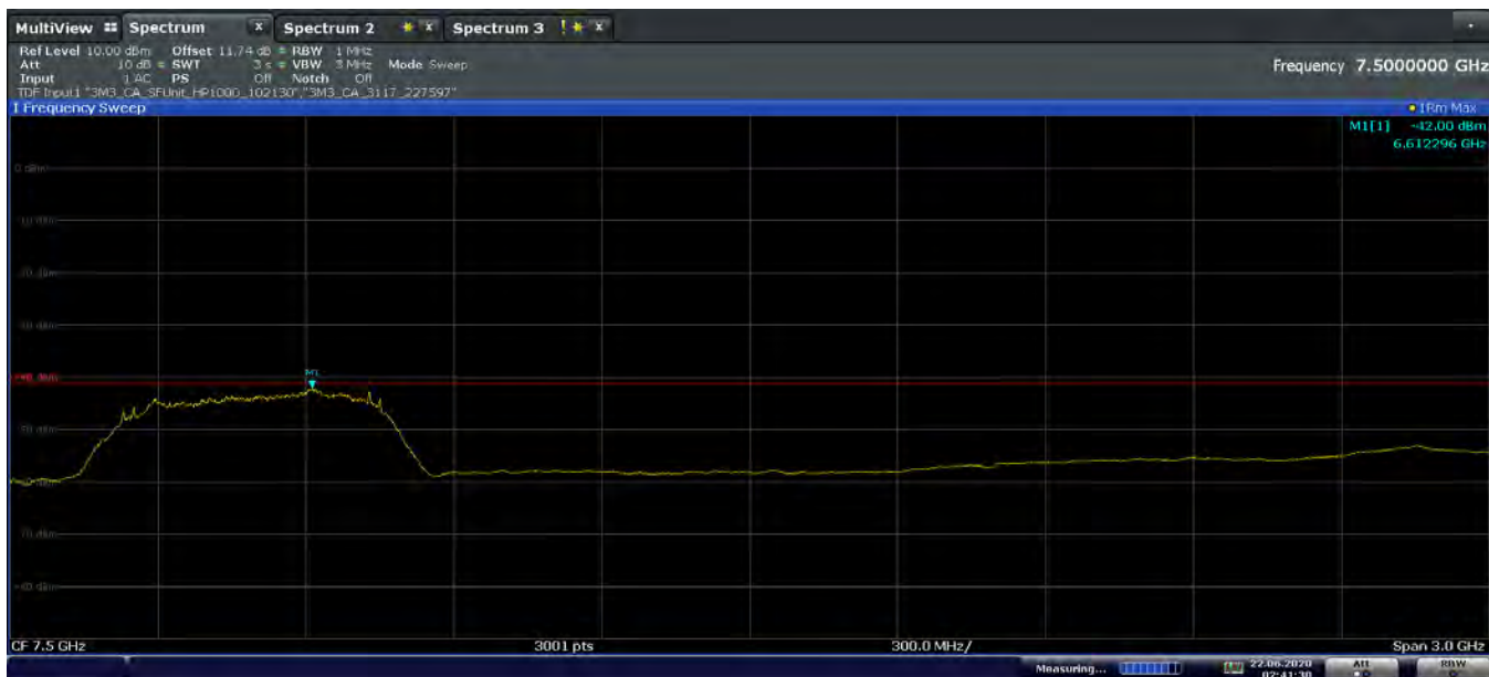
Plot 7-64. Average Radiated Power (Ch. 5, Config 1/Payload 45)
