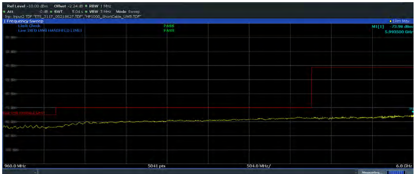
Plot 7-90. ISED Radiated Spurious Emission 960-6000MHz (Ch. 5, Config 3, Payload 125 Ant. Pol. V)
