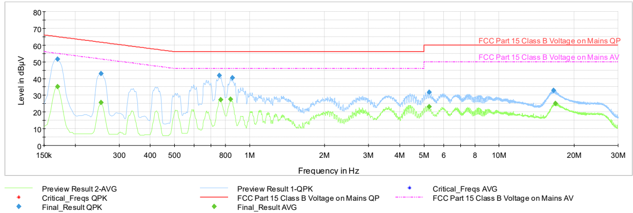
Plot 7-114. AC Line Conducted (Ch. 5, Config 3, Payload 125 N, with AC/DC Adapter)
