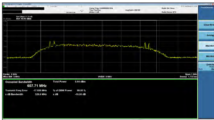
Plot 7-36. ISED Occupied Bandwidth (Ch. 9, Config 1/Payload 125)
