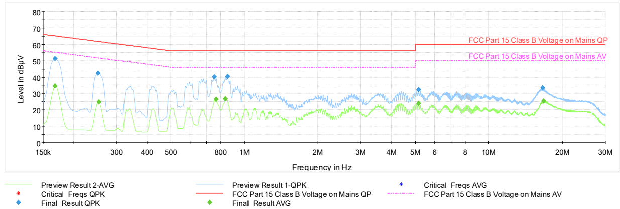
Plot 7-116. AC Line Conducted Plot (Ch. 9, Config 3, Payload 125 N, with AC/DC Adapter)
