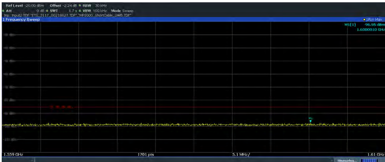
Plot 7-93. Radiated Spurious Emission 1559-1610MHz (Ch. 5, Config 3, Payload 125 Ant. Pol. H)
