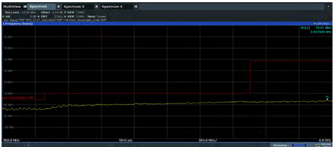
Plot 7-100. ISD Radiated Spurious Emission 960-6000MHz (Ch.9, Config 3, Payload 125 Ant. Pol. V)
