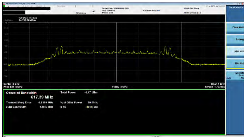
Plot 7-39. ISED Occupied Bandwidth (Ch. 9, Config 4/Payload 0)
