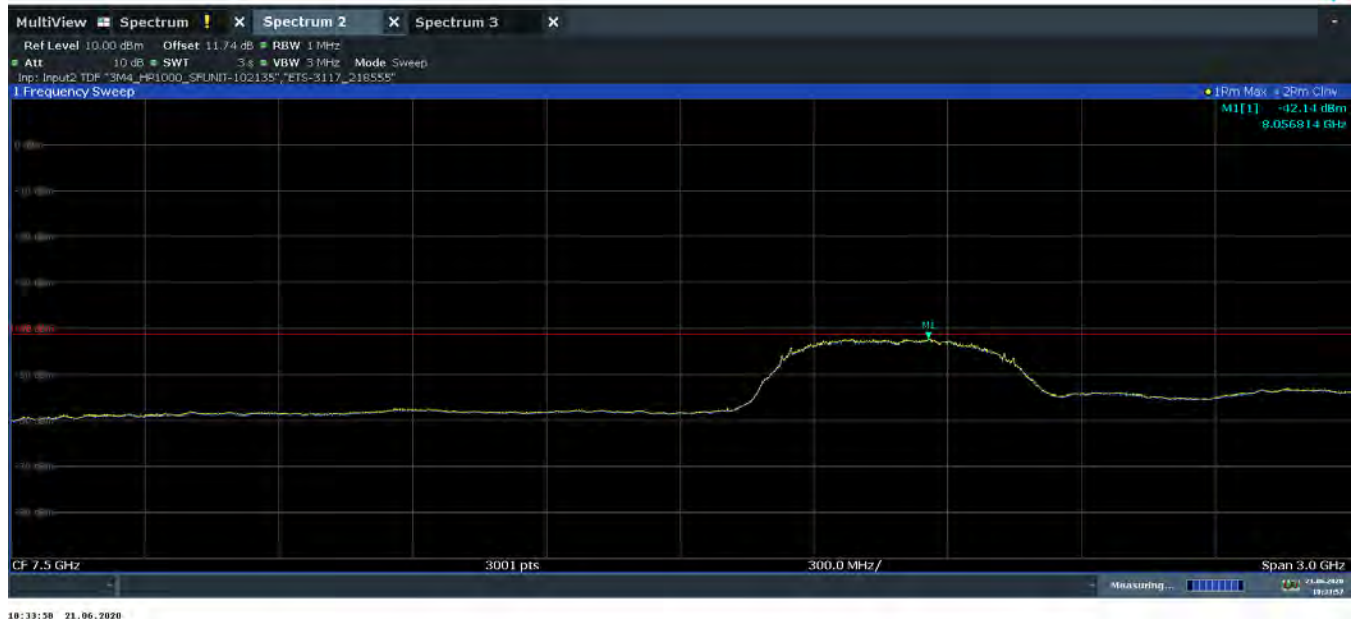
Plot 7-71. Average Radiated Power (Ch. 9, Config 0/Payload 25)
