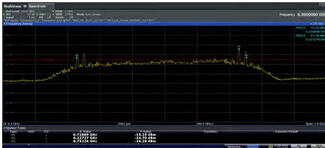
Plot 7-5. 10dBc Bandwidth (Ch. 5, Config 1/Payload 85)
