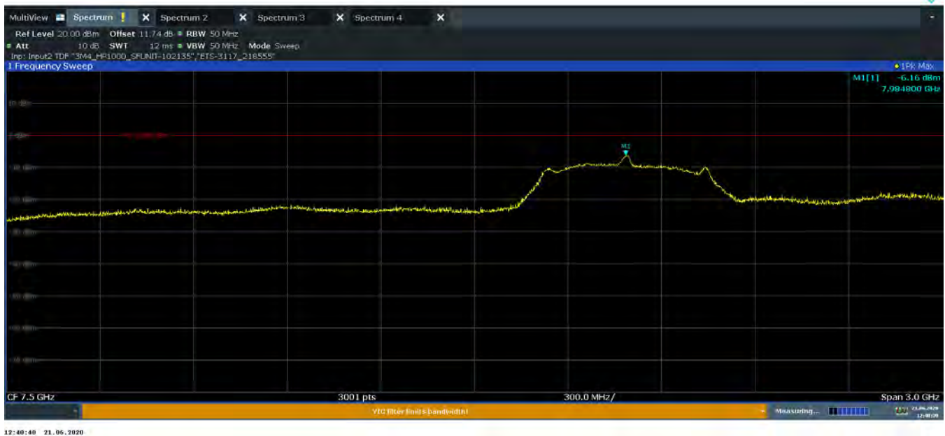
Plot 7-58. Peak Radiated Power (Ch. 9, Config 3/Payload 125)
