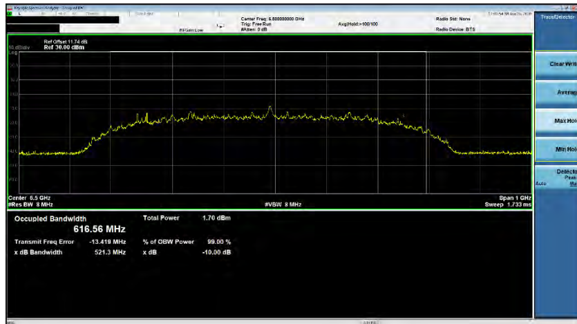
Plot 7-28. ISED Occupied Bandwidth (Ch. 5, Config 3/Payload 125)
