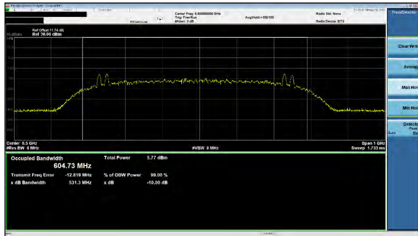
Plot 7-21. ISED Occupied Bandwidth (Ch. 5, Config 0/Payload 25)
