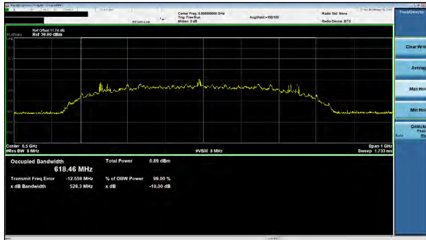
Plot 7-27. ISED Occupied Bandwidth (Ch. 5, Config 2/Payload 125)
