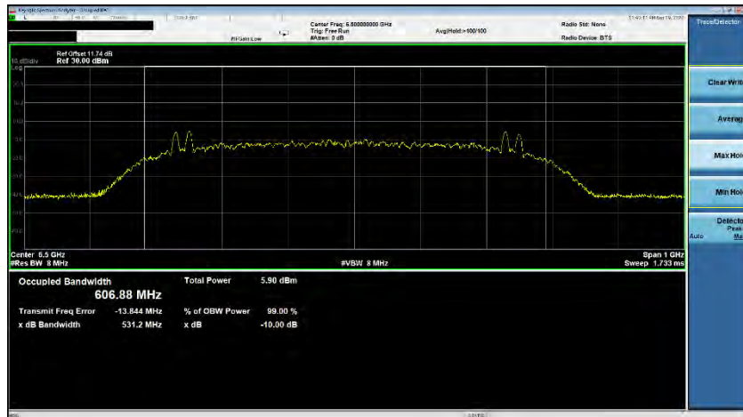
Plot 7-25. ISED Occupied Bandwidth (Ch. 5, Config 1/Payload 85)
