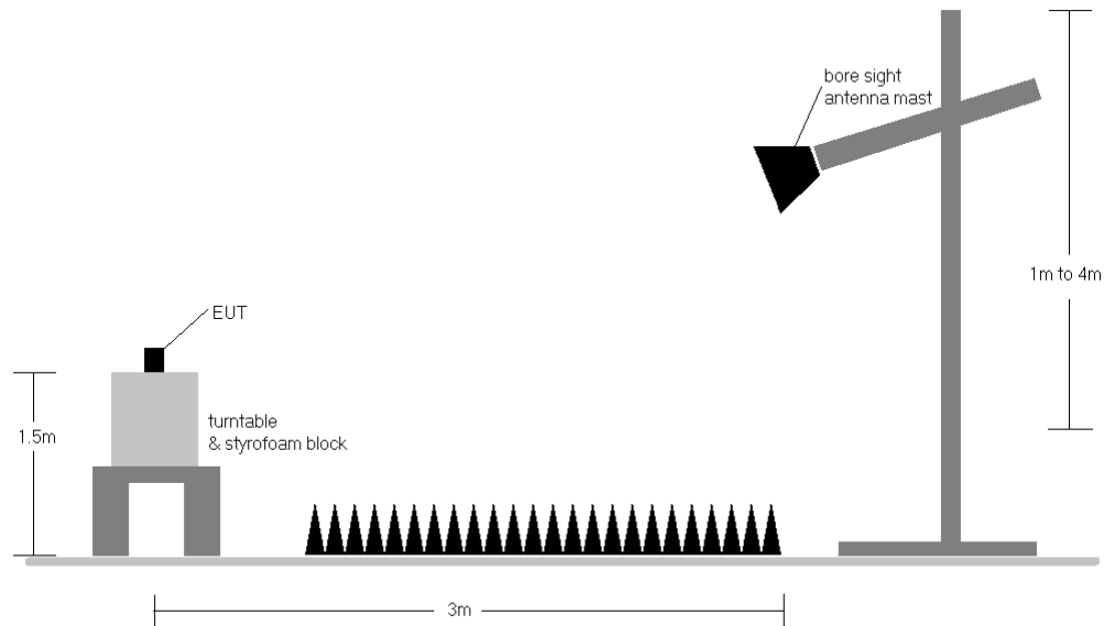
Figure 7-3. Test Setup
