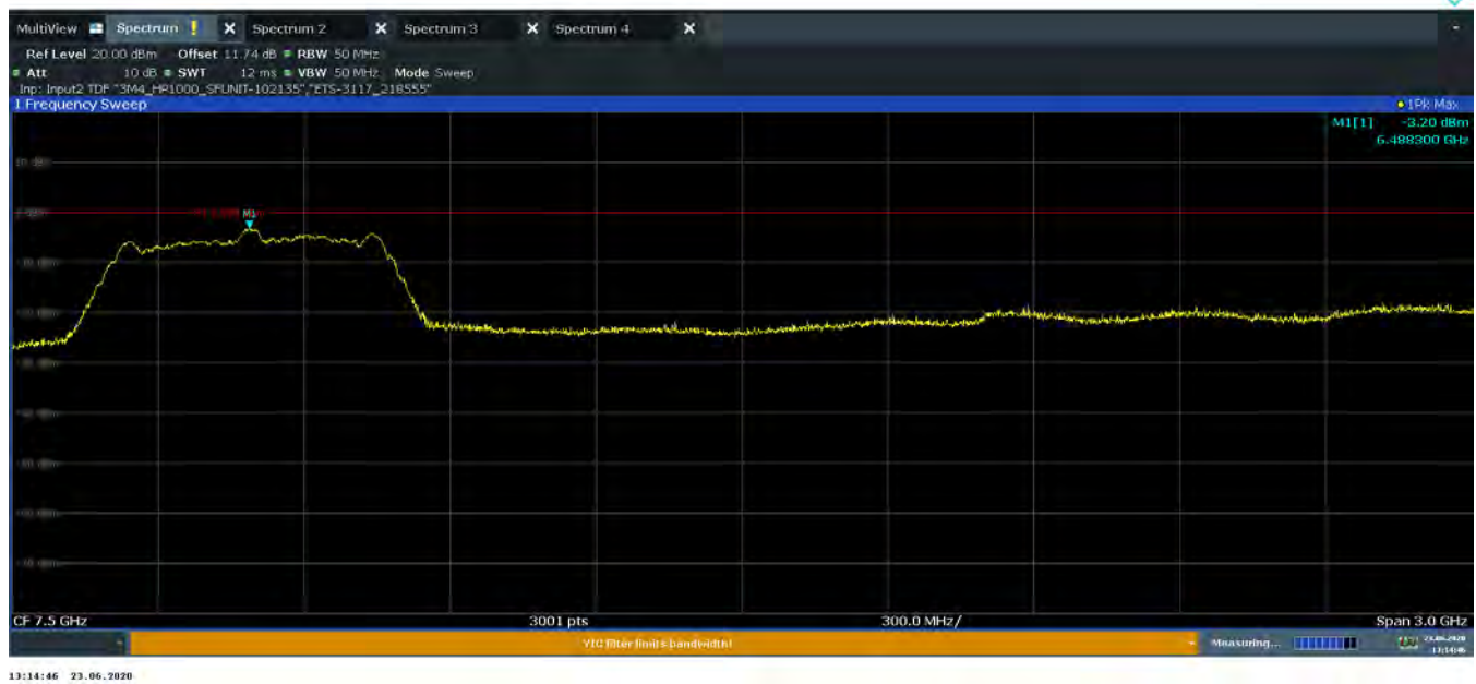
Plot 7-42. Peak Radiated Power (Ch. 5, Config 0/Payload 65)
