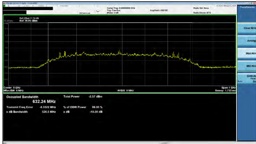
Plot 7-37. ISED Occupied Bandwidth (Ch. 9, Config 2/Payload 125)
