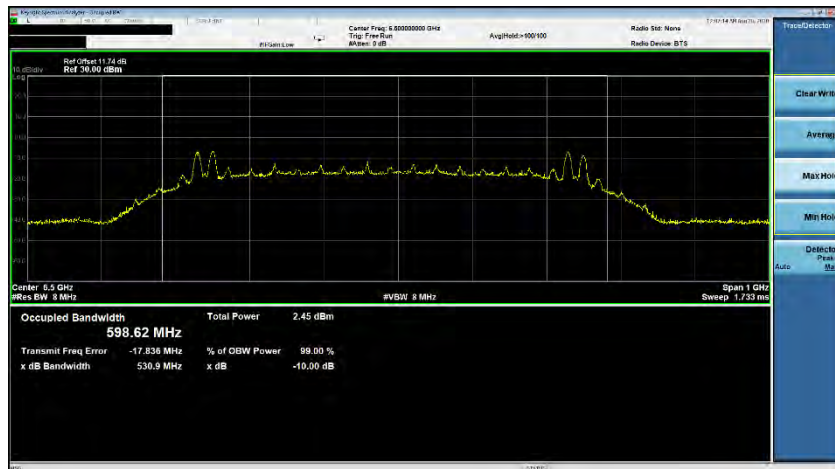
Plot 7-29. ISED Occupied Bandwidth (Ch. 5, Config 4/Payload 0)
