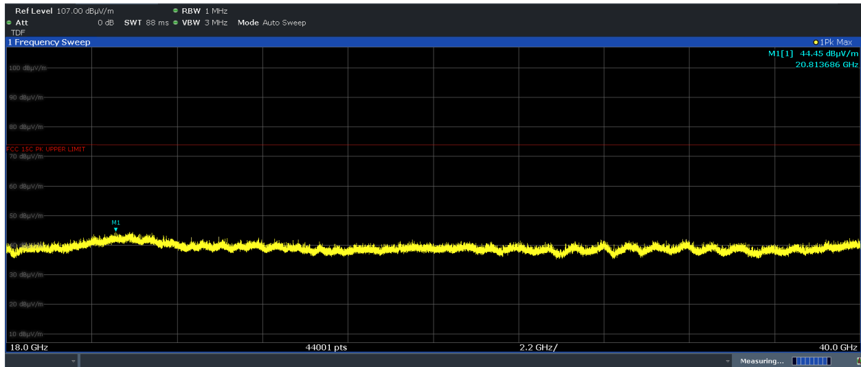
Plot 7-35. Radiated Spurious Emissions 18-40GHz (Simultaneous Transmission, Ant. Pol. H)
