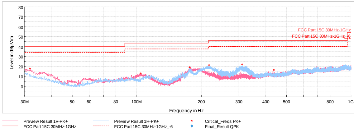
Plot 7-42. Radiated Spurious Emissions 30MHz-1GHz (Simultaneous Transmission, with WCP + AC/DC Adapter)
