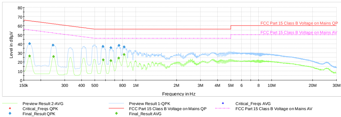
Plot 7-59. AC Line Conducted Emission with 802.11b Ch.1 (N, with WCP + AC/DC Adapter)
