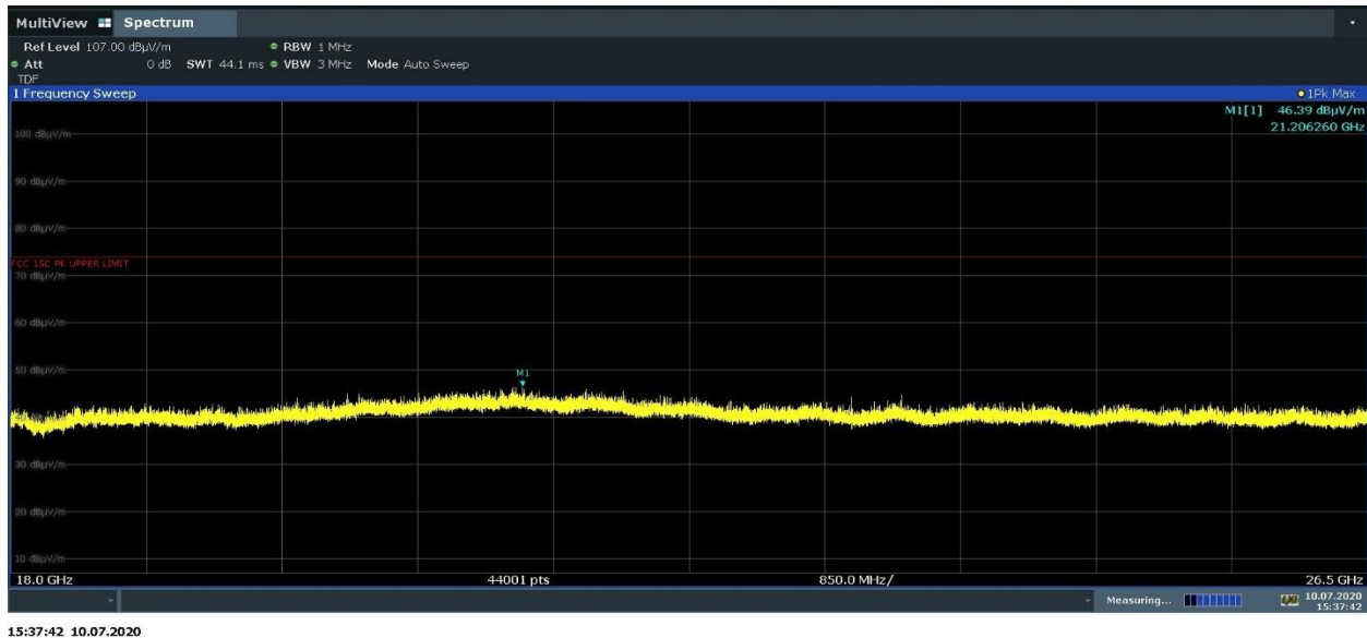
Plot 7-46. Radiated Spurious Emissions 18-26.5GHz (802.11b – Ch. 1, Ant. Pol. V)
