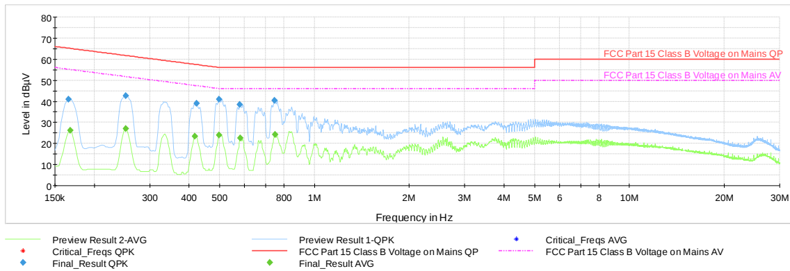
Plot 7-58. AC Line Conducted Emission with 802.11b Ch.1 (L1, with WCP + AC/DC Adapter)
