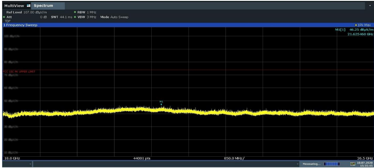
Plot 7-45. Radiated Spurious Emissions 18-26.5GHz (802.11b – Ch. 1, Ant. Pol. H)
