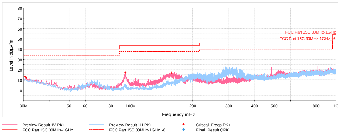
Plot 7-57. Radiated Spurious Emissions 30MHz-1GHz (802.11b – Ch.1, with WCP + laptop)
