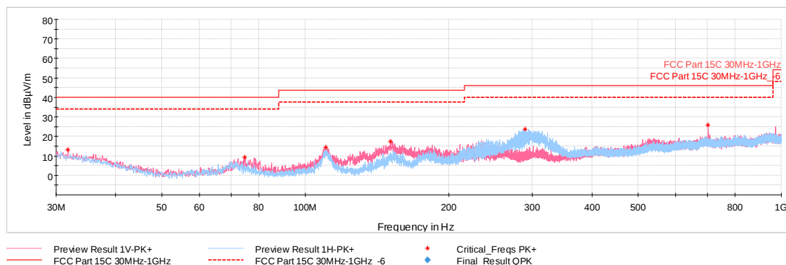
Plot 7-38. Radiated Spurious Emissions 30MHz-1GHz (4Mbps, ePA – Ch.38, with WCP + laptop)
