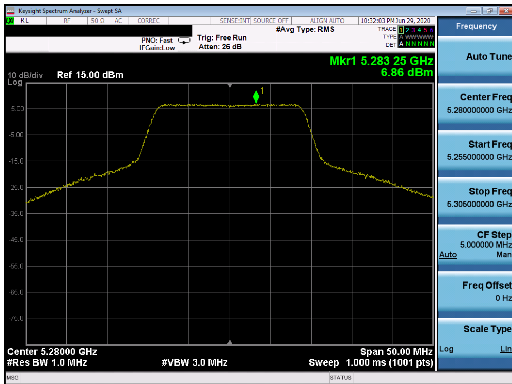
Plot 7-17. Power Spectral Density Plot (20MHz BW 802.11n (UNII Band 2A) – Ch. 56)
