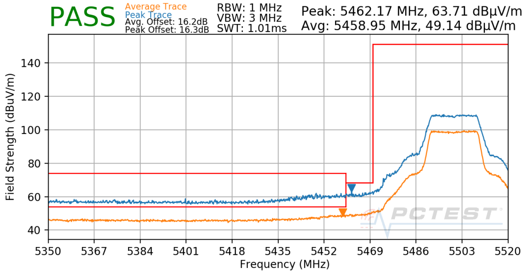
Plot 7-44. Radiated Lower Band Edge Plot (UNII Band 2C)
