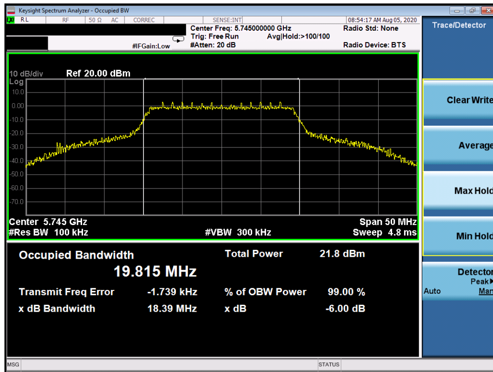
Plot 7-10. 6dB Bandwidth Plot (20MHz BW 802.11n (UNII Band 3) – Ch. 149)
