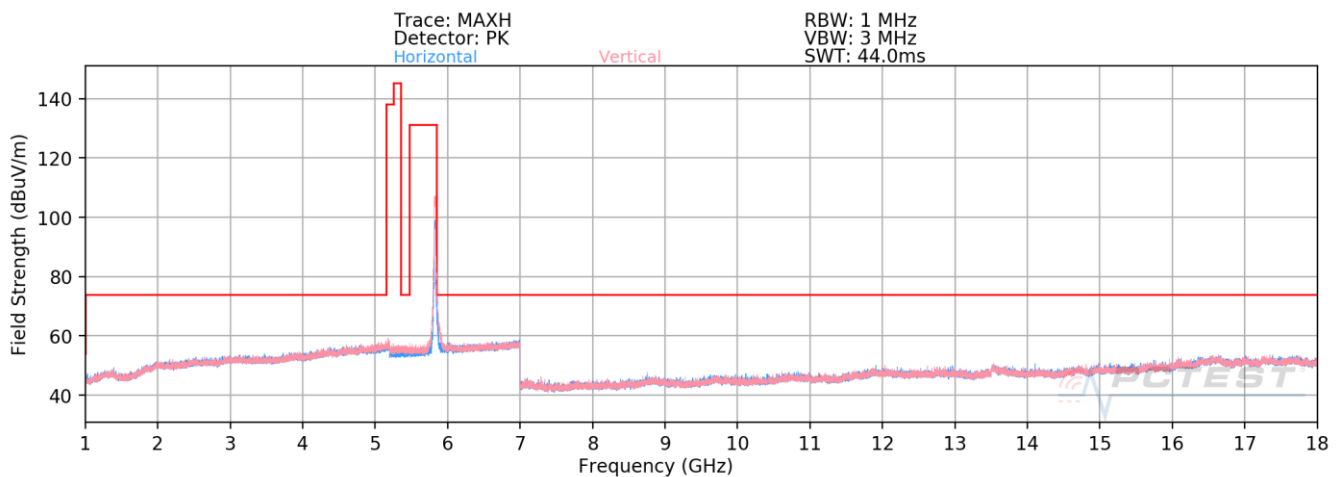
Plot 7-36. Radiated Spurious Emissions above 1GHz (802.11n – UNII 3 Ch. 165)
