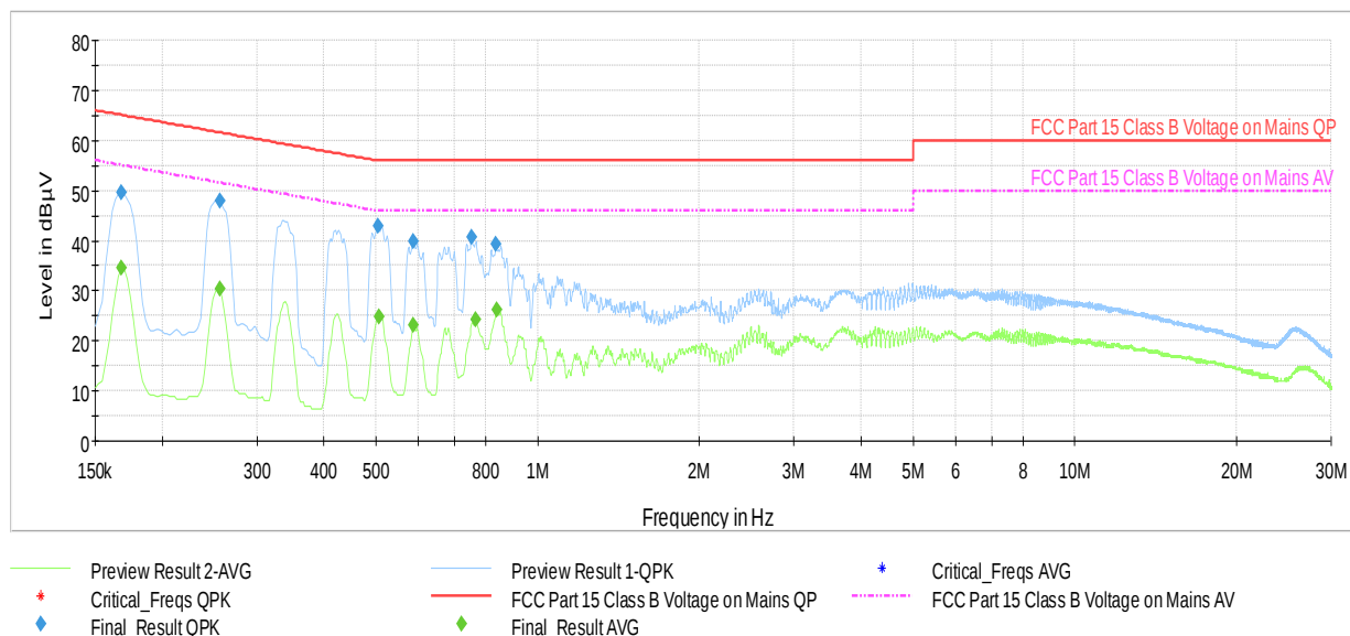
Plot 7-51. AC Line Conducted Plot with 802.11n UNII Band 2C – Ch.100 (L1) with WCP + AC/DC Adapter
