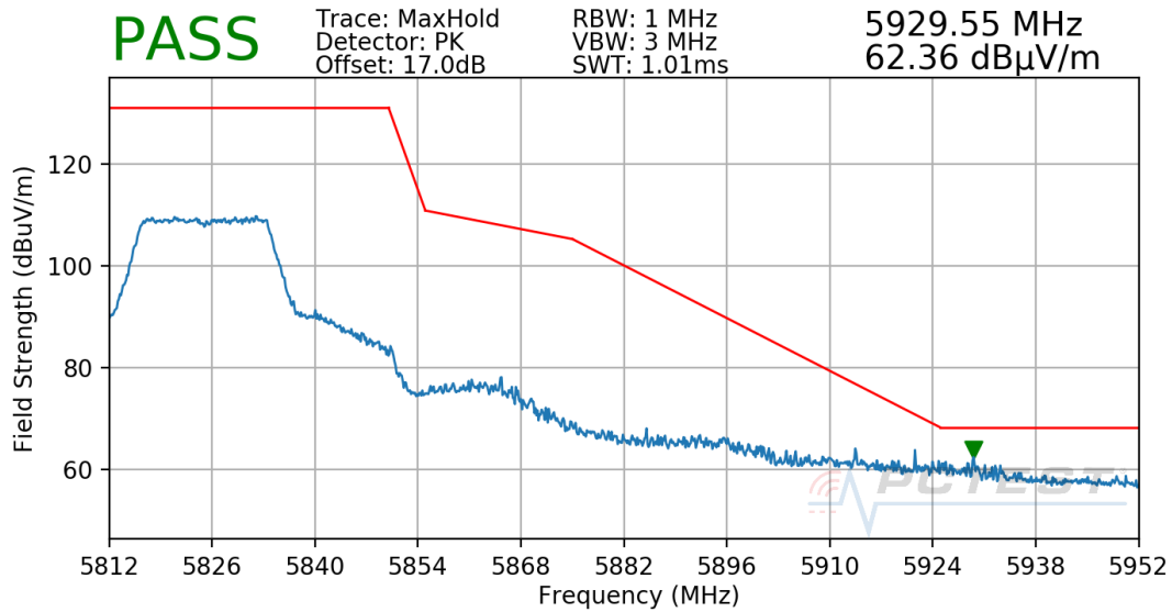
Plot 7-48. Radiated Upper Band Edge Plot (Peak – UNII Band 3)
