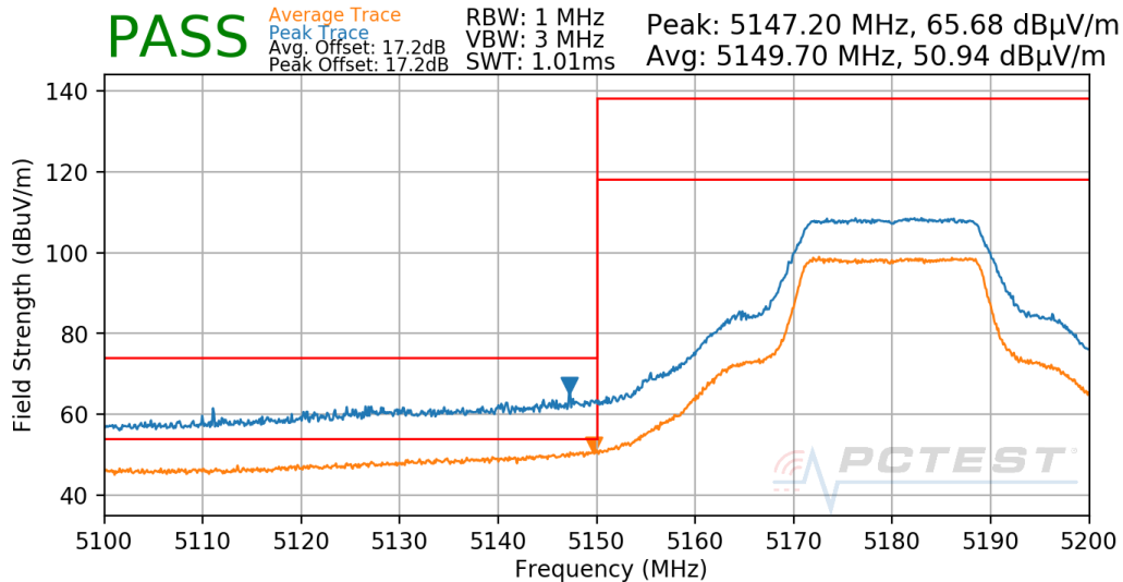
Plot 7-42. Radiated Lower Band Edge Plot (UNII Band 1)
