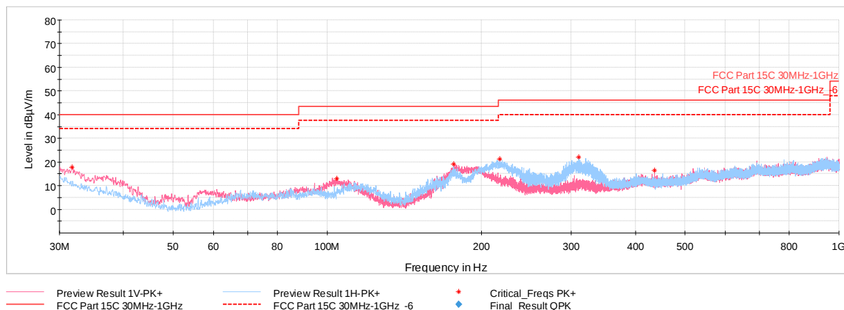
Plot 7-50. Radiated Spurious Emissions – Simultaneous Transmission below 1GHz with WCP + AC/DC Adapter
