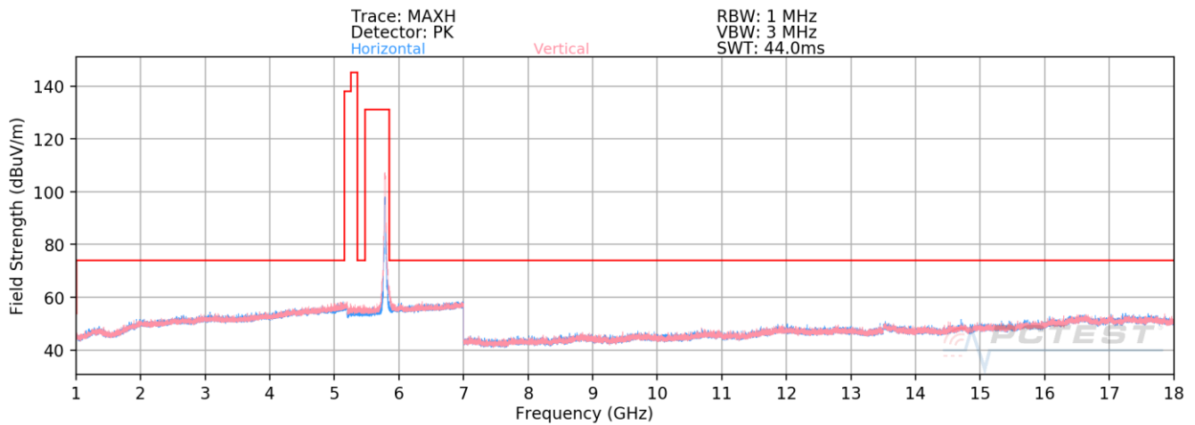
Plot 7-35. Radiated Spurious Emissions above 1GHz (802.11n – UNII 3 Ch. 157)
