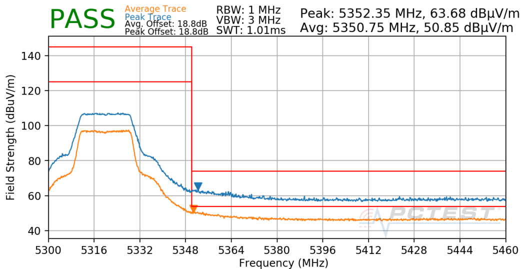
Plot 7-43. Radiated Upper Band Edge Plot (UNII Band 2A)
