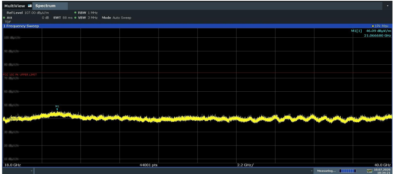
Plot 7-37. Radiated Spurious Emissions 18GHz - 40GHz – H Polarity (802.11n Ch 100)
