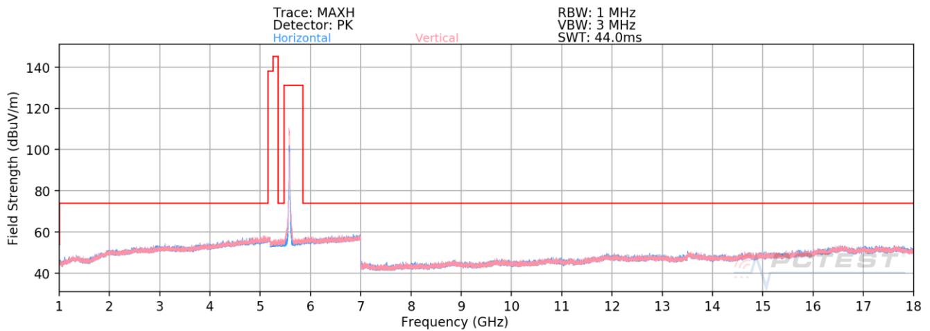
Plot 7-32. Radiated Spurious Emissions above 1GHz (802.11n – UNII 2C Ch. 116)
