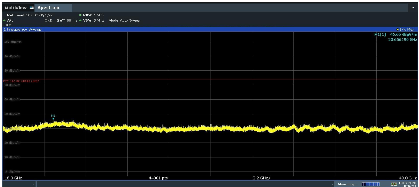
Plot 7-38. Radiated Spurious Emissions 18GHz - 40GHz – V Polarity (802.11n Ch 100)
