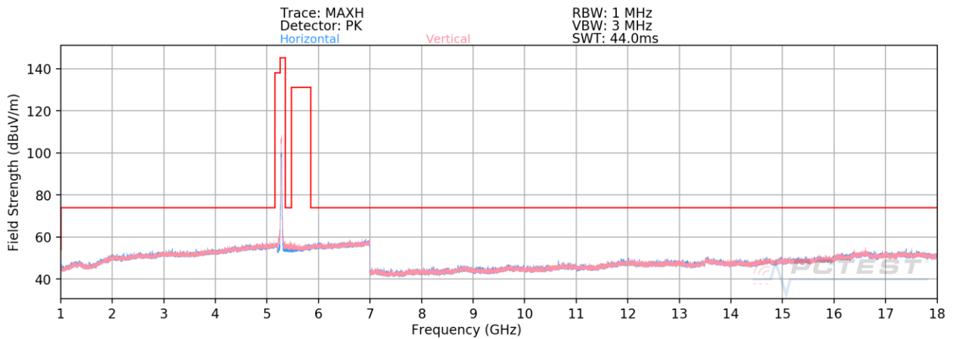
Plot 7-29. Radiated Spurious Emissions above 1GHz (802.11n – UNII 2A Ch. 56)
