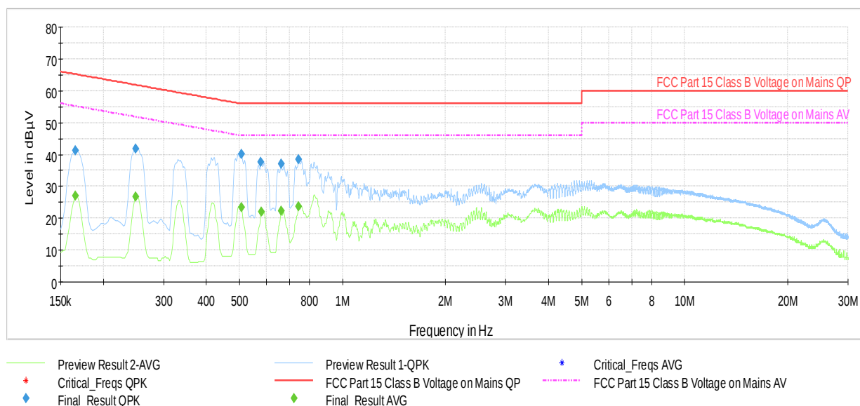
Plot 7-52. AC Line Conducted Plot with 802.11n UNII Band 2C – Ch.100 (N) with WCP + AC/DC Adapter
