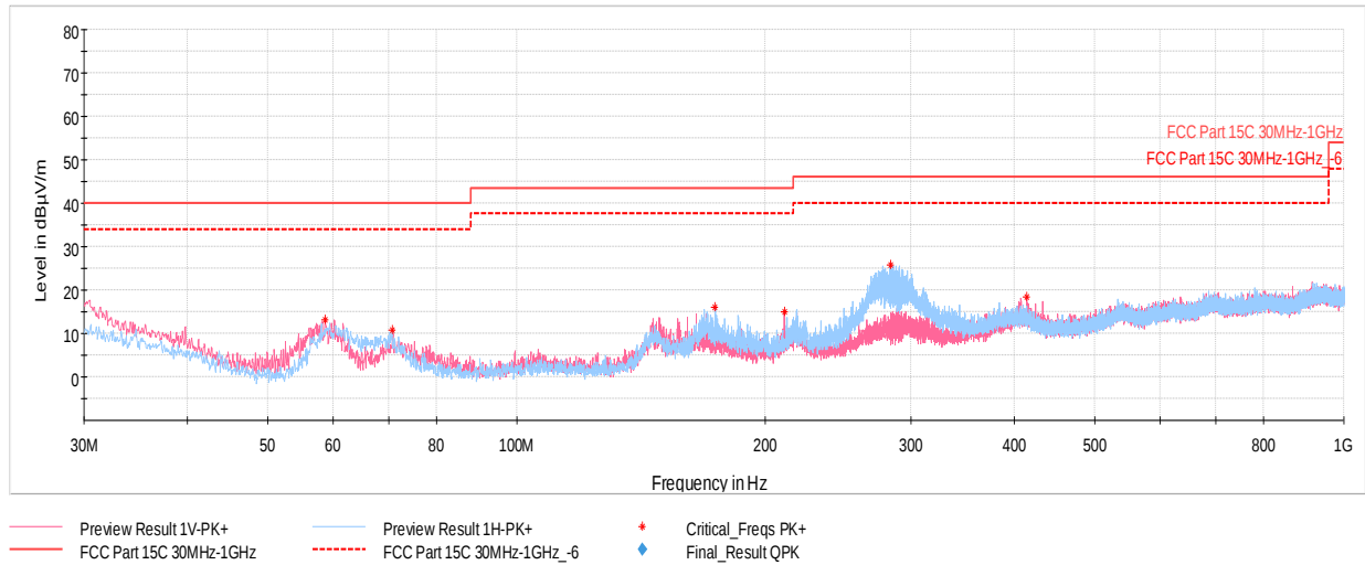
Plot 7-49. Radiated Spurious Emissions below 1GHz (802.11n – UNII 2C Ch. 100) with WCP + laptop
