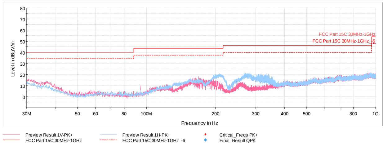
Plot 7-11. Radiated Spurious Emissions 30MHz – 1GHz (Reader 10% Ask 1 out of 256, with WCP + AC/DC Adapter)
