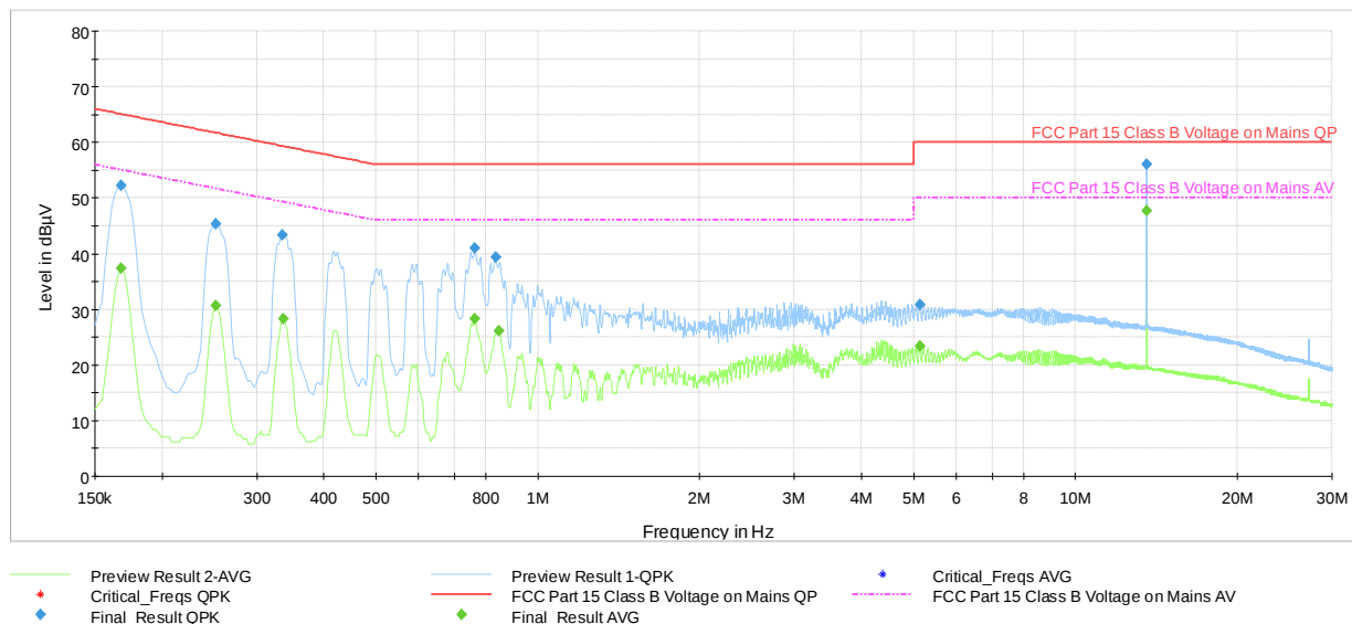
Plot 7-13. AC Line-Conducted Test Plot (N, with WCP + AC/DC Adapter)
