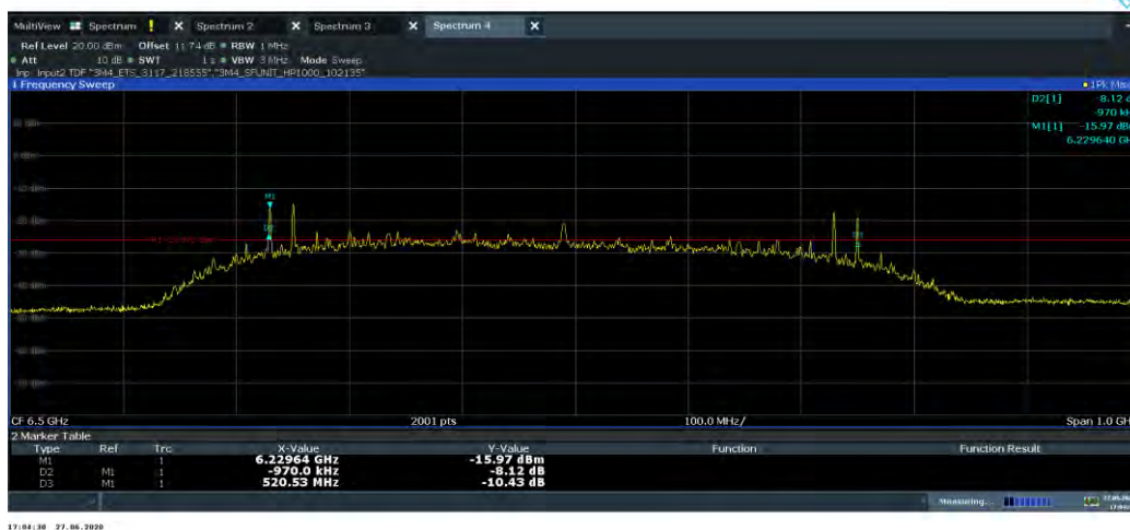
Plot 7-8. 10dBc Bandwidth (Ch. 5, Config 3/Payload 125)
