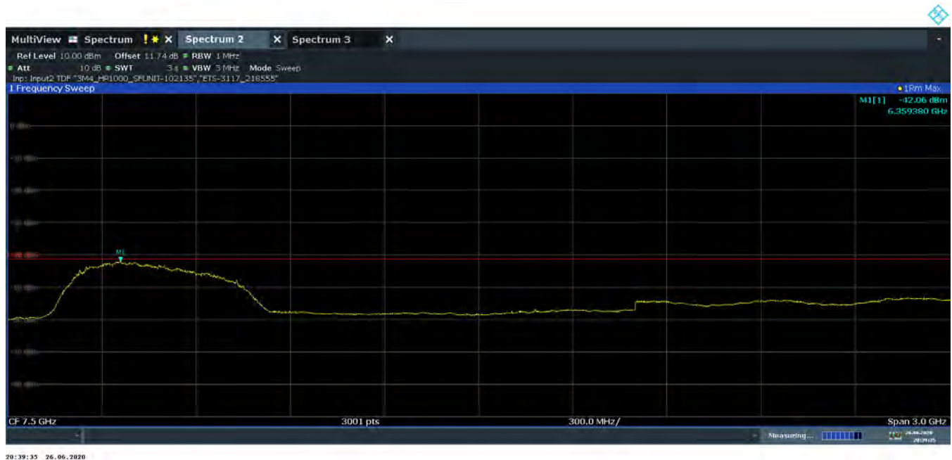
Plot 7-62. Average Radiated Power (Ch. 5, Config 0/Payload 65)
