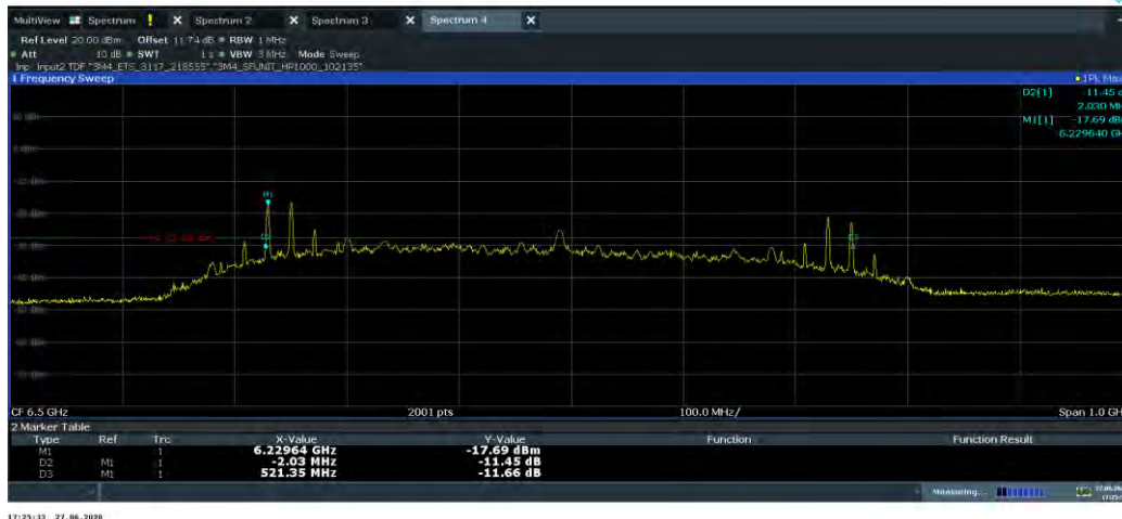
Plot 7-7. 10dBc Bandwidth (Ch. 5, Config 2/Payload 125)
