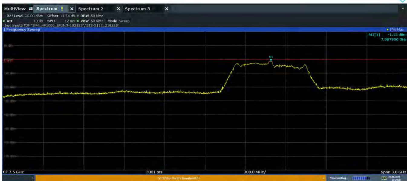
Plot 7-54. Peak Radiated Power (Ch. 9, Config 1/Payload 45)
