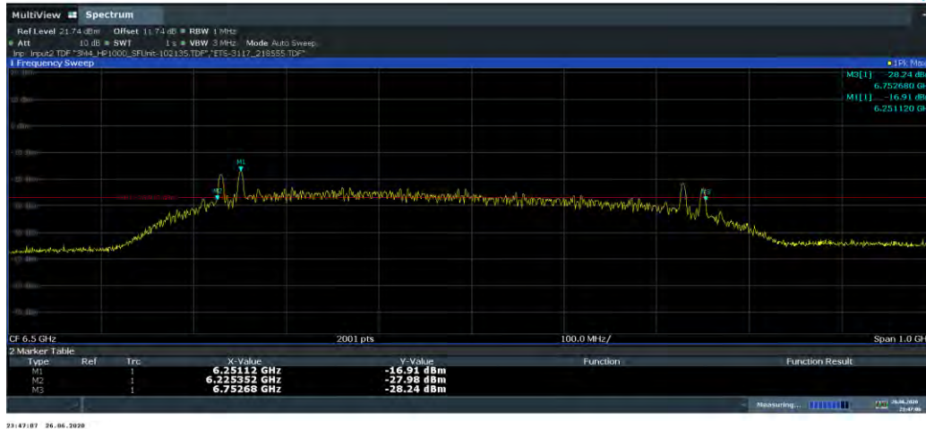
Plot 7-10. 10dBc Bandwidth (Ch. 5, Config 5/Payload 0)
