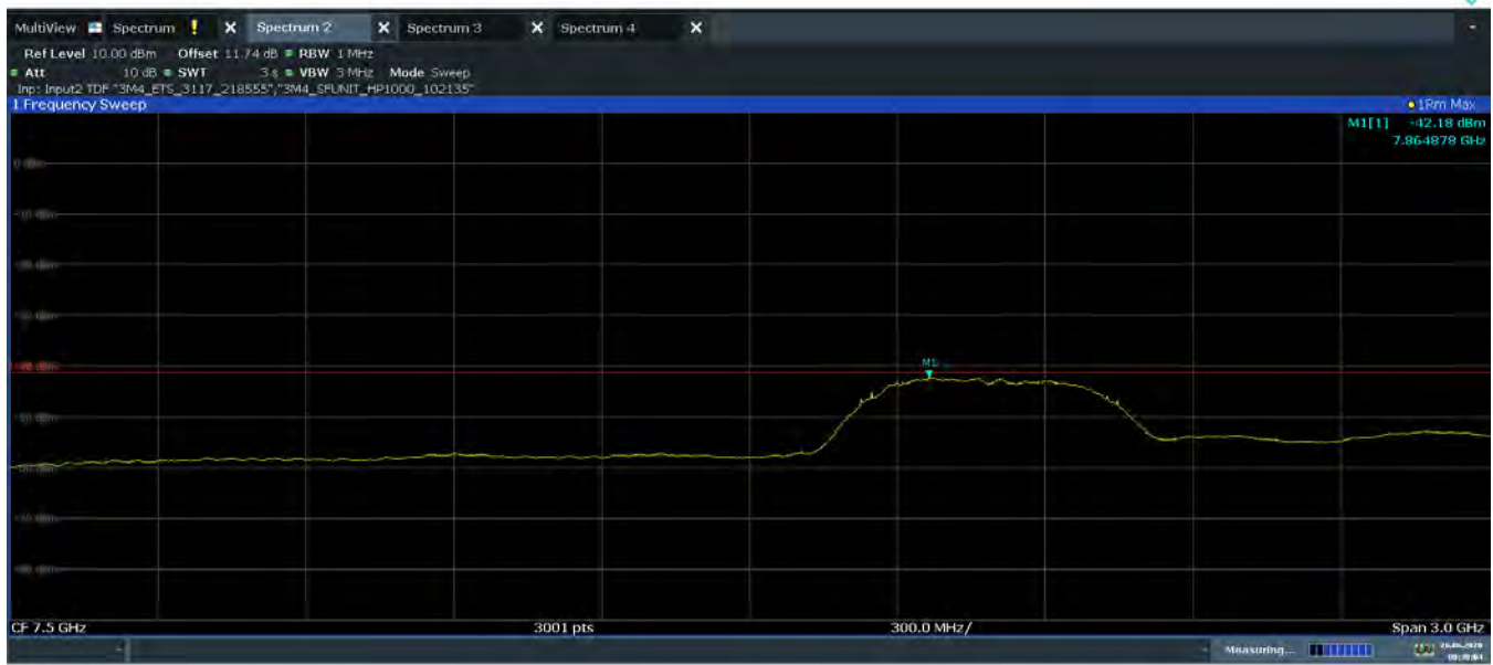
Plot 7-77. Average Radiated Power (Ch. 9, Config 2/Payload 125)
