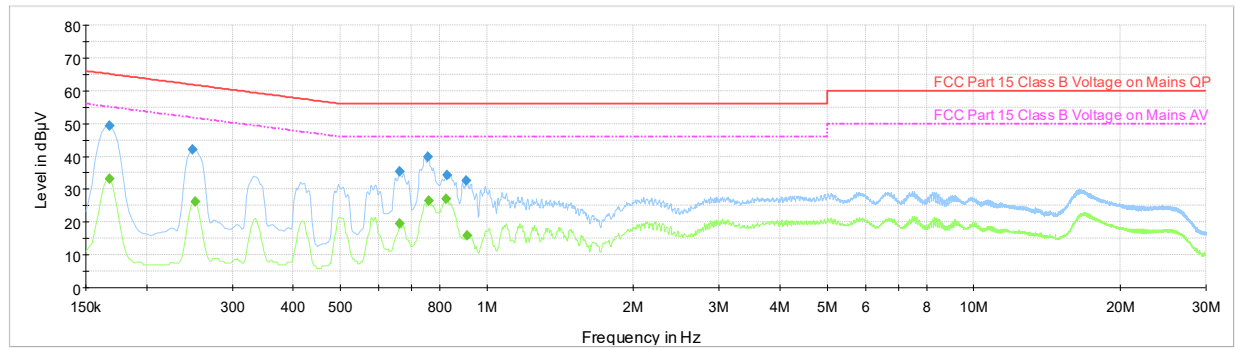
Plot 7-115. AC Line Conducted (Ch. 9, Config 3, Payload 125 L1, with AC/DC Adapter)
