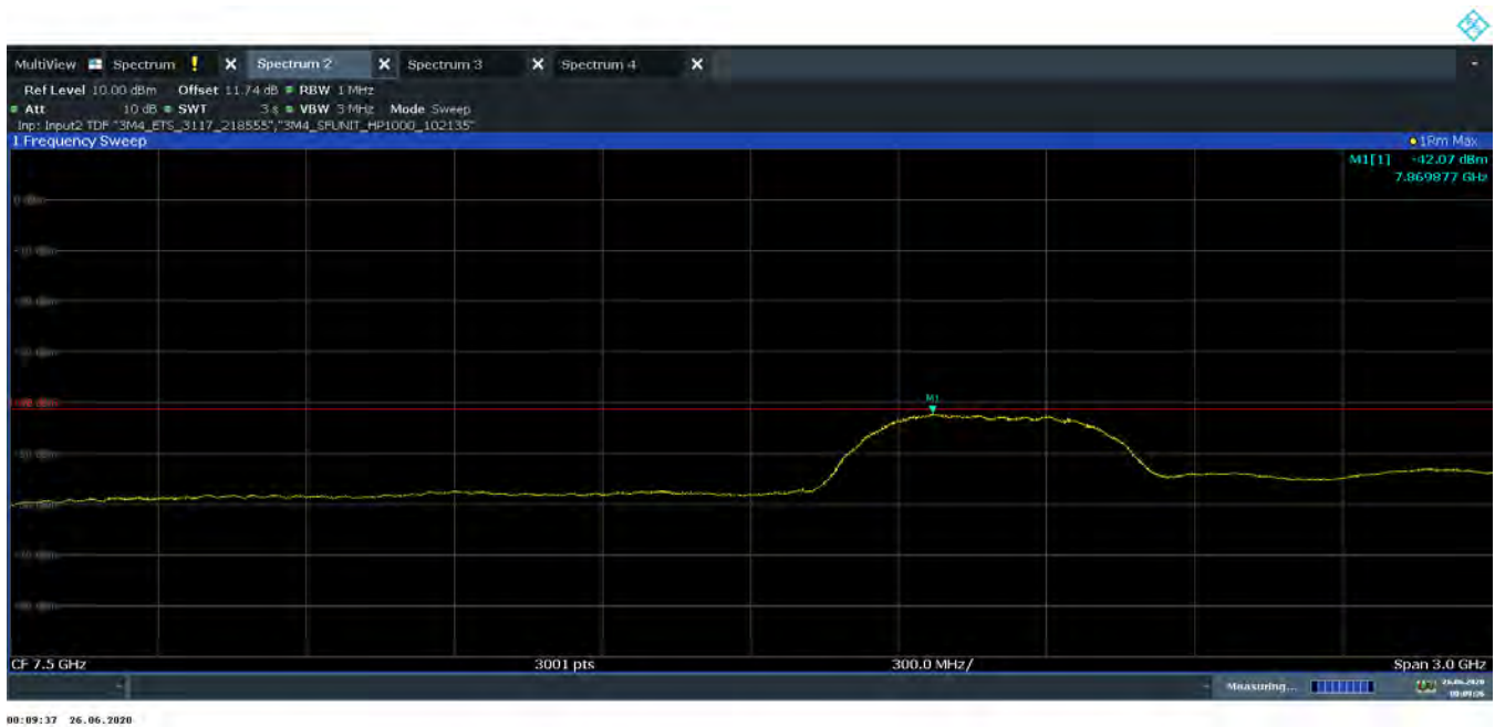
Plot 7-78. Average Radiated Power (Ch. 9, Config 3/Payload 125)
