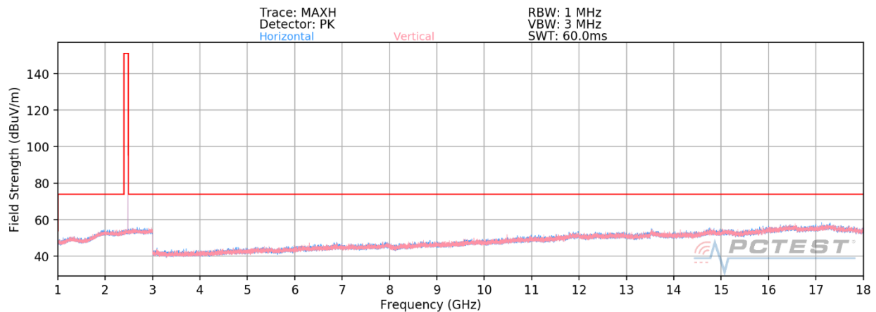
Plot 7-31. Radiated Spurious Emissions 1-18GHz (BT GFSK ePA – Ch. 78)
