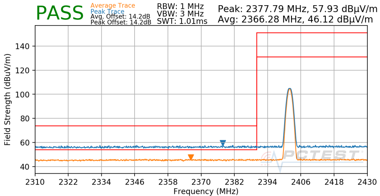
Plot 7-37. Radiated Restricted Lower Band Edge Measurement
