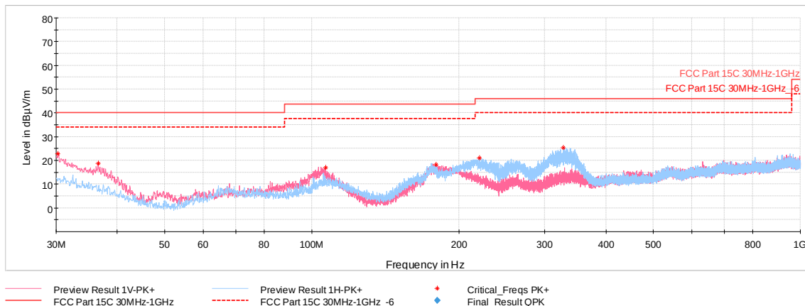
Plot 7-42. Radiated Spurious Emissions 30MHz-1GHz (Simultaneous Transmission, with WCP + AC/DC Adapter)
