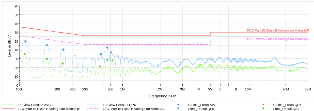
Plot 7-43. Line-Conducted Test Plot – GFSK ePA Ch.39 (L1, with WCP + AC/DC Adapter)
