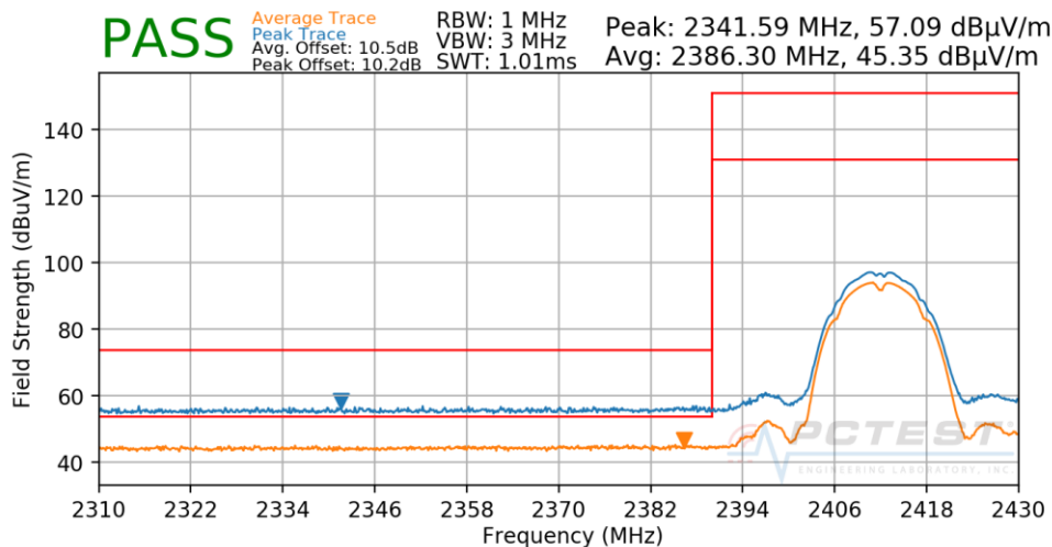
Plot 7-42. Radiated Restricted Lower Band Edge Measurement
