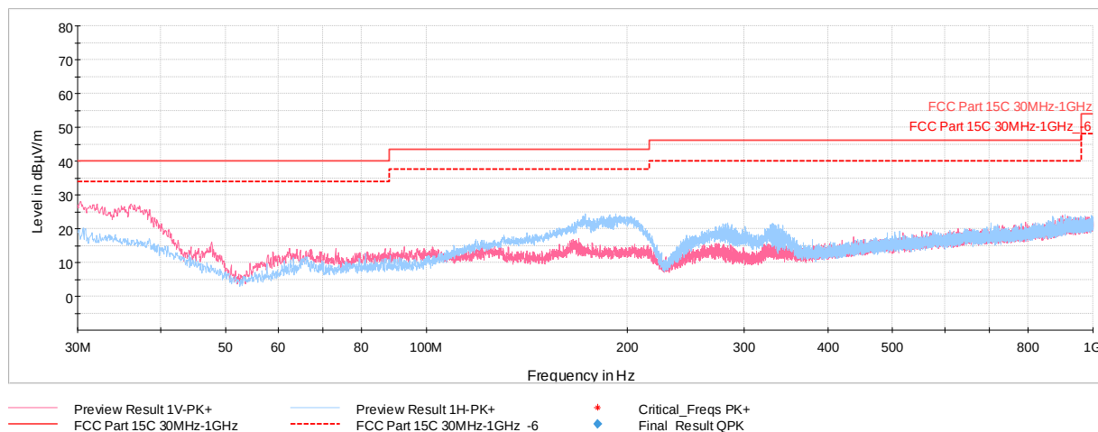
Plot 7-38. Radiated Spurious Plot below 1GHz (1Mbps, ePA, Ch.19 with WCP + AC/DC Adapter)
