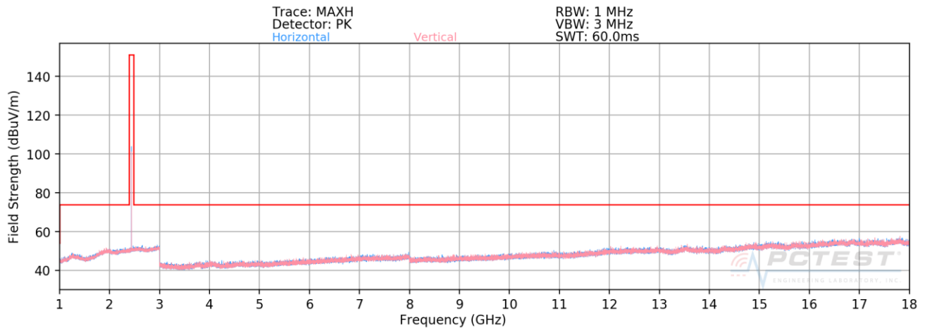
Plot 7-30. Radiated Spurious Plot Above 1GHz (1Mbps, ePA – Ch. 19)
