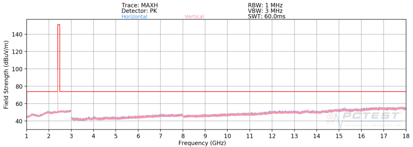
Plot 7-29. Radiated Spurious Plot Above 1GHz (1Mbps, ePA – Ch. 0)
