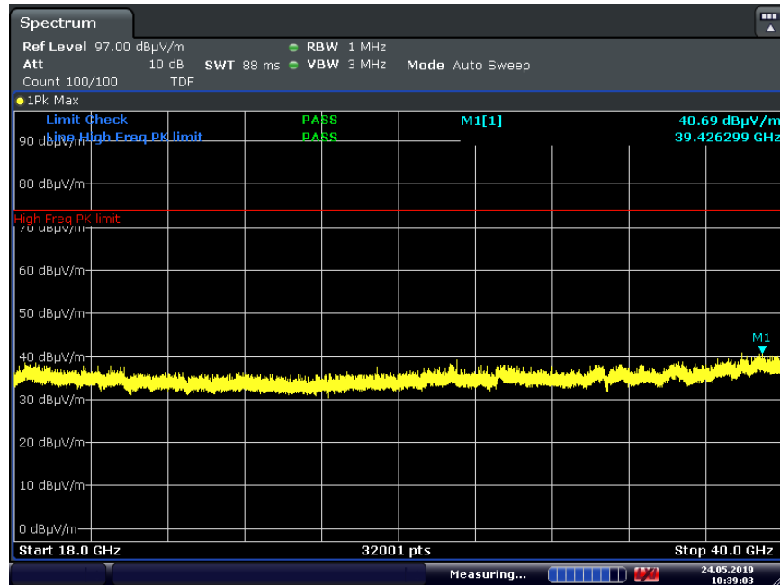
Plot 7-32. Radiated Spurious Plot Above 18GHz (1Mbps, ePA – Ch. 19, Ant. Pol. H)
