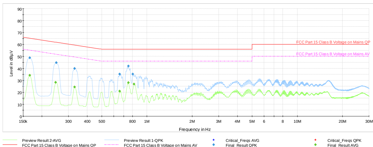
Plot 7-39. Line Conducted Plot with Bluetooth LE (L1 - 1Mbps, ePA, Ch.19 with WCP + AC/DC Adapter)
