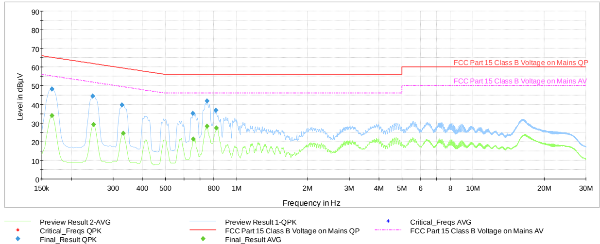
Plot 7-40. Line Conducted Plot with Bluetooth LE (N - 1Mbps, ePA, Ch.19 with WCP + AC/DC Adapter)
