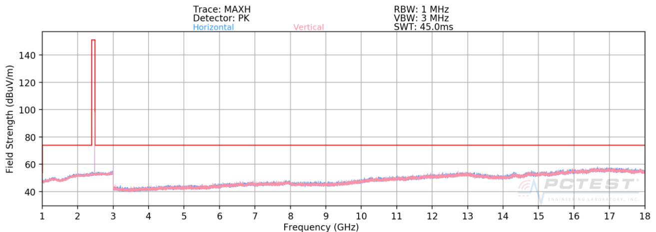
Plot 7-31. Radiated Spurious Plot Above 1GHz (1Mbps, ePA – Ch. 39)
