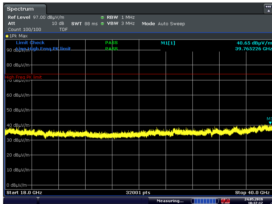
Plot 7-33. Radiated Spurious Plot Above 18GHz (1Mbps, ePA – Ch. 19, Ant. Pol. V)
