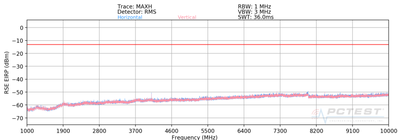
Plot 7-23. Radiated Spurious Plot Above 1GHz (Band 26)
