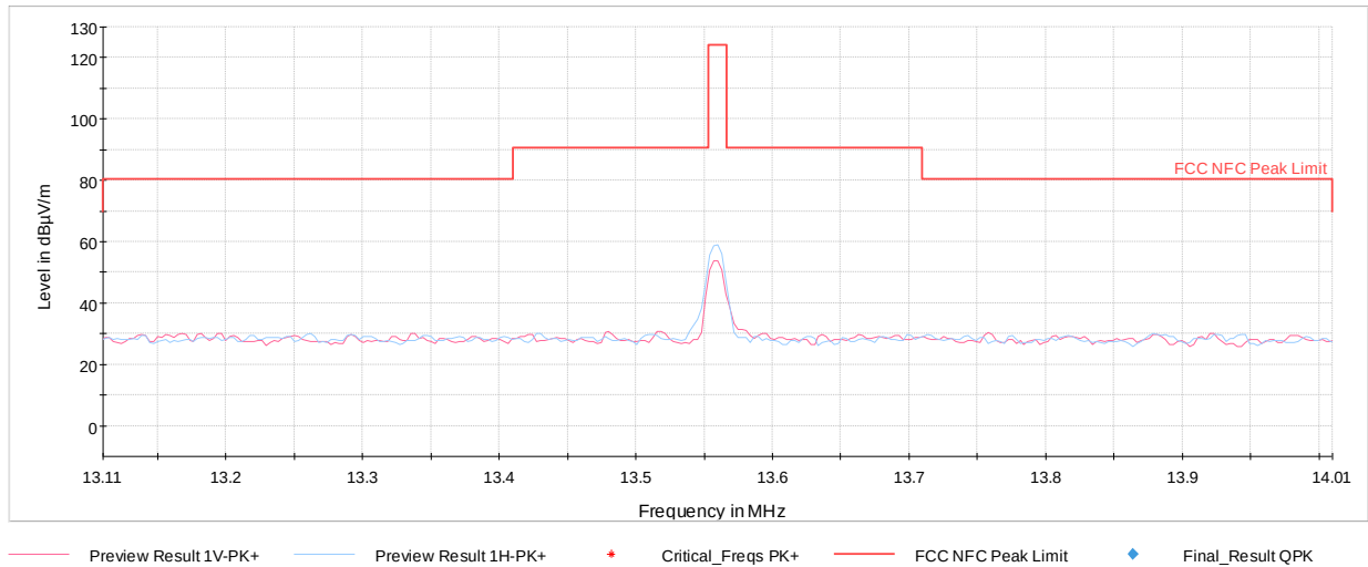
Plot 7-6. In Band Radiated Spurious Plot (CE A 848kbps)
