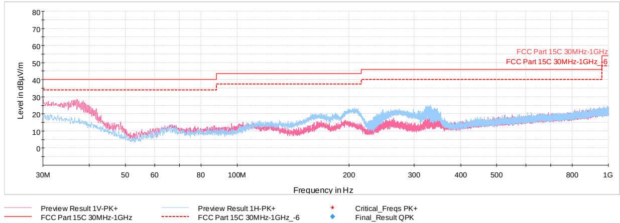
Plot 7-41. Radiated Spurious Plot below 1GHz GFSK ePA – Ch.39, with WCP + AC/DC Adapter
