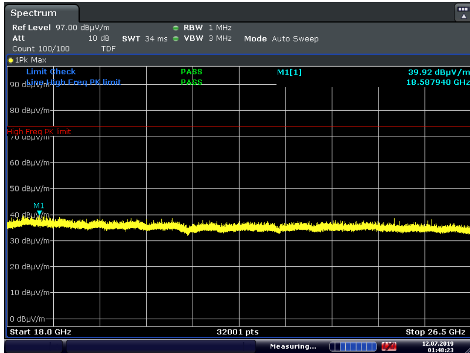
Plot 7-35. Radiated Spurious Plot above 18GHz (BT GFSK Mid Ch. + LTE Band 41 Mid Ch.- Ant. Pol. V)
