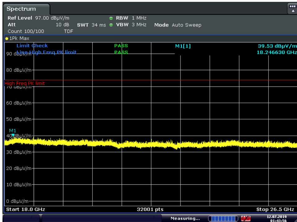
Plot 7-36. Radiated Spurious Plot above 18GHz (BT GFSK Mid Ch. + LTE Band 41 Mid Ch.- Ant. Pol. H)
