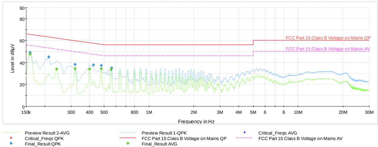
Plot 7-43. Line-Conducted Test Plot – Ch.39 (L1, with WCP + Laptop)
