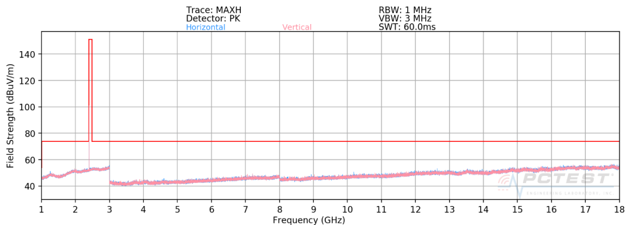
Plot 7-29. Radiated Spurious Plot above 1GHz (BT GFSK ePA – Ch. 0)
