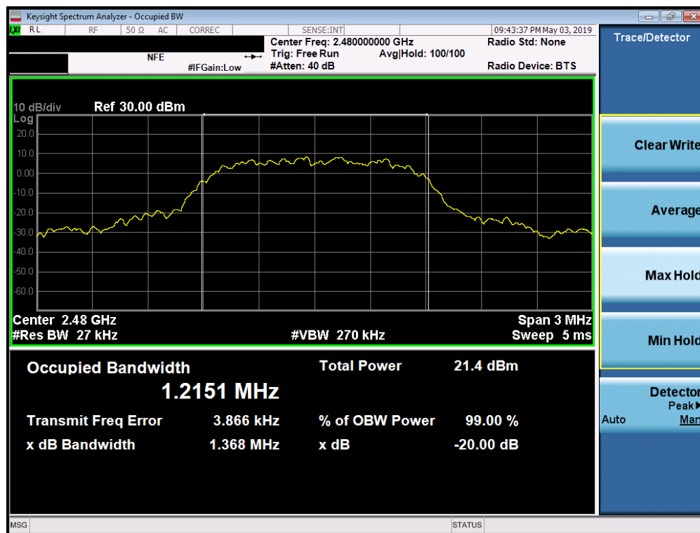
Plot 7-6. 20dB Bandwidth Plot (Bluetooth, 8DPSK, ePA – Ch. 78)
