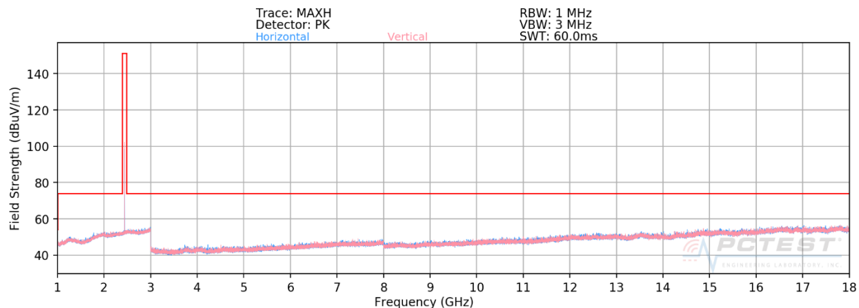
Plot 7-30. Radiated Spurious Plot above 1GHz (BT GFSK ePA – Ch. 39)
