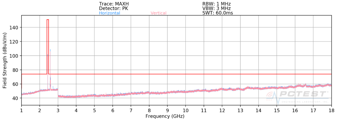
Plot 7-34. Radiated Spurious Plot above 1GHz (BT GFSK Mid Ch. + LTE Band 41 Mid Ch.)
