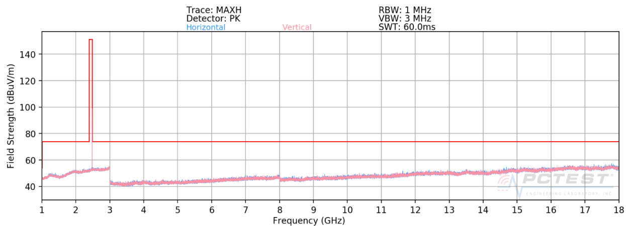
Plot 7-31. Radiated Spurious Plot above 1GHz (BT GFSK ePA – Ch. 78)
