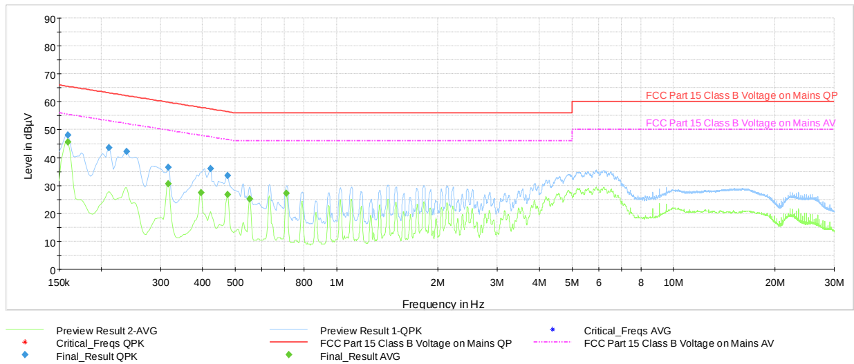
Plot 7-44 Line-Conducted Test Data – Ch.39 (N, with WCP + Laptop)
