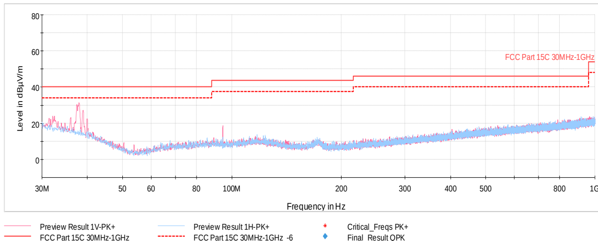
Plot 7-42. Radiated Spurious Plot below 1GHz with WCP + AC/DC Adapter
