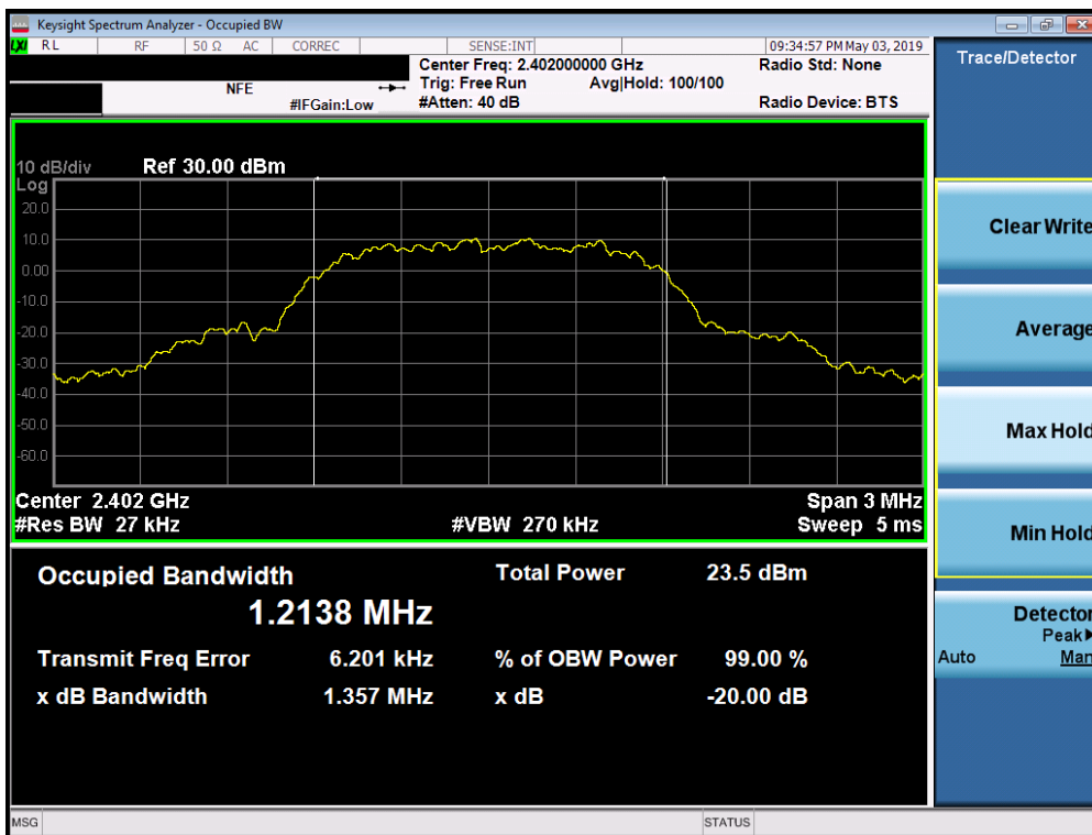
Plot 7-4. 20dB Bandwidth Plot (Bluetooth, 8DPSK, ePA – Ch. 0)
