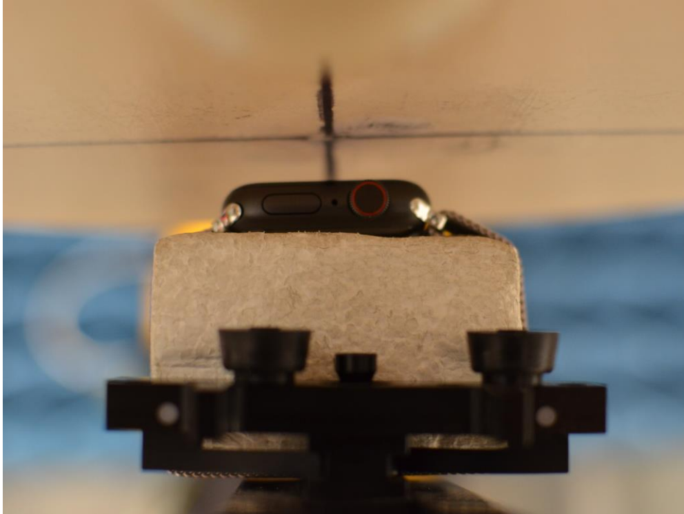
SAR Test Setup Photo 3: Aluminum with Metal Loop Wristband, Front side at 1.0 cm
