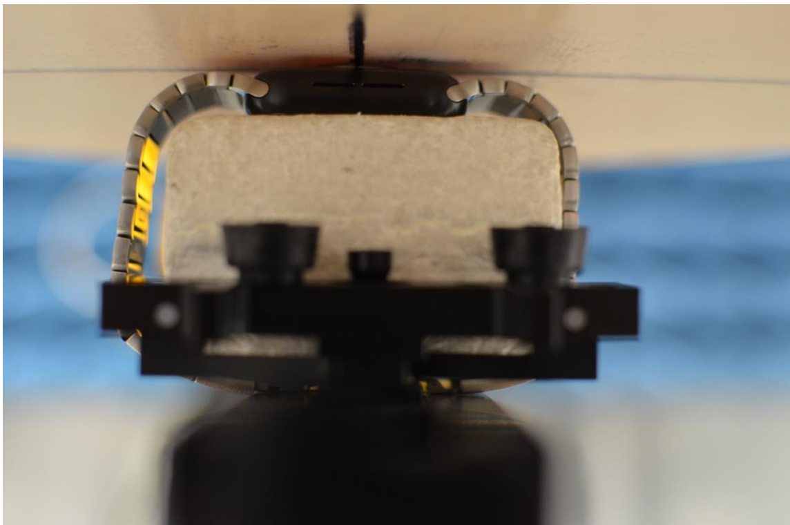
SAR Test Setup Photo 20: Titanium with Metal Links Wristband, Back side at 0.0 cm
