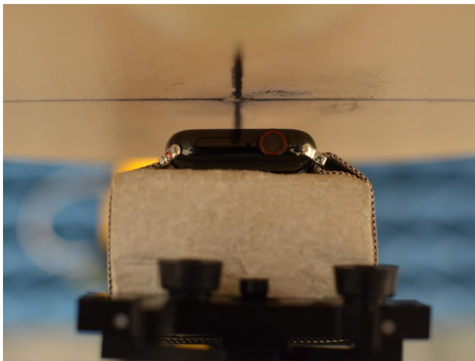
SAR Test Setup Photo 6: Stainless Steel with Metal Loop Wristband, Front side at 1.0 cm
