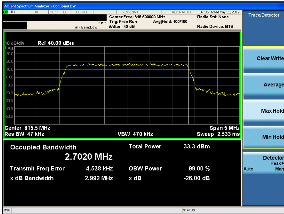
Plot 7-3. Occupied Bandwidth Plot (LTE Band 26, 3MHz QPSK – RB Size 15– Low Channel)
