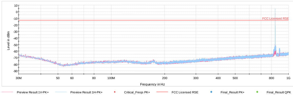
Plot 7-22. Radiated Spurious Plot - Below 1GHz (LTE Band 26 High channel, with WCP + AC/DC Adapter)
