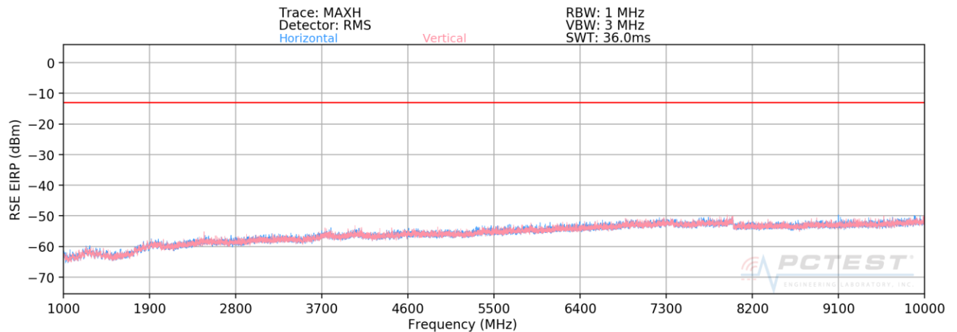
Plot 7-24. Radiated Spurious Plot Above 1GHz (Band 26)
