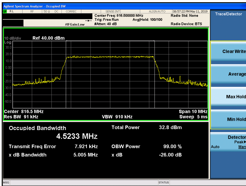
Plot 7-6. Occupied Bandwidth Plot (LTE Band 26, 5MHz 16-QAM – RB Size 25– Low Channel)
