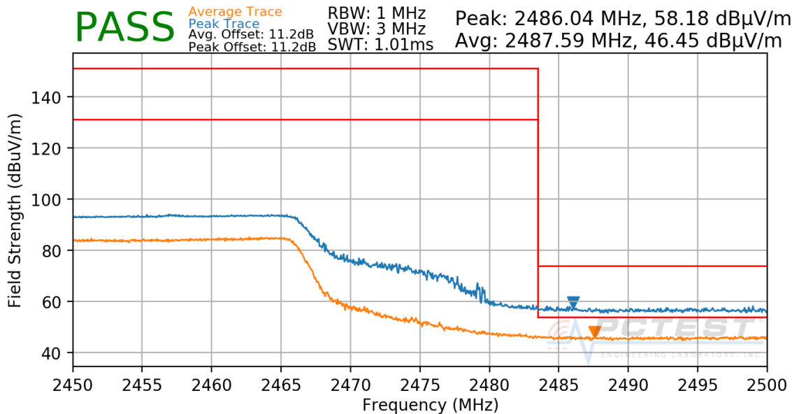
Plot 7-47. Radiated Restricted Upper Band Edge Measurement
