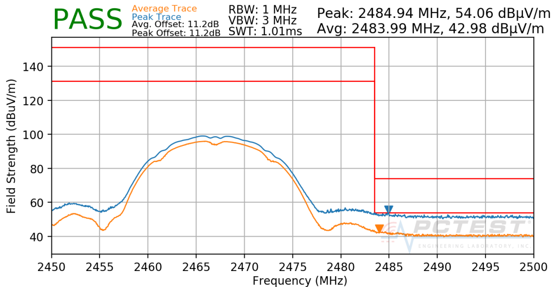
Plot 7-43. Radiated Restricted Upper Band Edge Measurement
