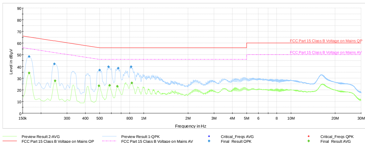
Plot 7-53. Line Conducted Plot with 802.11b Ch.6 (N, with WCP + AC/DC Adapter)
