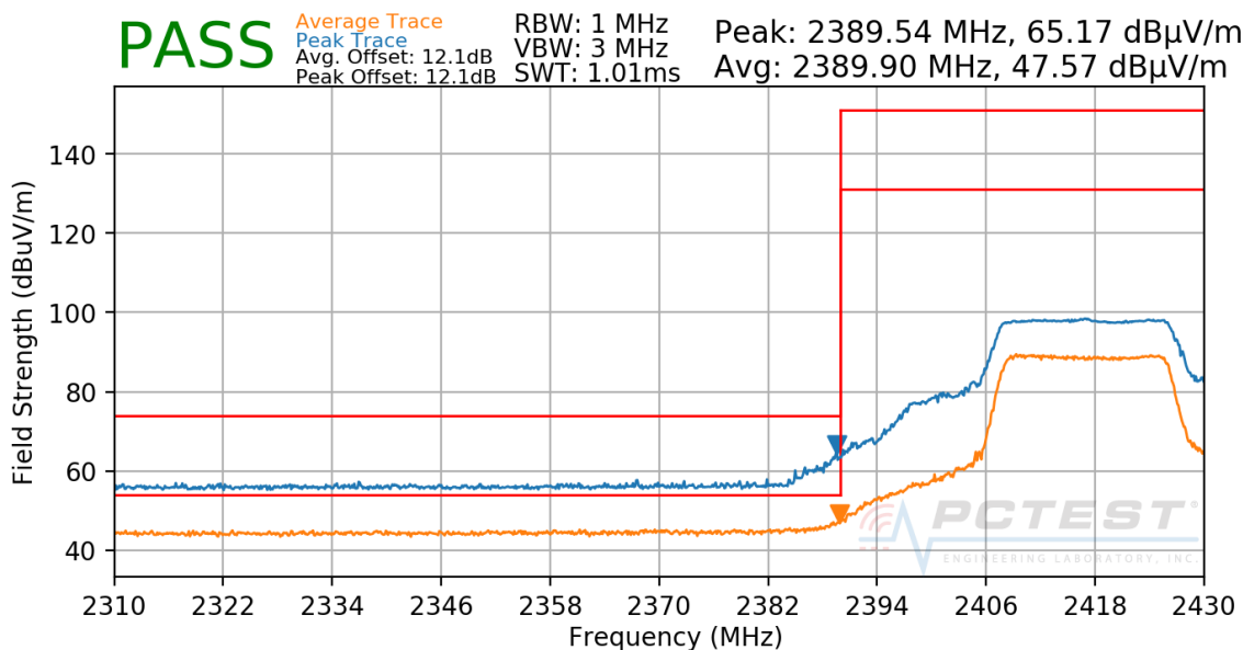
Plot 7-46. Radiated Restricted Lower Band Edge Measurement
