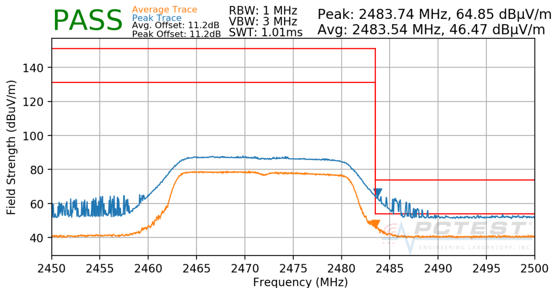
Plot 7-50. Radiated Restricted Upper Band Edge Measurement
