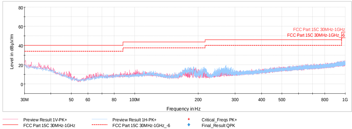
Plot 7-51. Radiated Spurious Plot Below 1GHz (802.11b – Ch.6, with WCP + AC/DC Adapter)
