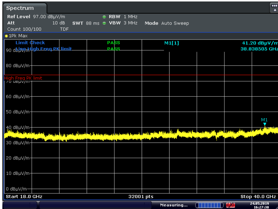
Plot 7-41. Radiated Spurious Plot above 18GHz (802.11b – Ch. 6, Ant. Pol. V)
