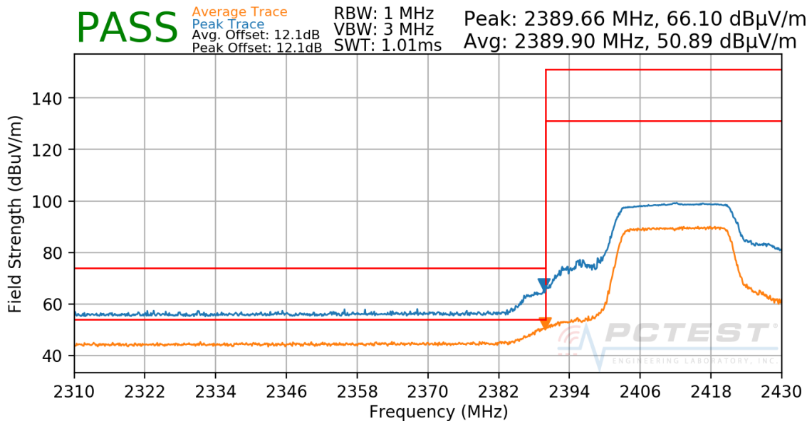
Plot 7-45. Radiated Restricted Lower Band Edge Measurement
