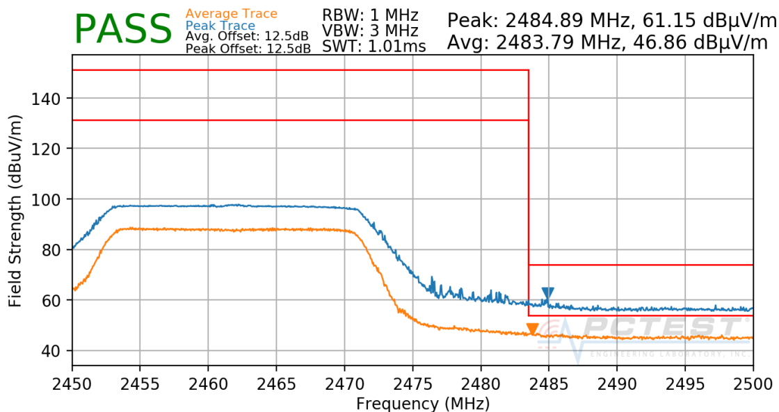
Plot 7-48. Radiated Restricted Upper Band Edge Measurement
