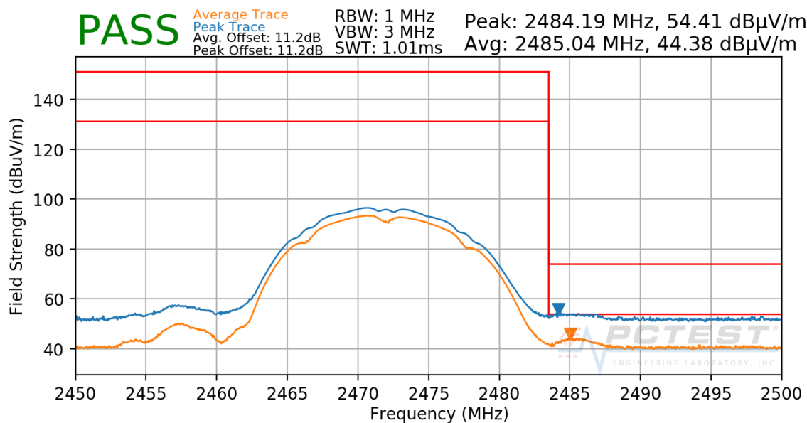
Plot 7-44. Radiated Restricted Upper Band Edge Measurement
