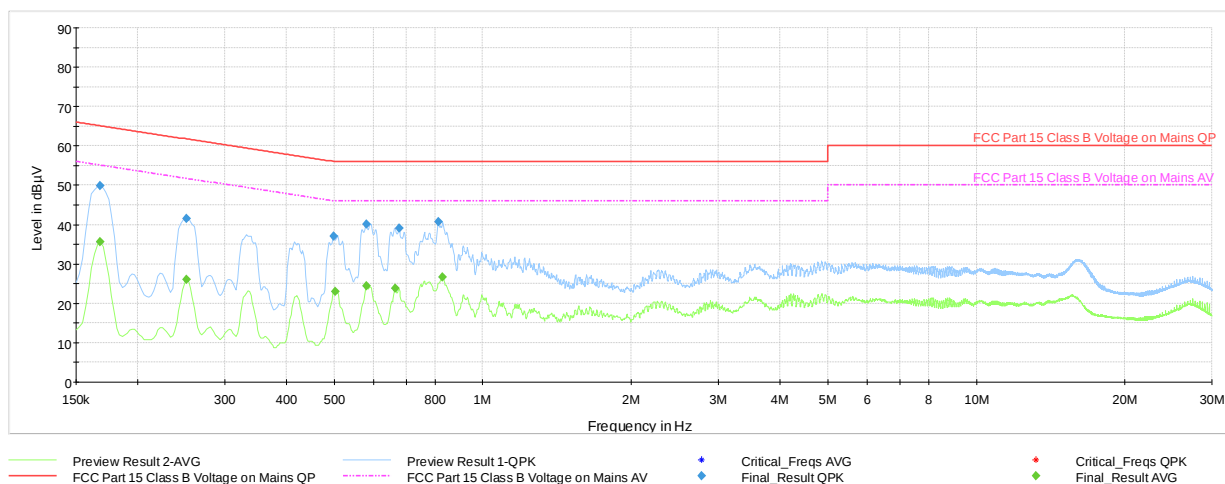
Plot 7-52. Line Conducted Plot with 802.11b Ch.6 (L1, with WCP + AC/DC Adapter)
