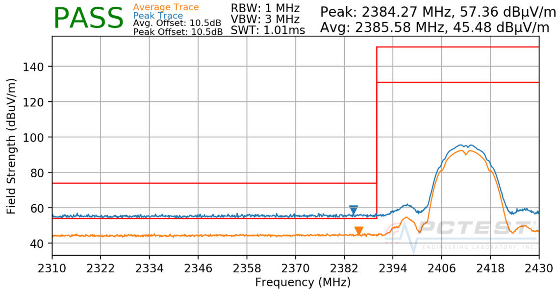
Plot 7-42. Radiated Restricted Lower Band Edge Measurement
