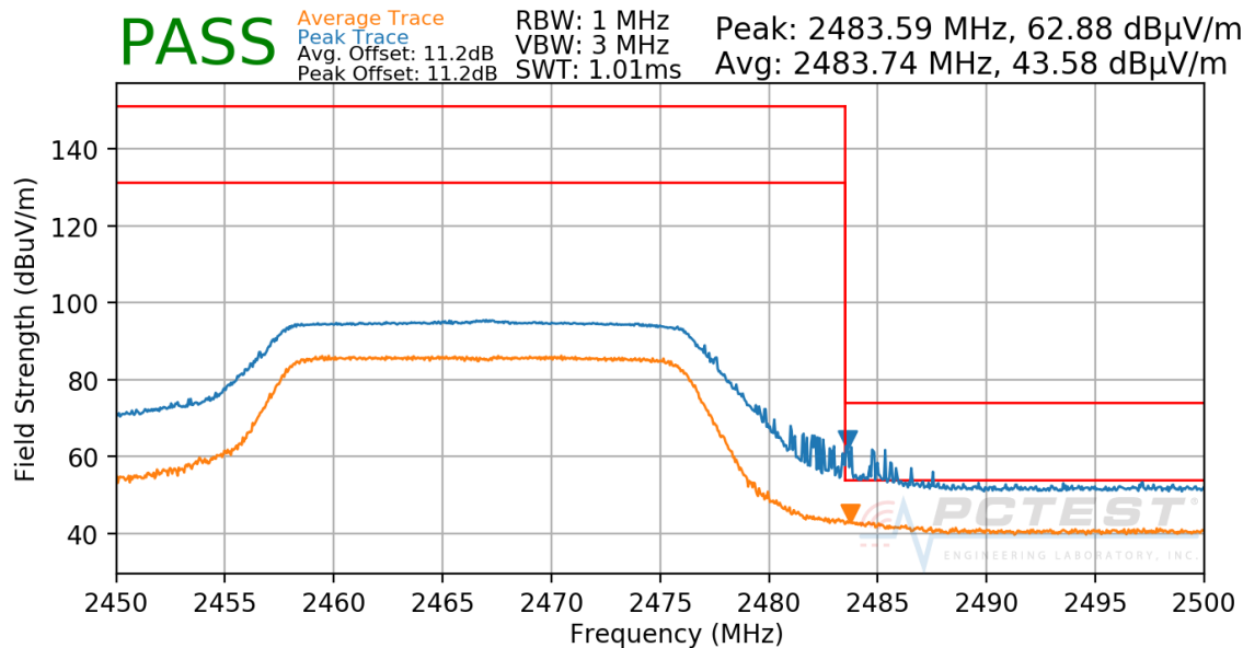
Plot 7-49. Radiated Restricted Upper Band Edge Measurement
