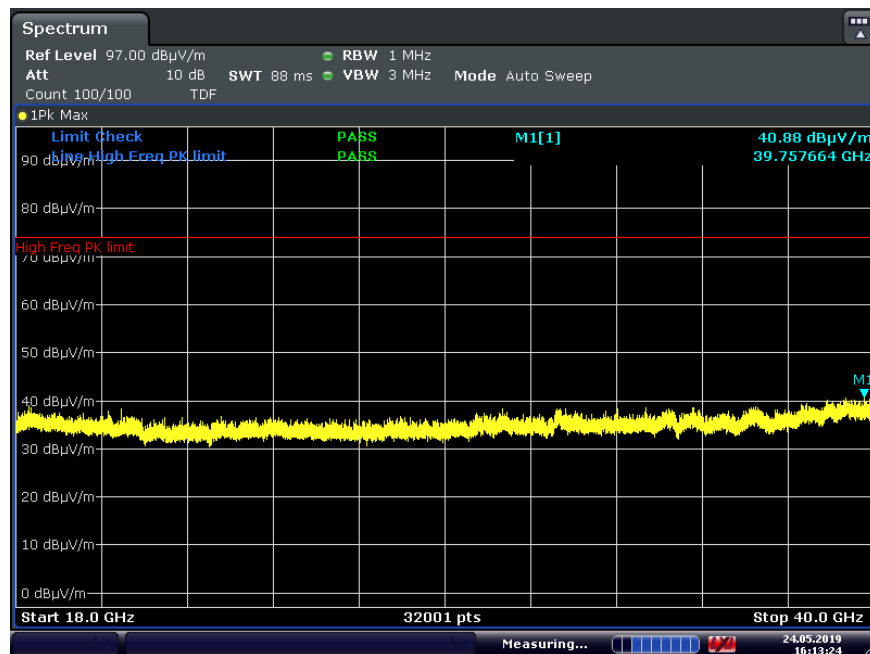
Plot 7-33. Radiated Spurious Plot Above 18GHz (1Mbps, ePA – Ch. 39, Ant. Pol. V)
