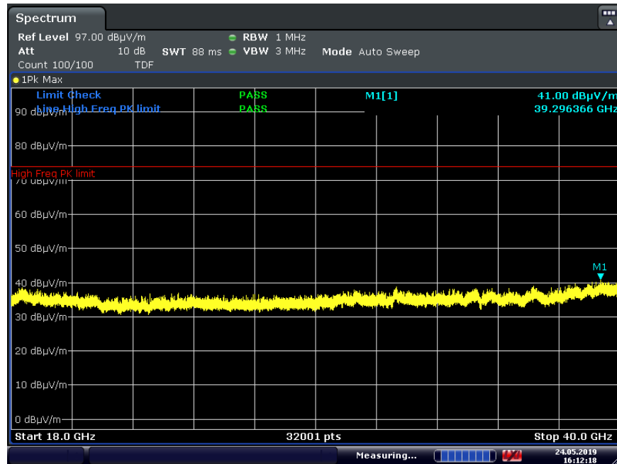
Plot 7-32. Radiated Spurious Plot Above 18GHz (1Mbps, ePA – Ch. 39, Ant. Pol. H)
