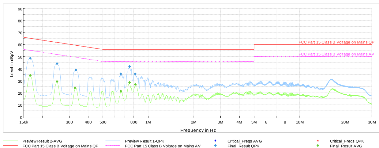
Plot 7-40. Line Conducted Plot with Bluetooth HDR (N- 4Mbps, ePA, Ch.38 with WCP + AC/DC Adapter)
