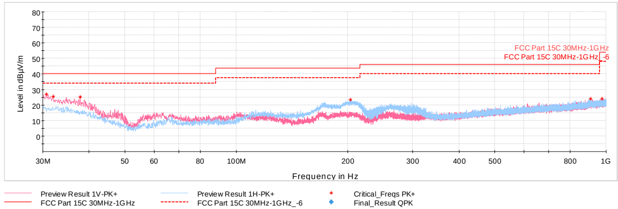
Plot 7-38. Radiated Spurious Plot below 1GHz (4Mbps, ePA – Ch.38 with WCP + AC/DC Adapter)
