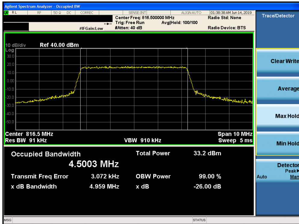
Plot 7-5. Occupied Bandwidth Plot (LTE Band 26, 5MHz QPSK – RB Size 25– Low Channel)
