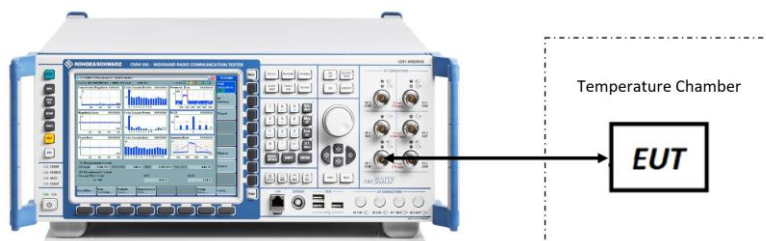
Figure 7-7. Test Instrument & Measurement Setup
