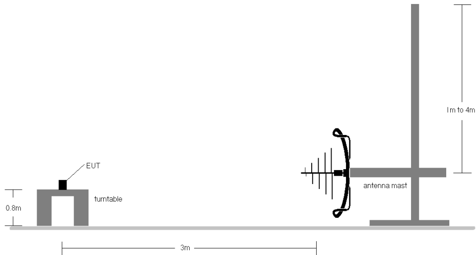
Figure 7-5. Test Instrument & Measurement Setup < 1GHz
