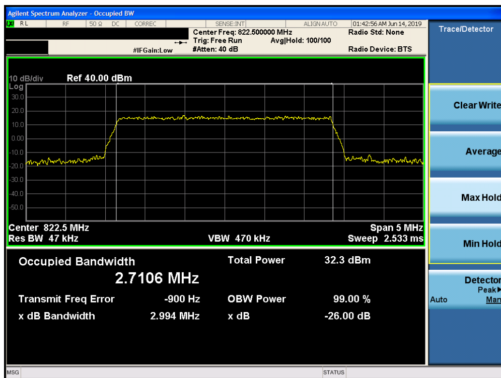
Plot 7-4. Occupied Bandwidth Plot (LTE Band 26, 3MHz 16-QAM – RB Size 15– High Channel)
