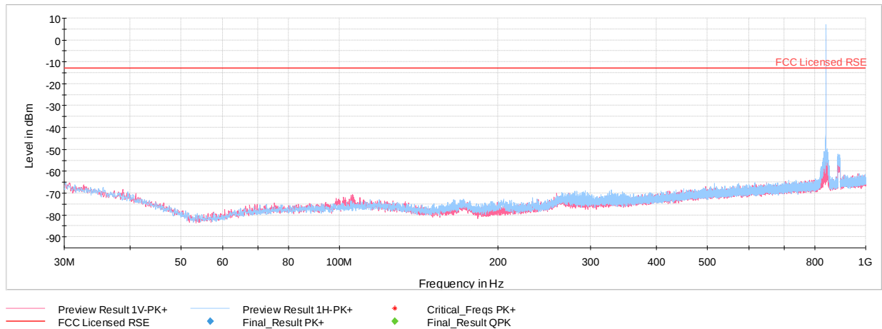
Plot 7-22. Radiated Spurious Plot - Below 1GHz (Band 26)
