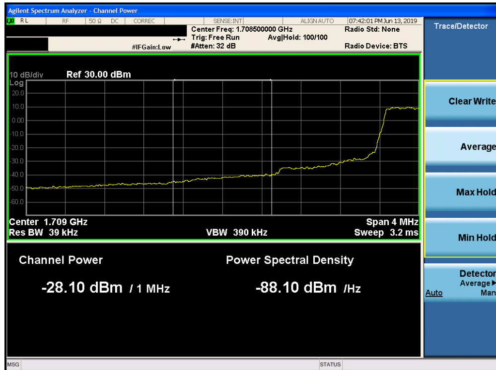
Plot 7-157. Lower Extended Band Edge Plot (Band 66 - 1.4.0MHz QPSK - Full RB Configuration)
