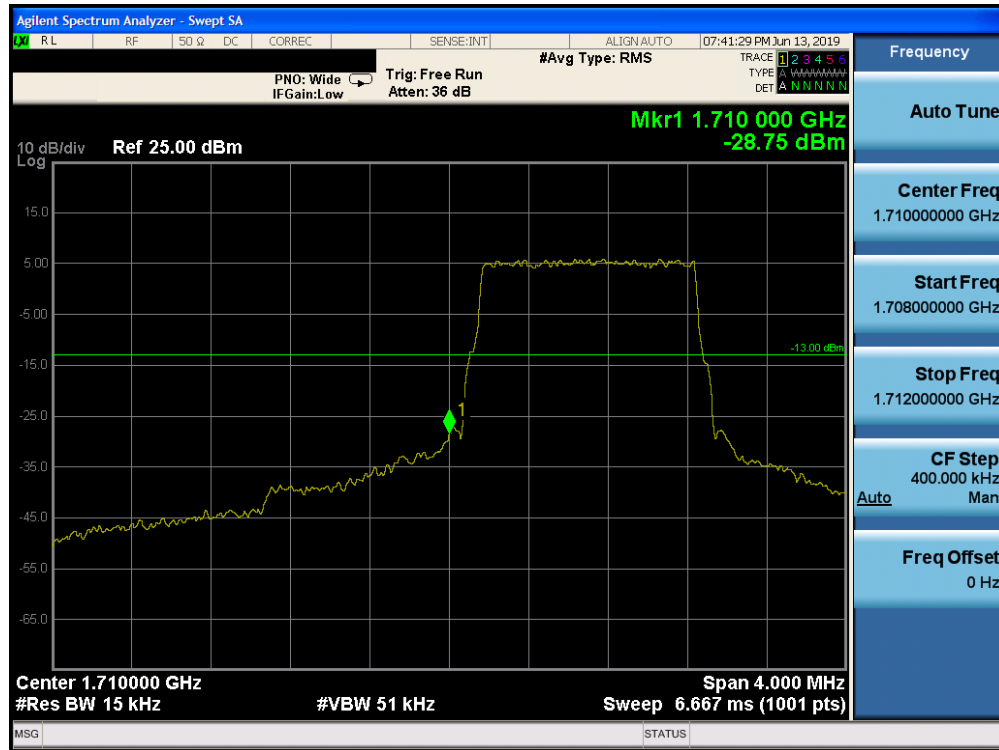
Plot 7-156. Lower Band Edge Plot (Band 66 - 1.4.0MHz QPSK - Full RB Configuration)
