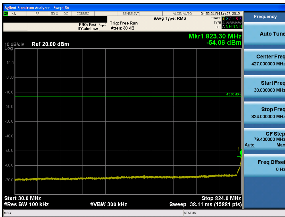
Plot 7-7. Conducted Spurious Plot (Cellular WCDMA Mode - Mid Channel)
