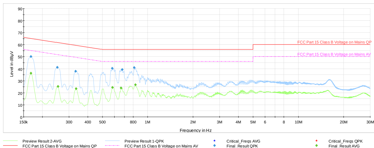
Plot 7-56. Line Conducted Plot with 802.11b Ch.6 (L1, with WCP + AC/DC Adapter)
