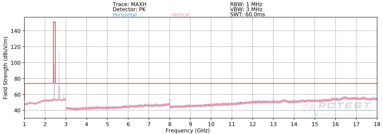
Plot 7-42. Radiated Spurious Plot Above 1GHz
