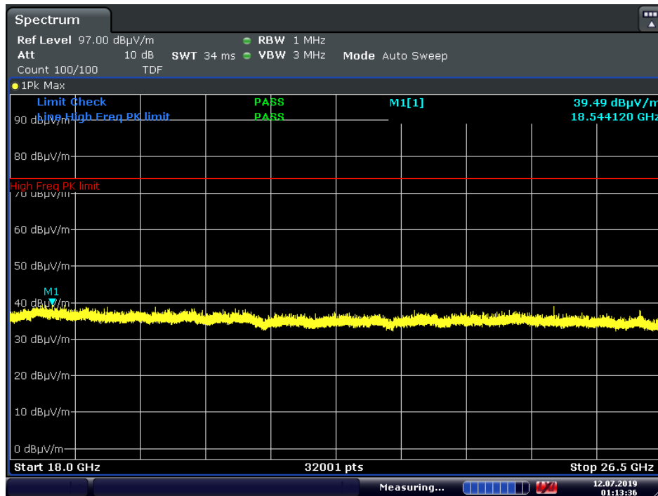
Plot 7-44. Radiated Spurious Plot Above 18GHz (Ant. Pol. V)
