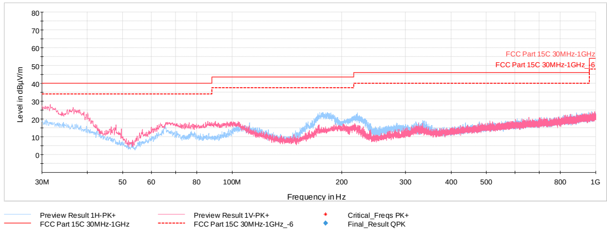
Plot 7-54. Radiated Spurious Plot Below 1GHz (802.11b – Ch.6, with WCP + AC/DC Adapter)
