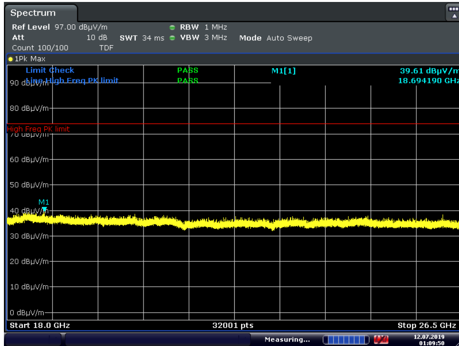
Plot 7-43. Radiated Spurious Plot Above 18GHz (Ant. Pol. H)
