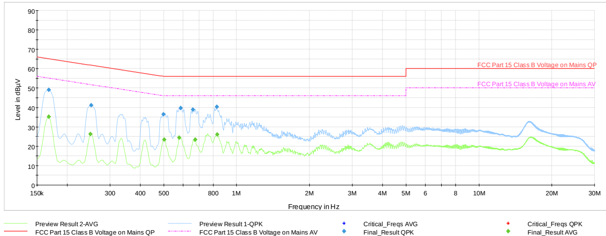
Plot 7-57. Line Conducted Plot with 802.11b Ch.6 (N, with WCP + AC/DC Adapter)
