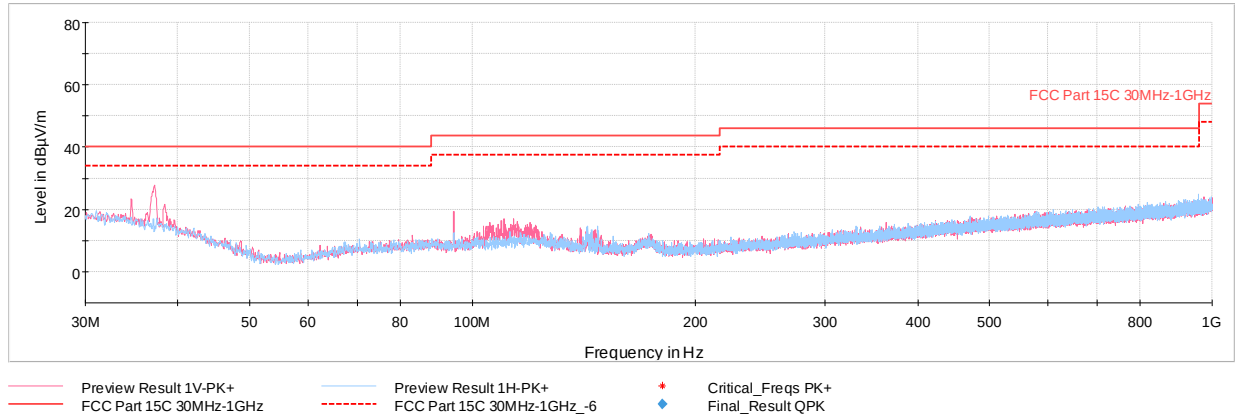
Plot 7-55. Radiated Spurious Plot Below 1GHz (with WCP + AC/DC Adapter)
