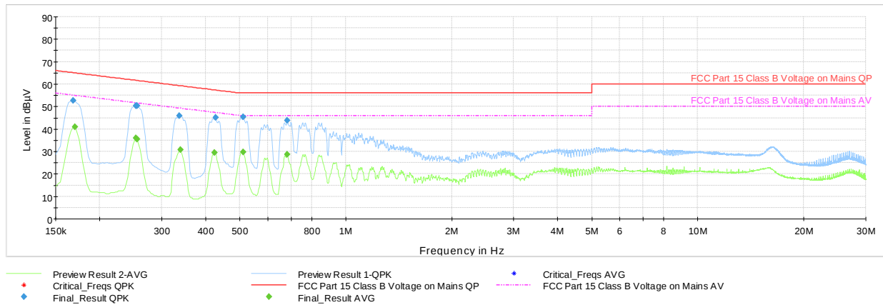
Plot 7-53. Line Conducted Plot with 802.11b Ch. 6 (L1, with WCP + AC/DC Adapter)
