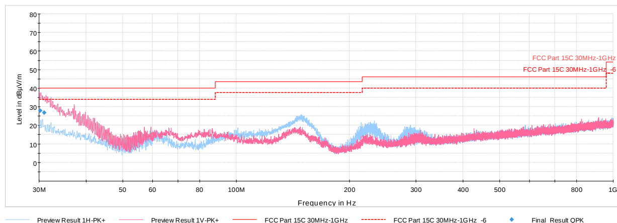
Plot 7-52. Radiated Spurious Plot below 1GHz (802.11b – Ch.6, with WCP + AC/DC Adapter)
