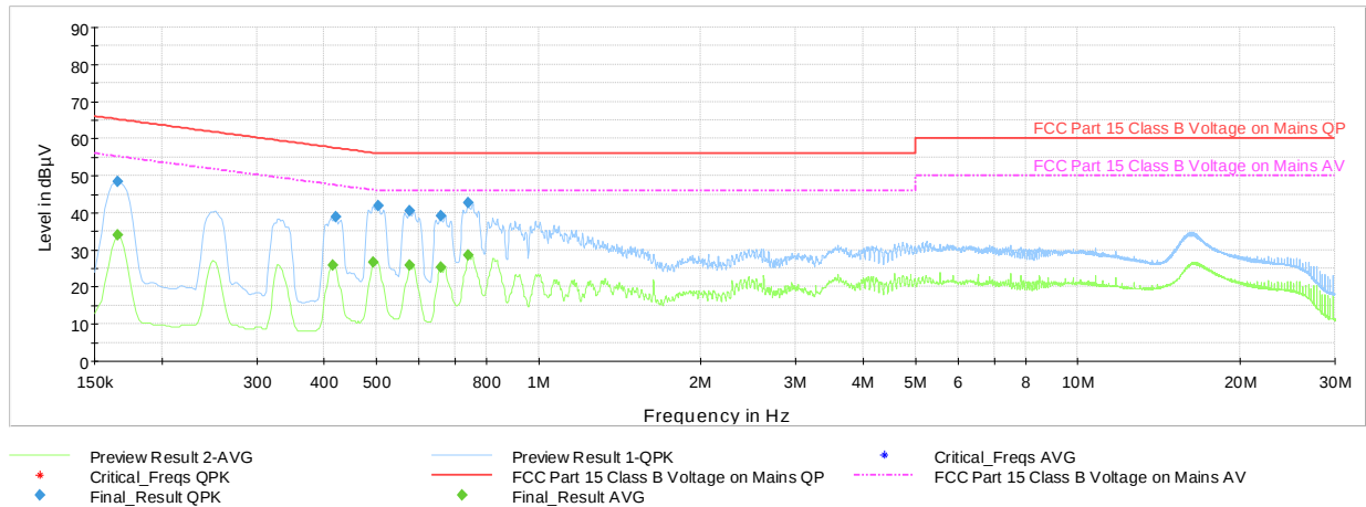
Plot 7-54. Line Conducted Plot with 802.11b Ch. 6 (N, with WCP + AC/DC Adapter)
