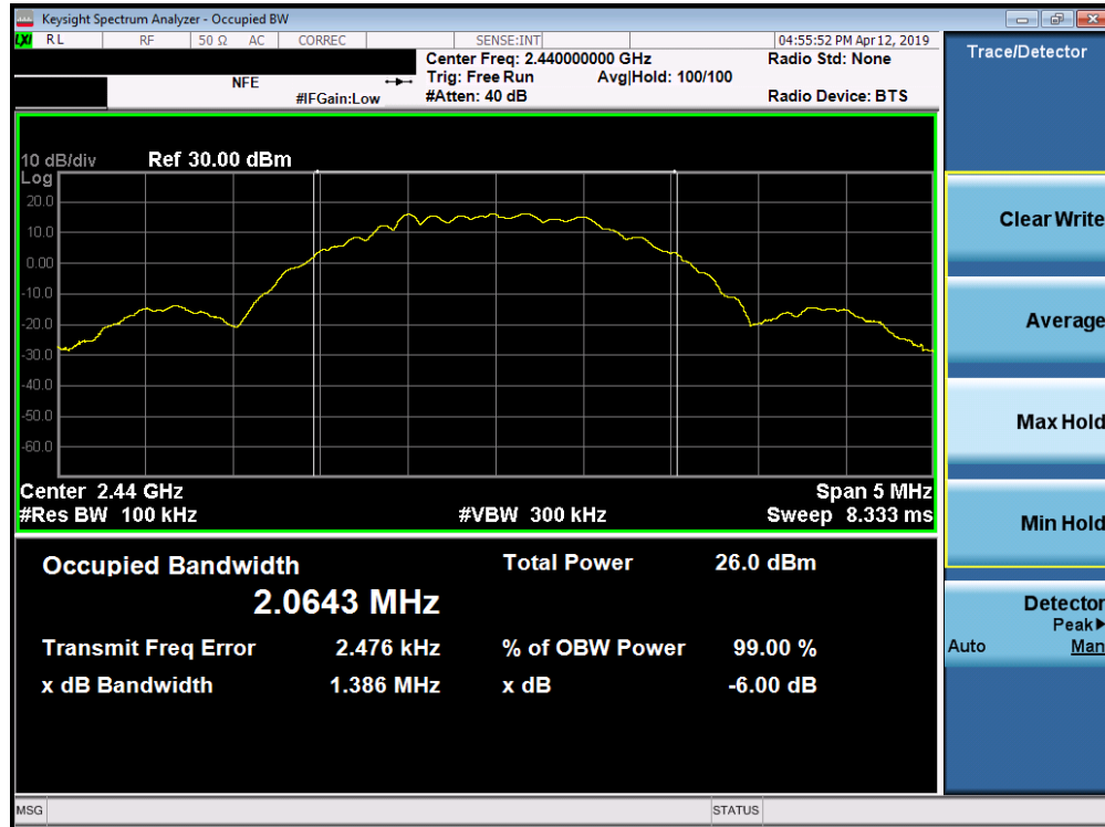
Plot 7-5. 6dB Bandwidth Plot (Bluetooth (LE), ePA – Ch. 19)
