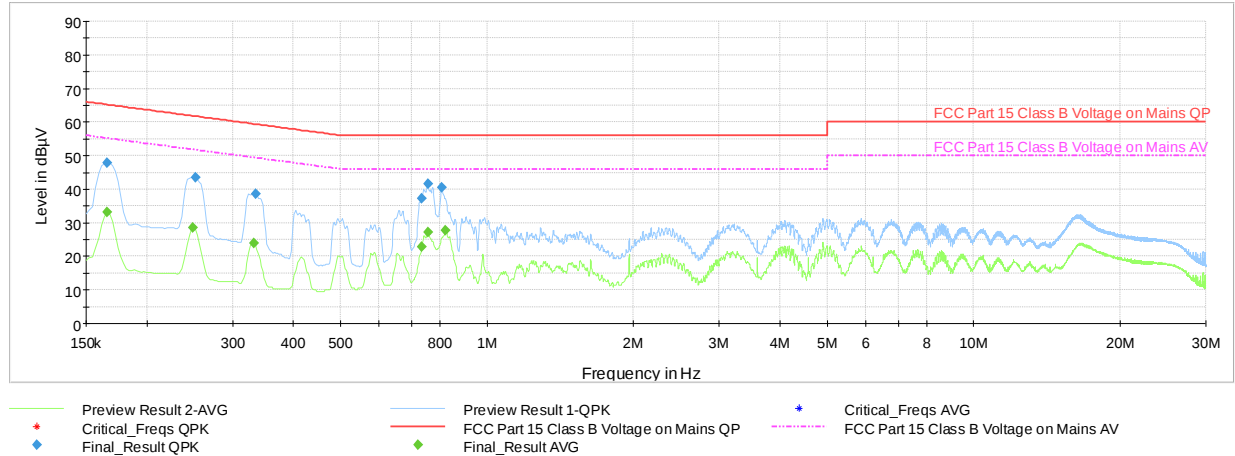
Plot 7-40. Line Conducted Plot with Bluetooth LE (N - 1Mbps, ePA, Ch.19 with WCP + AC/DC Adapter)
