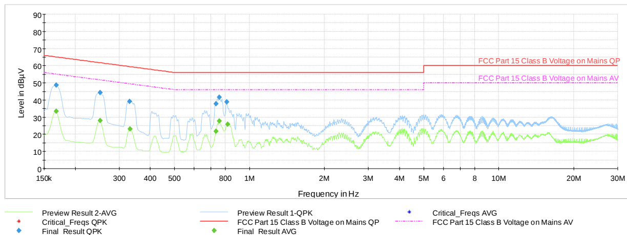
Plot 7-39. Line Conducted Plot with Bluetooth LE (L1 - 1Mbps, ePA, Ch.19 with WCP + AC/DC Adapter)
