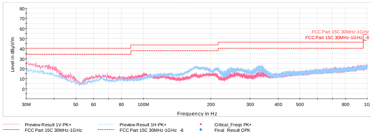
Plot 7-38. Radiated Spurious below 1GHz (4Mbps, HDR ePA, Ch.38 with WCP + AC/DC Adapter attached)
