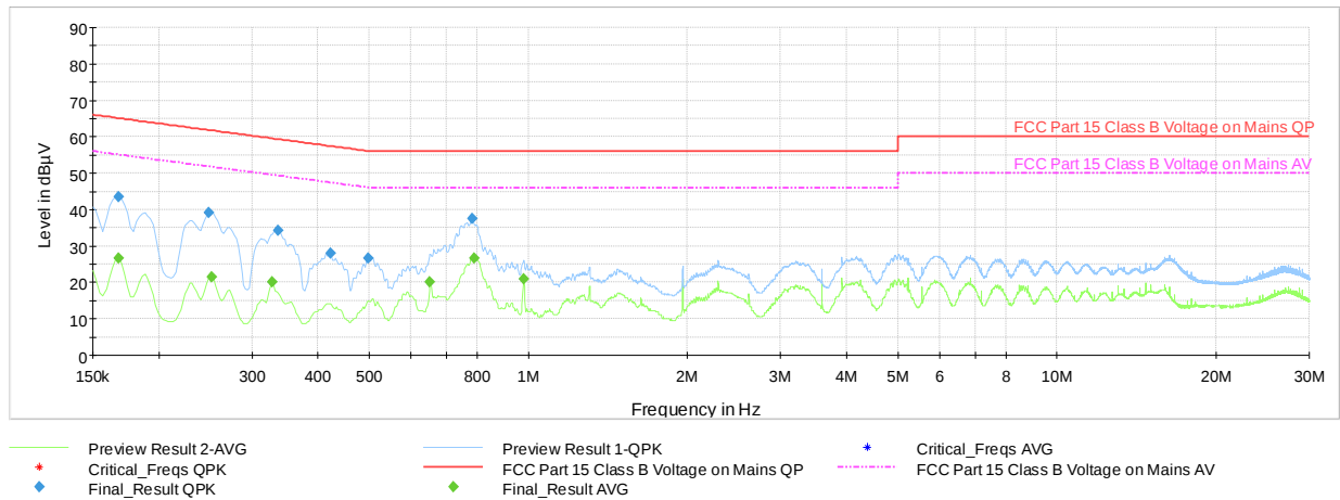
Plot 7-53. Line Conducted Plot with 802.11b Ch.6 (L1, with WCP + AC/DC Adapter)
