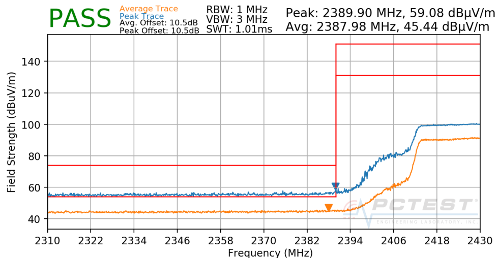
Plot 7-47. Radiated Restricted Lower Band Edge Measurement
