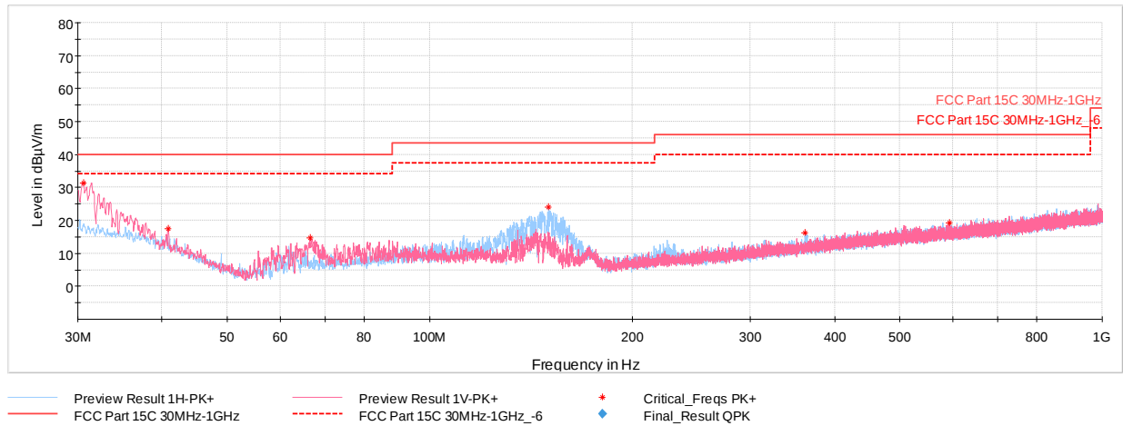
Plot 7-52. Radiated Spurious Plot below 1GHz (802.11b – Ch.6, with WCP + AC/DC Adapter)
