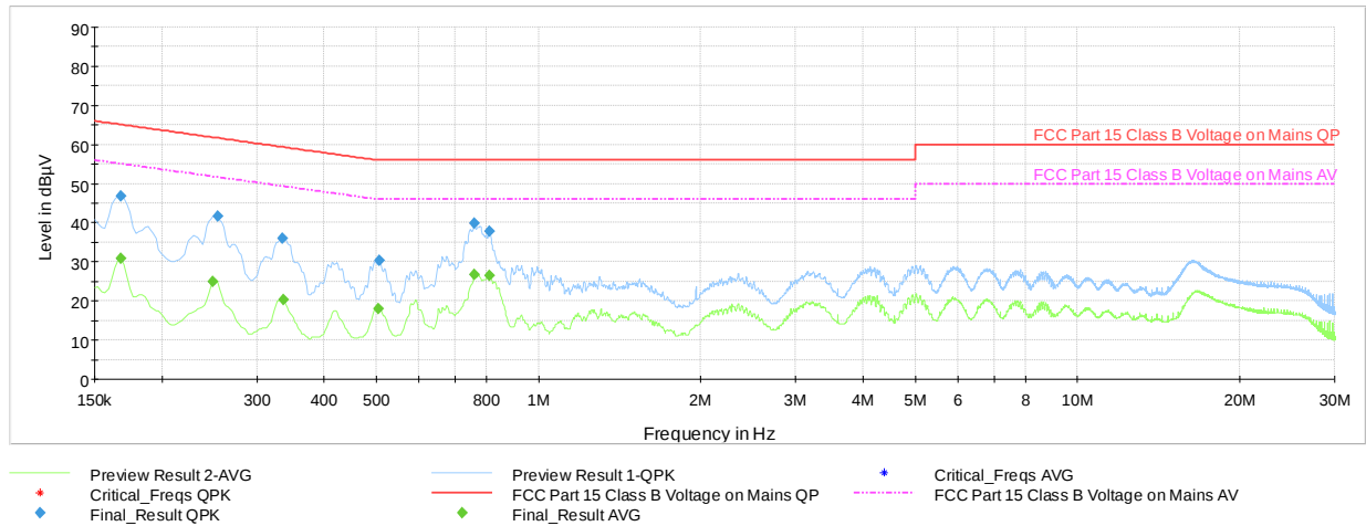
Plot 7-54. Line Conducted Plot with 802.11b Ch.6 (N, with WCP + AC/DC Adapter)
