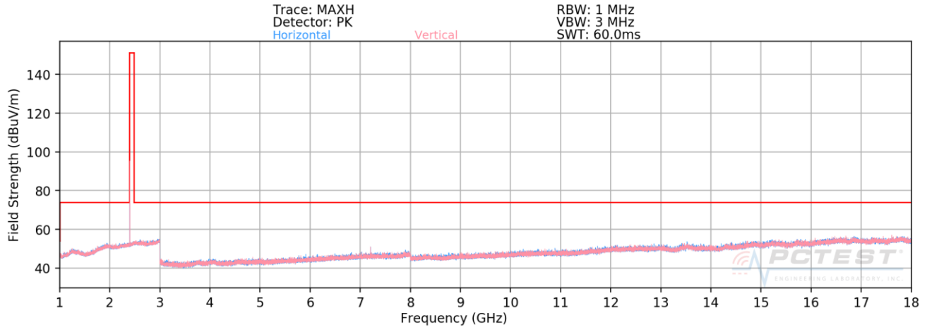
Plot 7-29. Radiated Spurious Plot Above 1GHz (1Mbps, ePA – Ch. 9)
