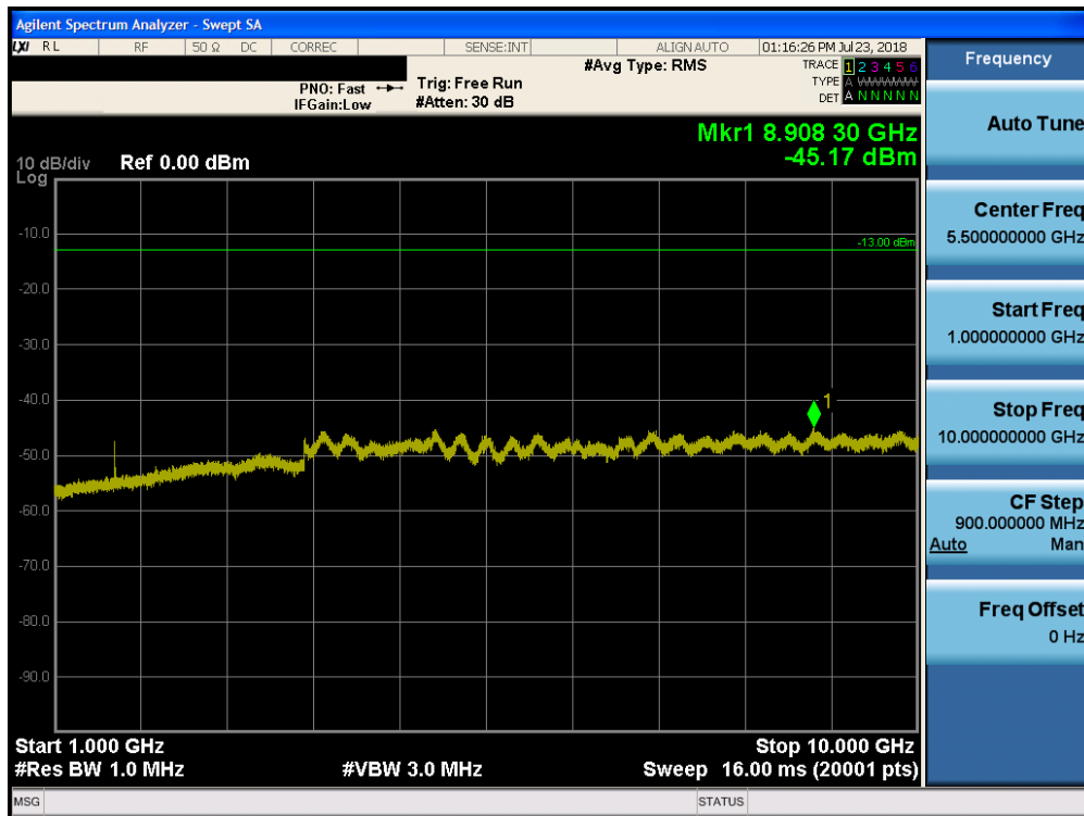
Plot 7-11. Conducted Spurious Plot (10MHz QPSK – RB Size 1, RB Offset 0)
