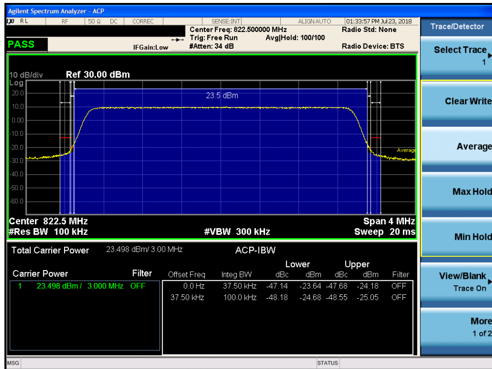
Plot 7-15. Channel Edge Plot (3MHz QPSK – RB Size 15 – High Channel)
