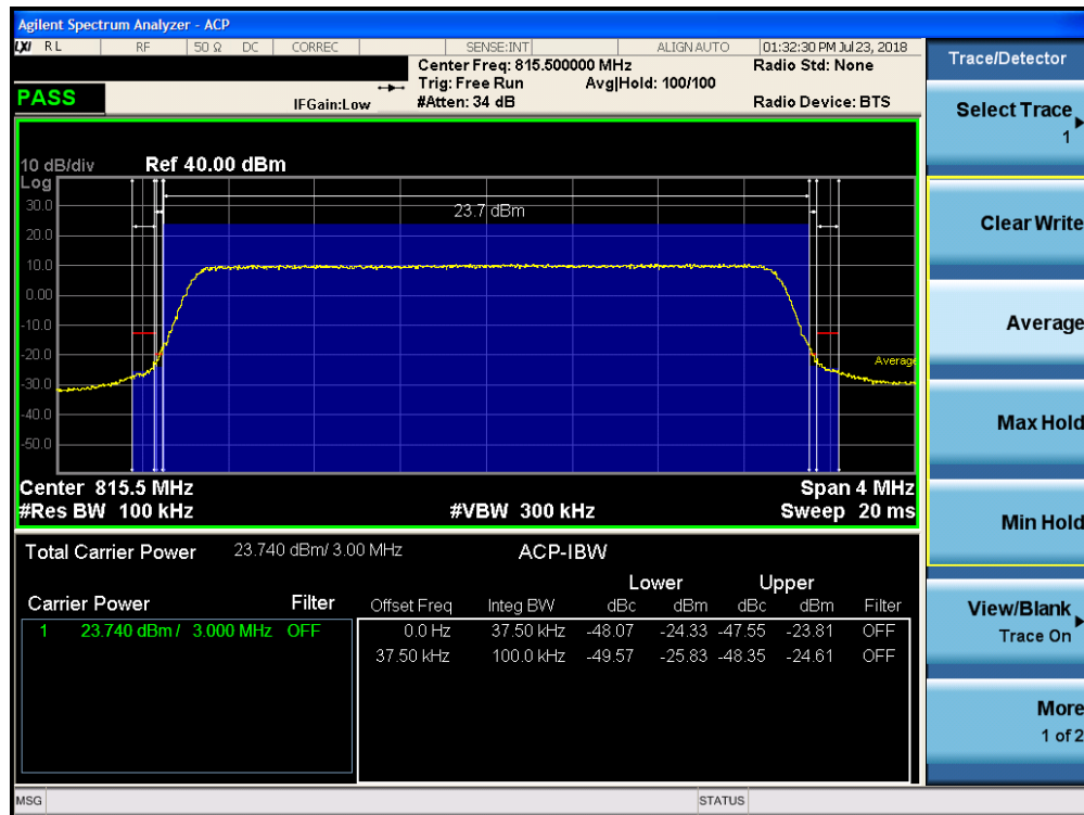
Plot 7-14. Channel Edge Plot (3MHz QPSK – RB Size 15– Low Channel)
