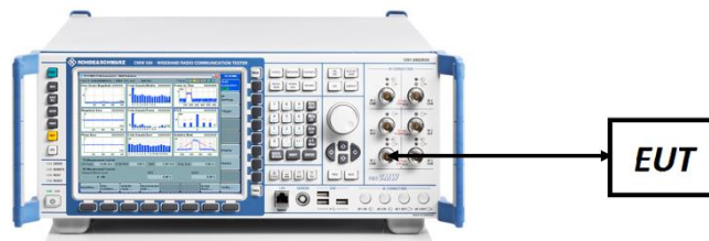
Figure 7-4. Conducted Power Measurement Setup
