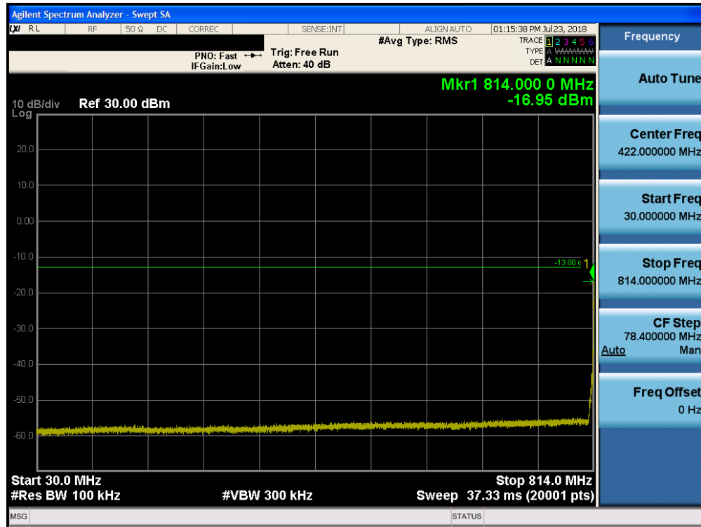
Plot 7-9. Conducted Spurious Plot (10MHz QPSK – RB Size 1, RB Offset 0)
