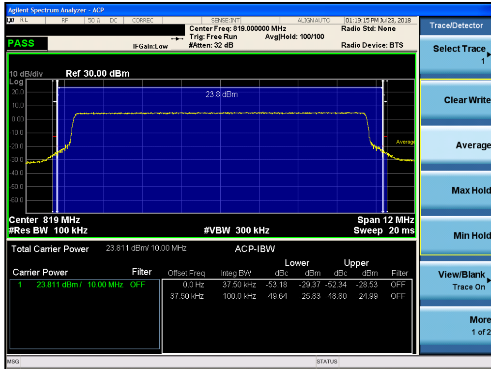
Plot 7-18. Channel Edge Plot (10MHz QPSK – RB Size 50)
