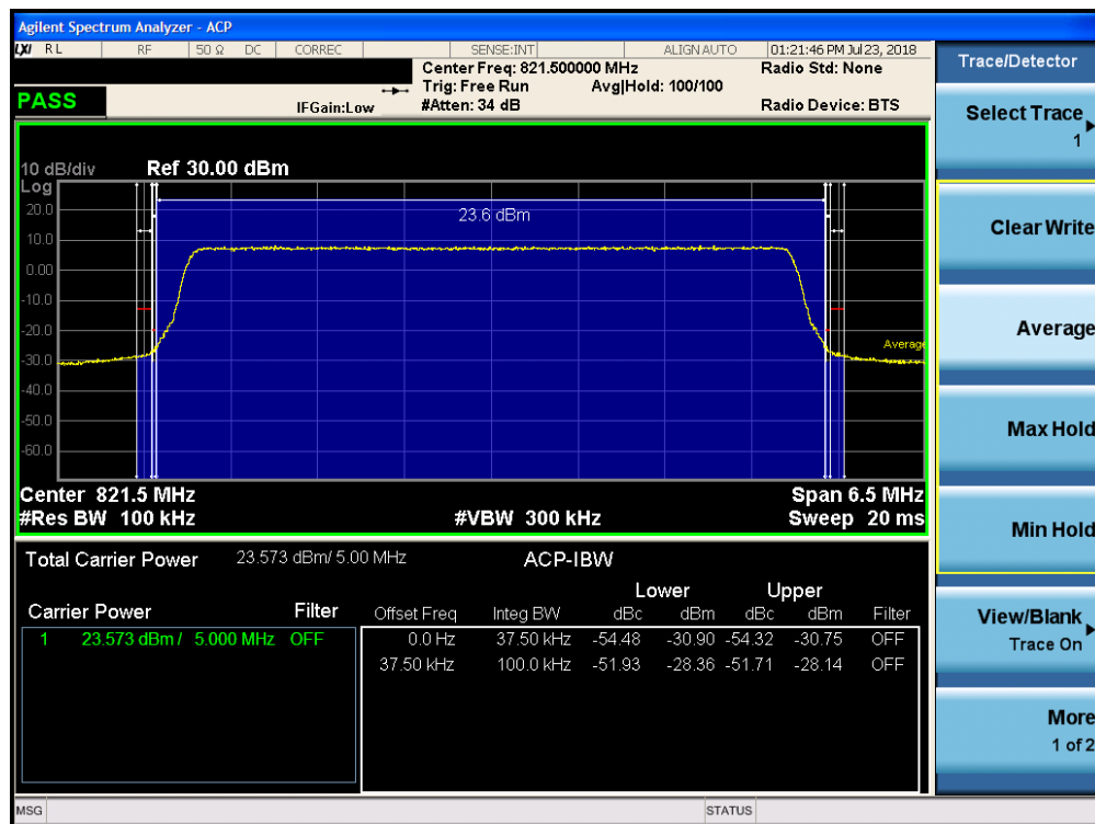
Plot 7-17. Channel Edge Plot (5MHz QPSK – RB Size 25 – High Channel)
