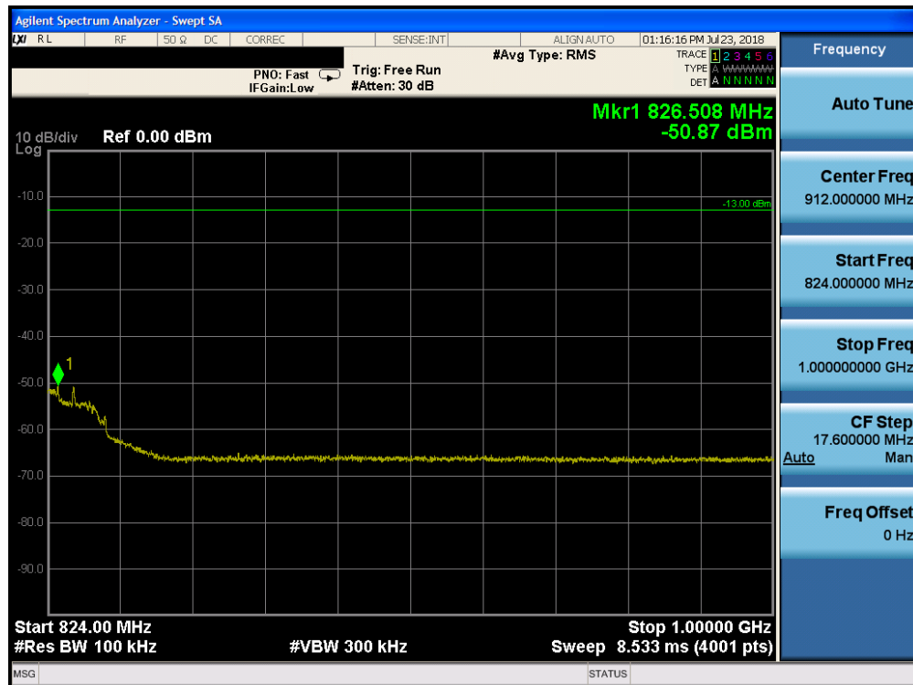
Plot 7-10. Conducted Spurious Plot (10MHz QPSK – RB Size 1, RB Offset 0)
