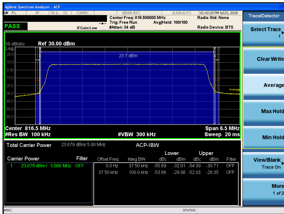
Plot 7-16. Channel Edge Plot (5MHz QPSK – RB Size 25– Low Channel)
