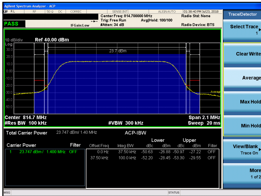
Plot 7-12. Channel Edge Plot (1.4MHz QPSK – RB Size 6– Low Channel)
