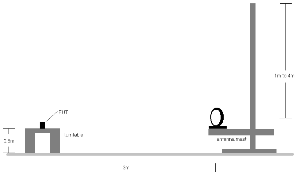
Figure 7-10. Radiated Test Setup < 30MHz
