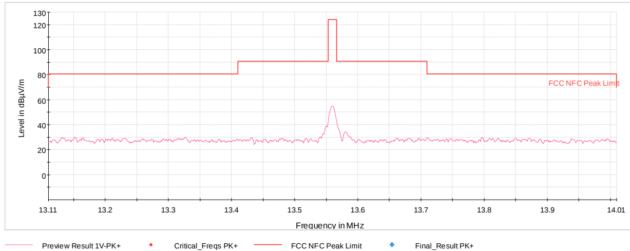
Plot 7-1. In Band Radiated Spurious Plot (CE A 848kdps, Pol. X)
