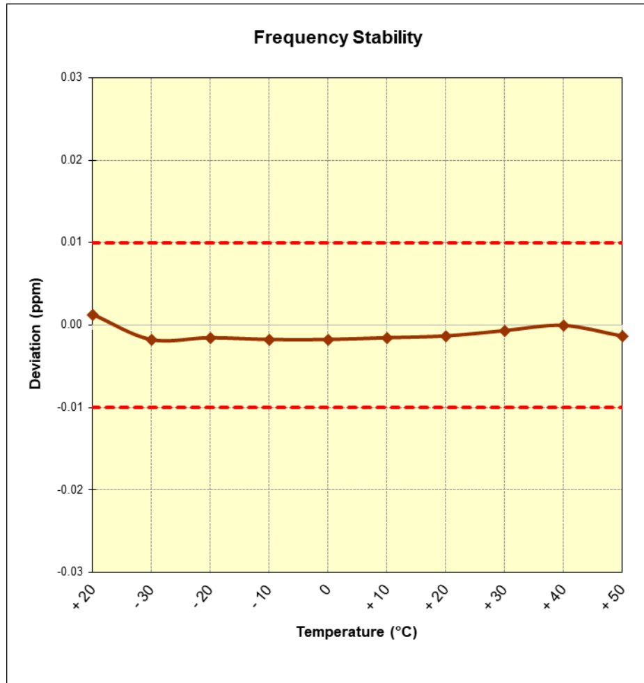
Figure 7-7. Frequency Stability Plot (CE A 848)
