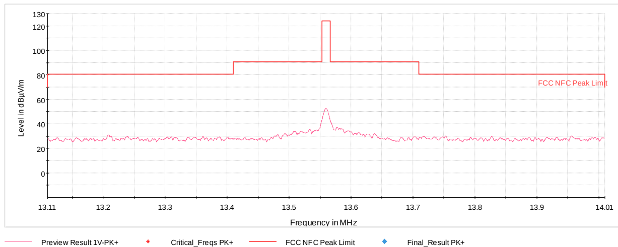
Plot 7-2. In Band Radiated Spurious Plot (Reader 100 Ask 1 out of 4, Pol. X)
