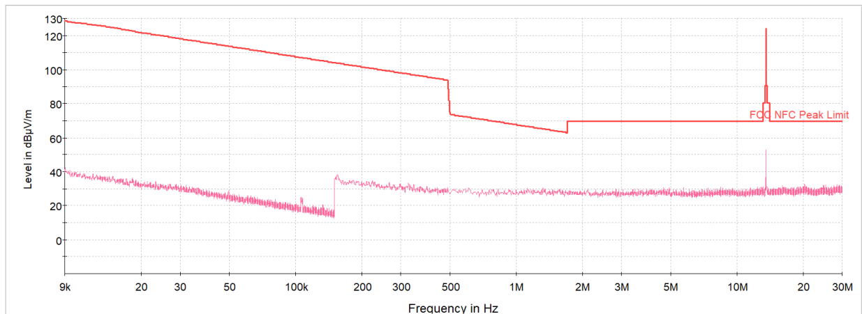
Plot 7-4. Radiated Spurious Plot 9kHz – 30MHz (Reader 100% Ask 1 out of 4 - Pol. X)
