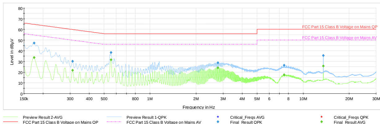
Plot 7-8. Line-Conducted Test Plot (N, with WCP + Laptop)
