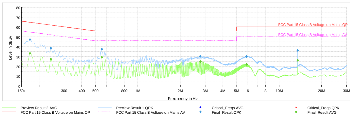
Plot 7-7. Line-Conducted Test Plot (L1, with WCP + Laptop)
