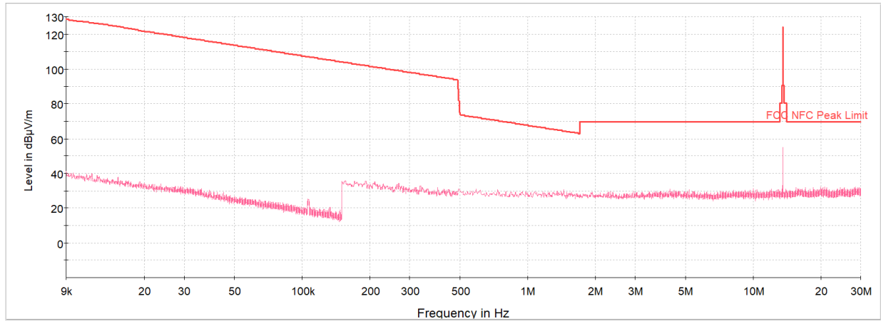
Plot 7-3. Radiated Spurious Plot 9kHz – 30MHz (CE A 848kbps - Pol. X)
