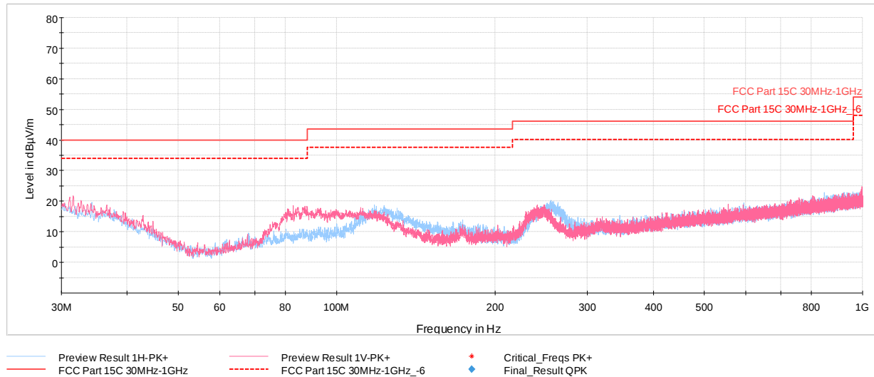
Plot 7-5. Radiated Spurious Plot 30MHz – 1GHz (CE A 848kdps, Pol. H & V, with AC/DC Adapter)
