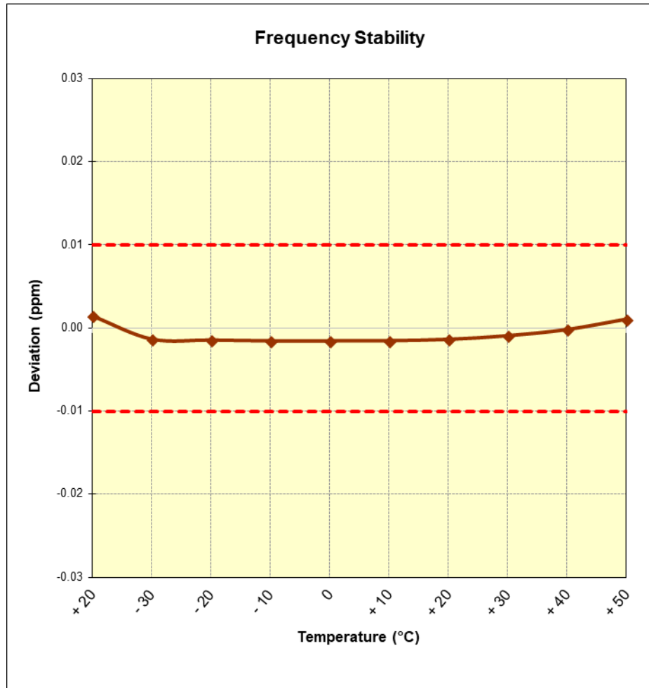
Figure 7-8. Frequency Stability Plot (Reader Ask 100% 1 out of 4)
