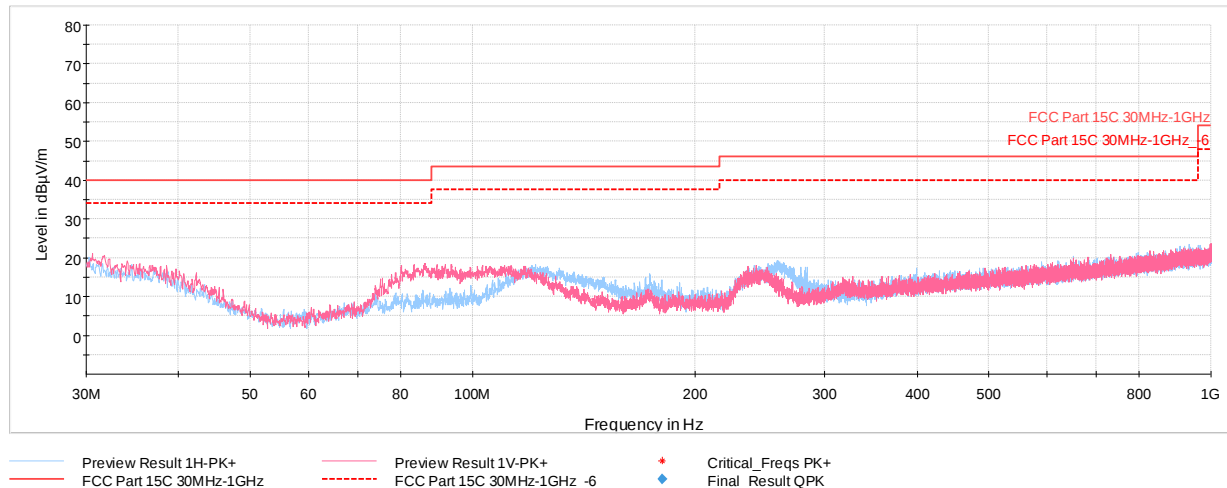
Plot 7-6. Radiated Spurious Plot 30MHz – 1GHz (Reader 100 Ask 1 out of 4, Pol. H & V with AC/DC Adapter)
