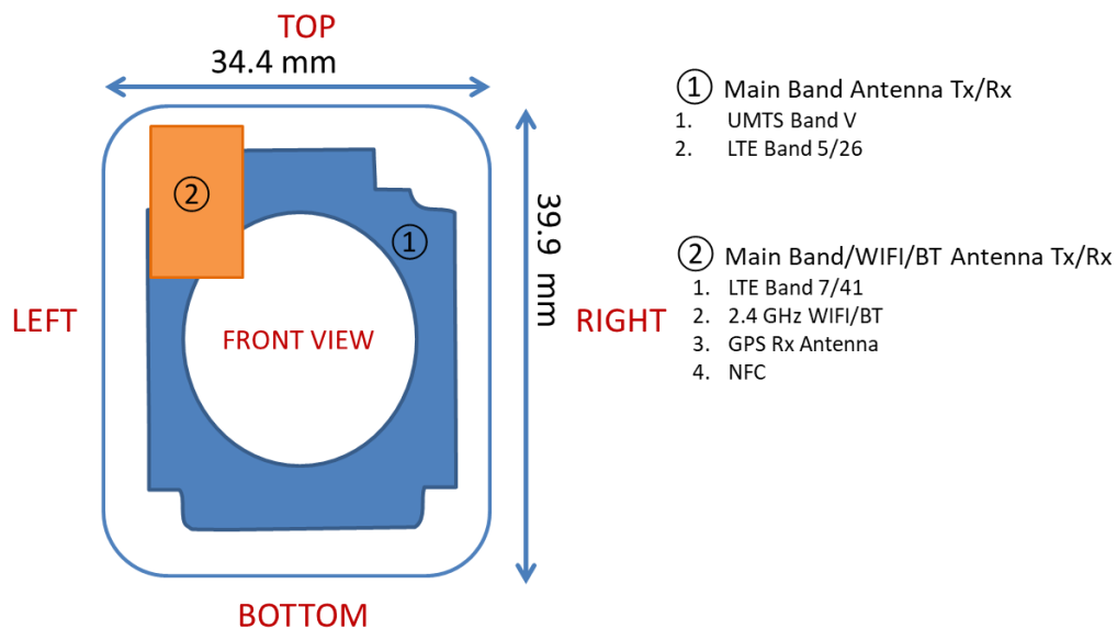
Figure F-1 DUT Antenna Locations
