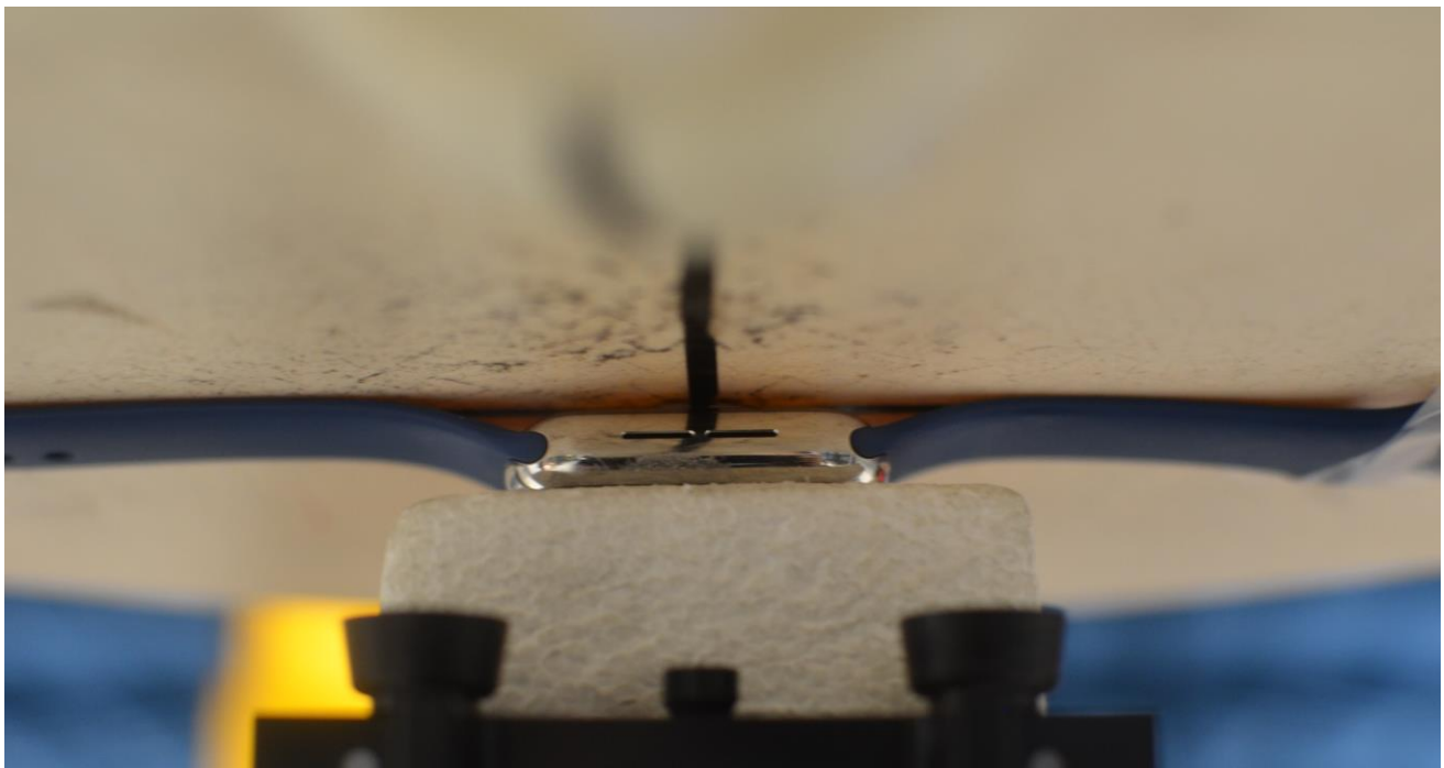
SAR Test Setup Photo 10: Stainless Steel with Sport wristband, Back side at 0.0 cm
