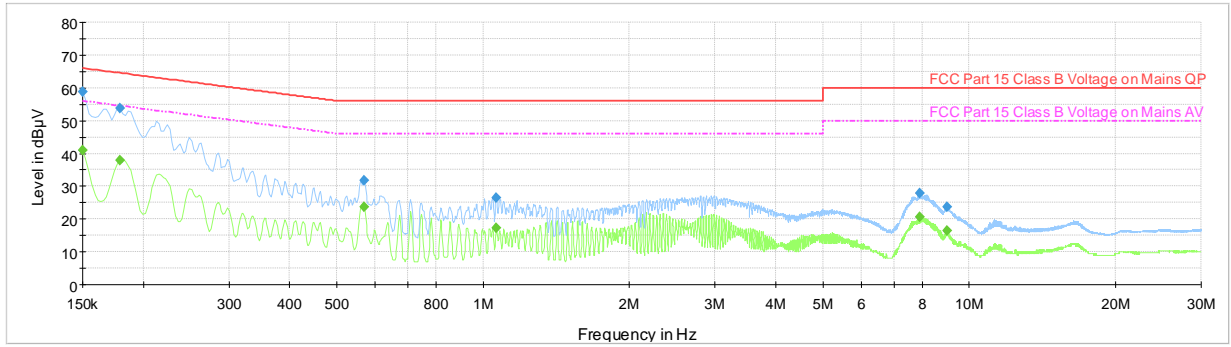
Plot 7-47. Line Conducted Plot with 802.11b (N with WCP + Laptop)
