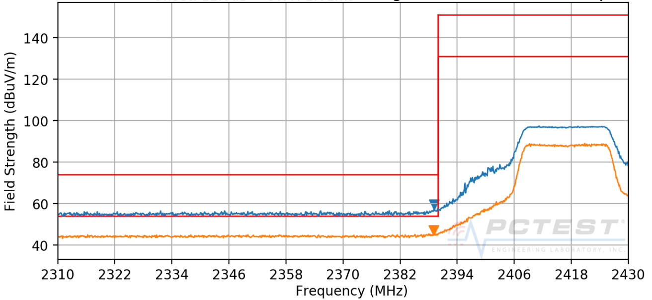
Plot 7-40. Radiated Restricted Lower Band Edge Measurement (Average & Peak)
