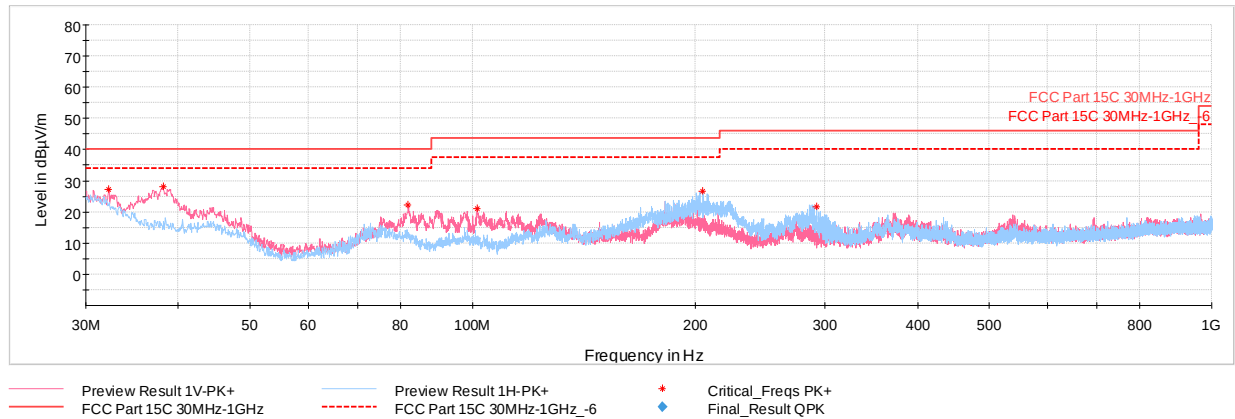
Plot 7-54. Radiated Spurious Plot below 1GHz (1Mbps, ePA, Pol. H & V, with WCP + Laptop)
