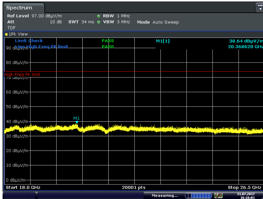
Plot 7-21. Radiated Spurious Plot above 18GHz (Pol. H)
