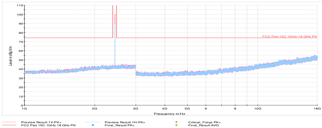
Plot 7-19. Radiated Spurious Plot above 1GHz (BT – Ch. 39, Ant. Pol. H & V)
