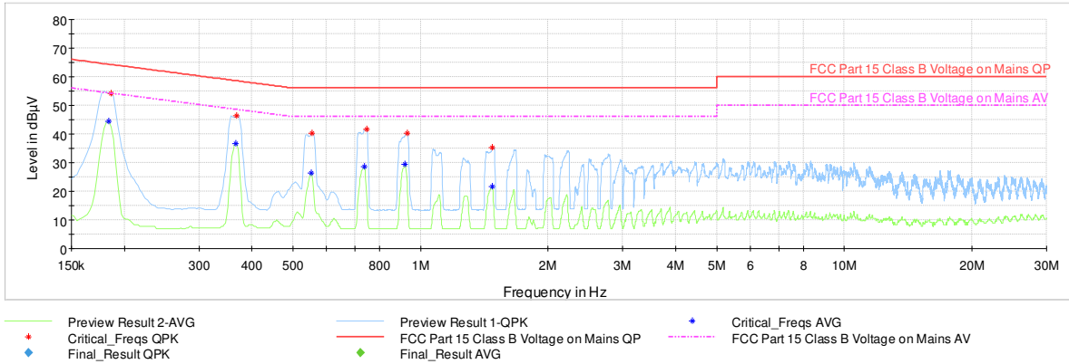
Plot 7-30. Line Conducted Plot with Bluetooth LE with AC Adapter (N)
