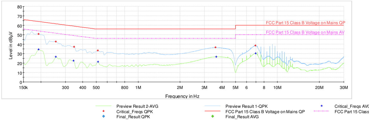
Plot 7-32. Line Conducted Plot with Bluetooth LE with Laptop (N)
