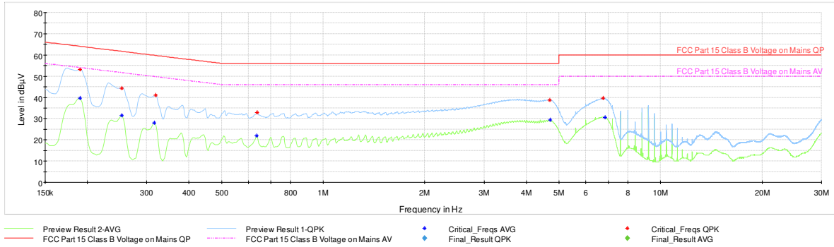
Plot 7-28. Line Conducted Plot with Bluetooth LE with Laptop (L1)
