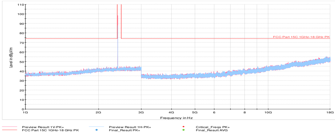
Plot 7-18. Radiated Spurious Plot above 1GHz (BT – Ch. 0, Ant. Pol. H & V)
