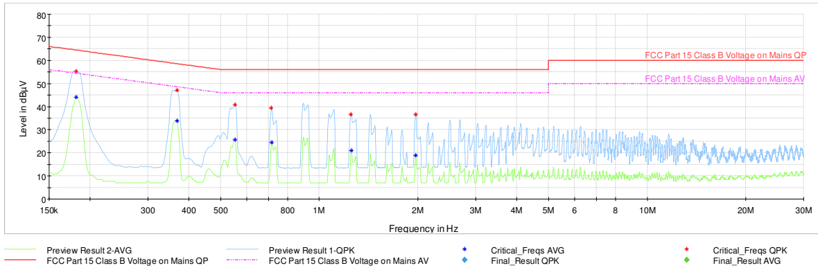
Plot 7-26. Line Conducted Plot with Bluetooth LE with AC Adapter (L1)
