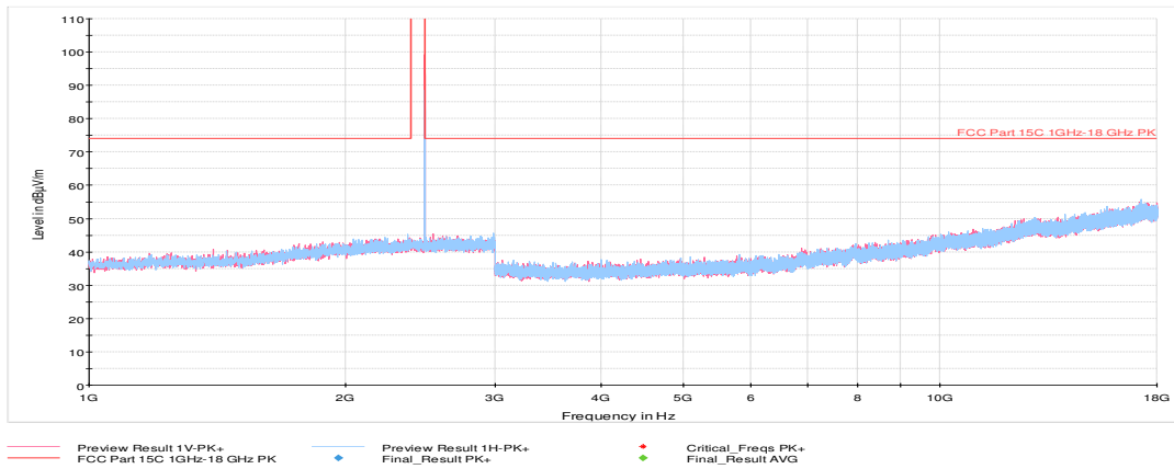
Plot 7-20. Radiated Spurious Plot above 1GHz (BT – Ch. 78, Ant. Pol. H & V)
