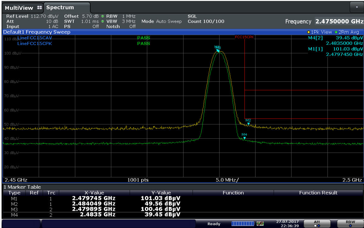
Plot 7-24. Radiated Restricted Upper Band Edge Measurement (Average & Peak)
