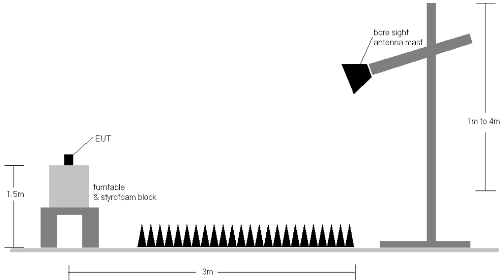
Figure 7-7. Radiated Test Setup >1GHz
