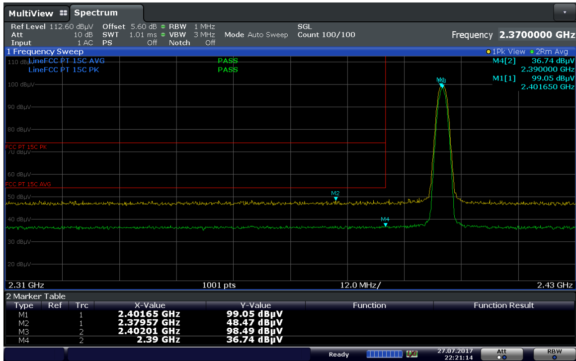
Plot 7-23. Radiated Restricted Lower Band Edge Measurement (Average & Peak)
