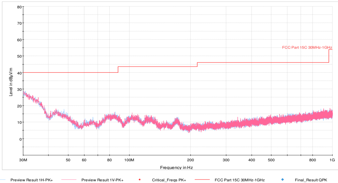
Plot 7-25. Radiated Spurious Plot below 1GHz (Pol. H & V)
