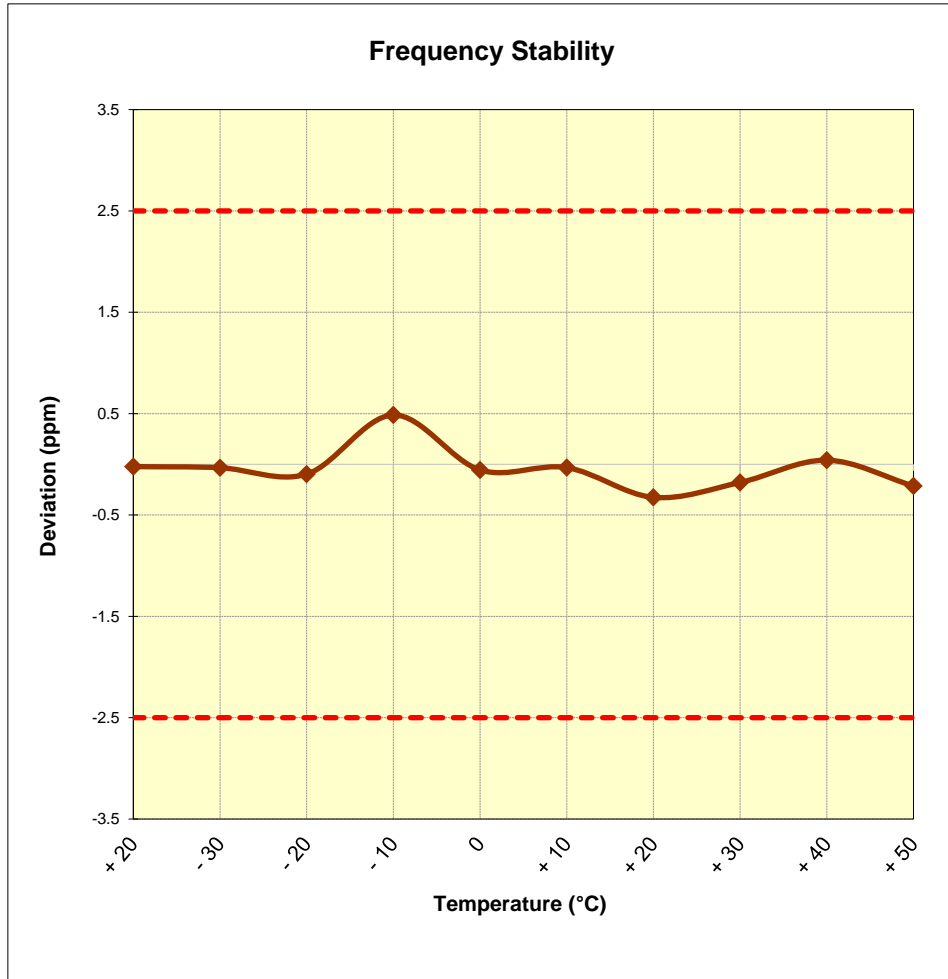
Figure 7-7. Frequency Stability Graph (Band 5/26)
