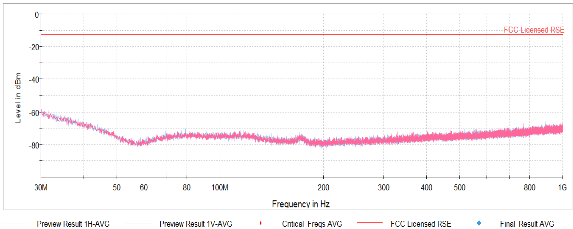
Plot 7-52. Radiated Spurious Plot (Band 7 – 10.0MHz QPSK – RB Size 50)
