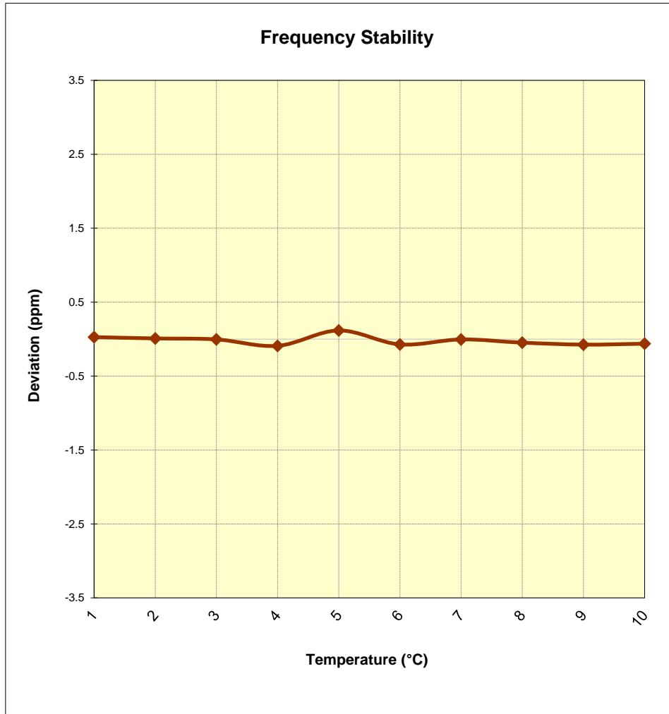
Figure 7-8. Frequency Stability Graph (Band 7)
