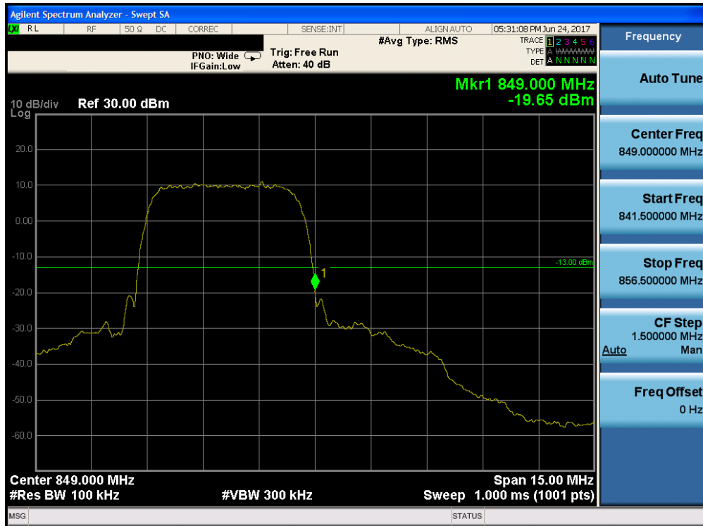
Plot 7-12. Band Edge Plot (Cellular WCDMA Mode – Ch. 4233)
