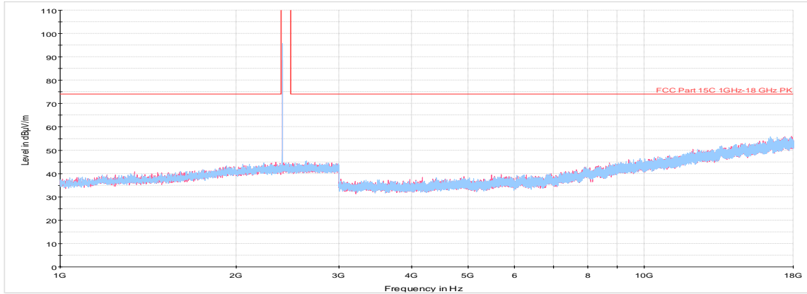
Plot 7-61. Radiated Spurious Plot above 1GHz (BT ePA – Ch. 0, Ant. Pol. H & V)
