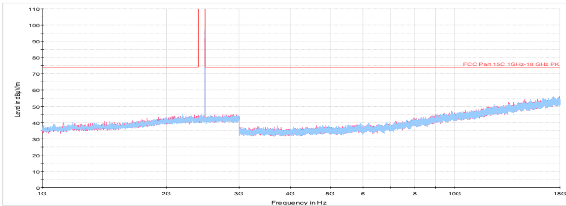
Plot 7-63. Radiated Spurious Plot above 1GHz (BT ePA – Ch. 78, Ant. Pol. H & V)
