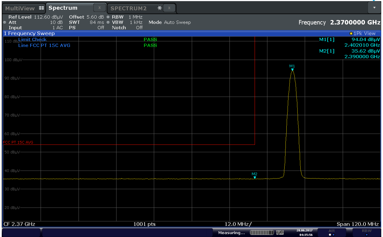
Plot 7-68. Radiated Restricted Lower Band Edge Measurement (Average)
