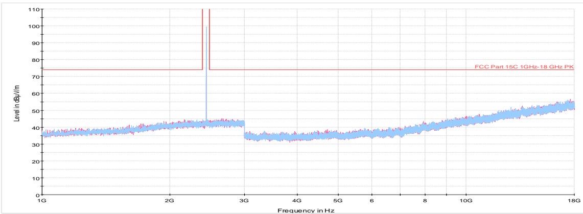
Plot 7-62. Radiated Spurious Plot above 1GHz (BT ePA – Ch. 39, Ant. Pol. H & V)
