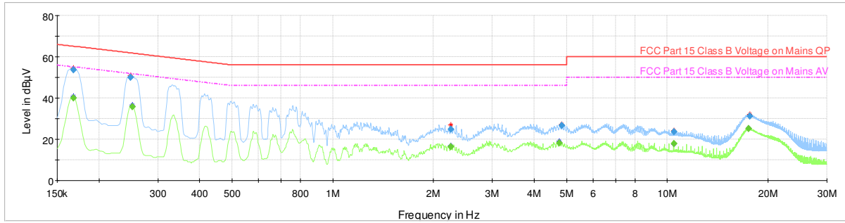
Plot 7-52. Line Conducted Plot with 802.11b (N)
