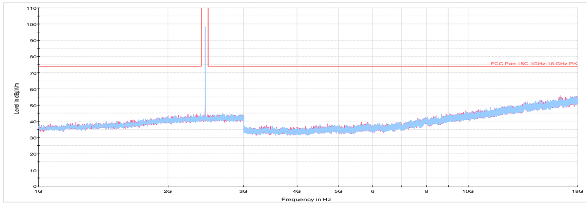
Plot 7-30. Radiated Spurious Plot above 1GHz (GFSK ePA – Ch. 39, Ant. Pol. H & V)
