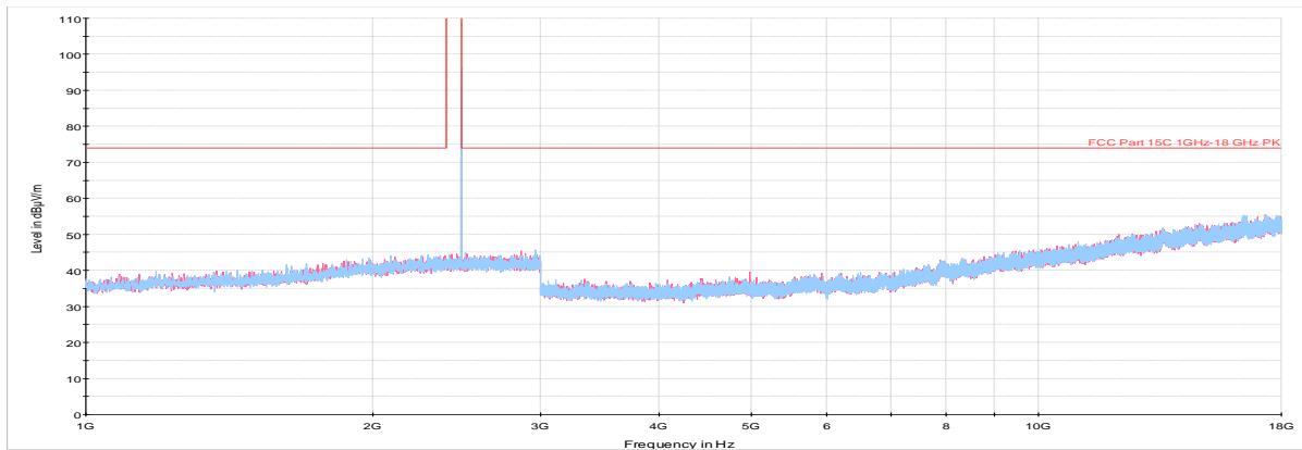
Plot 7-31. Radiated Spurious Plot above 1GHz (GFSK ePA – Ch. 78, Ant. Pol. H & V)
