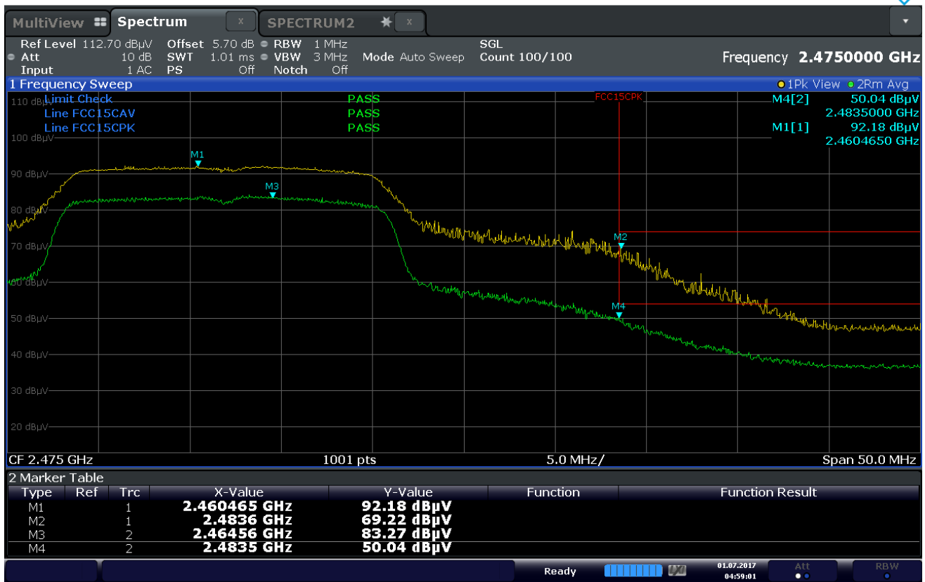
Plot 7-47. Radiated Restricted Upper Band Edge Measurement (Average & Peak)
