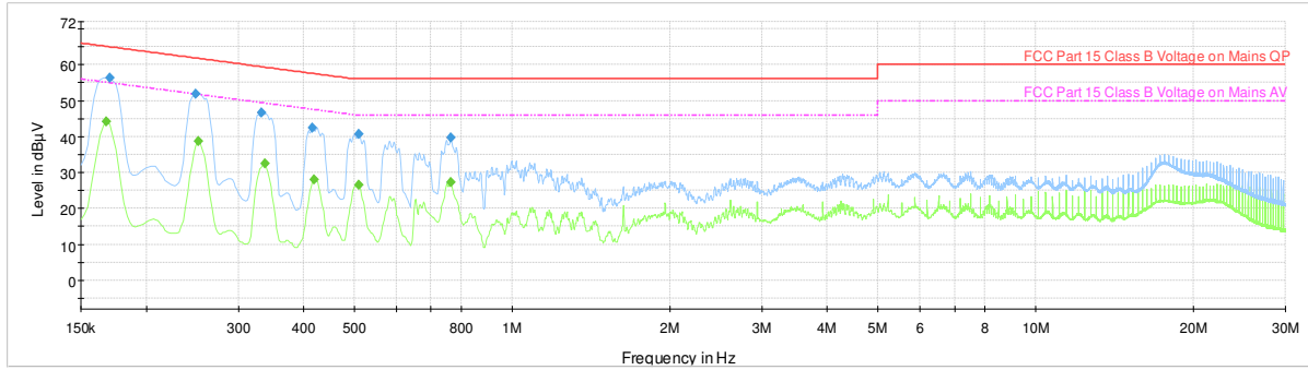
Plot 7-51. Line Conducted Plot with 802.11b (L1)
