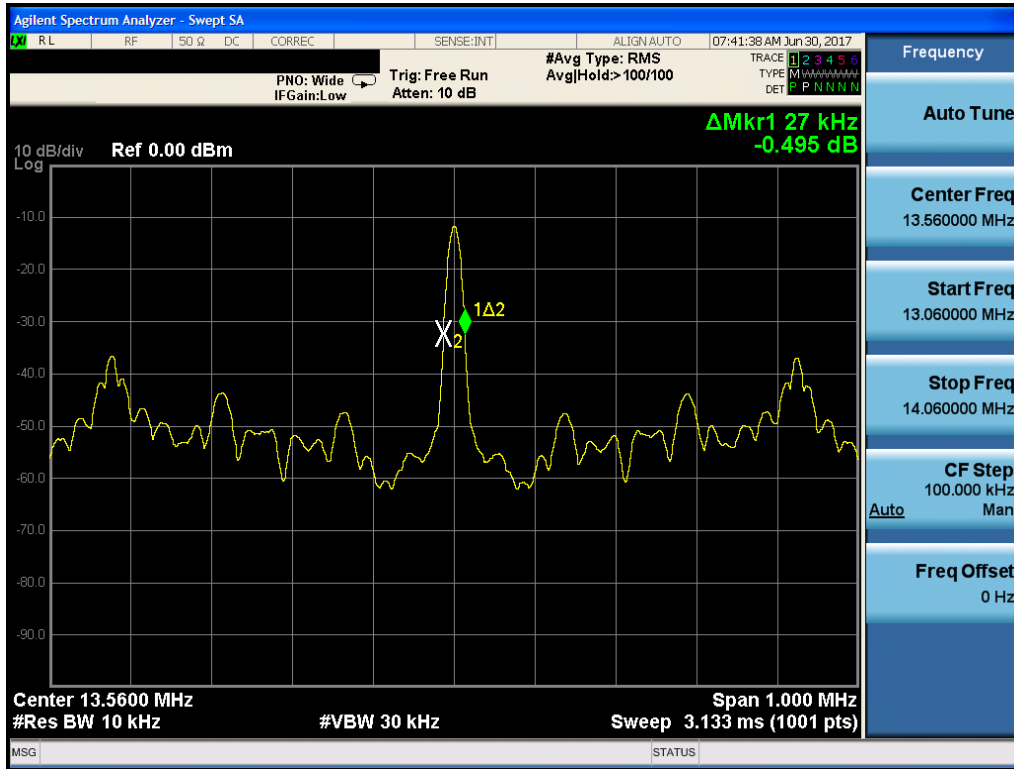
Figure 7-4. 20dB Bandwidth Plot (CE F 424kbps)
