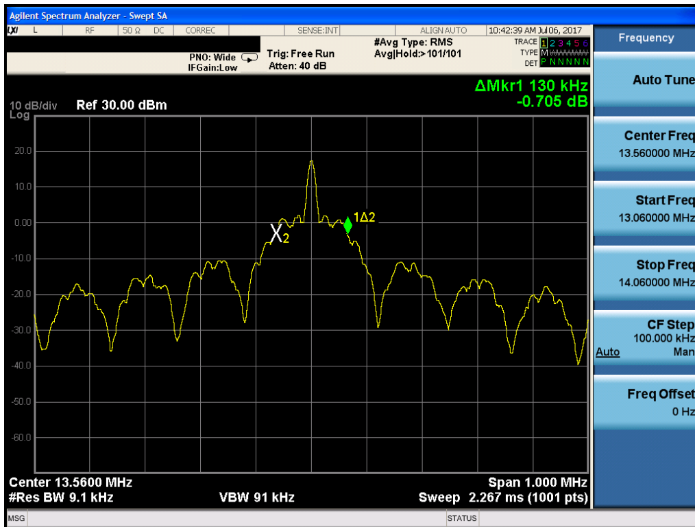
Figure 7-5. 20dB Bandwidth Plot (Reader 100% Ask 1 out of 4)
