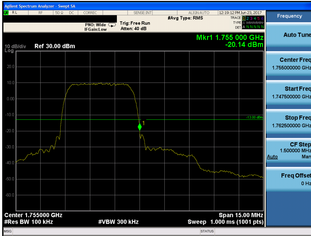
Plot 7-35. Band Edge Plot (AWS WCDMA Mode – Ch. 1513)
