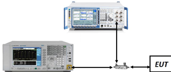
Figure 7-2. Test Instrument & Measurement Setup
