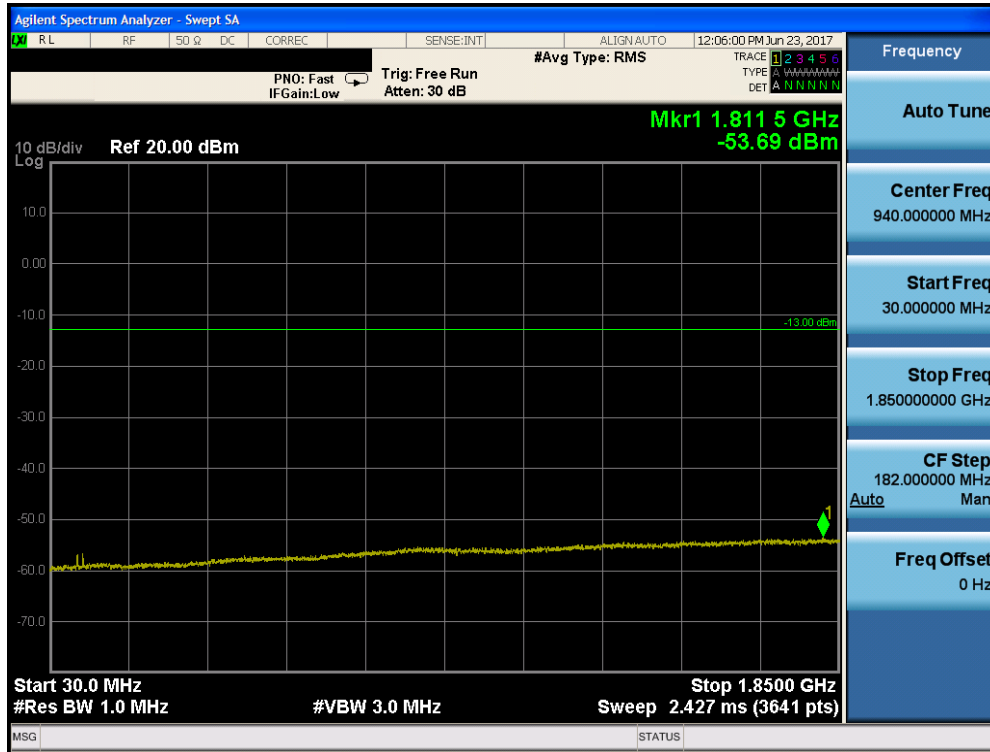
Plot 7-28. Conducted Spurious Plot (PCS WCDMA Mode – Ch. 9538)
