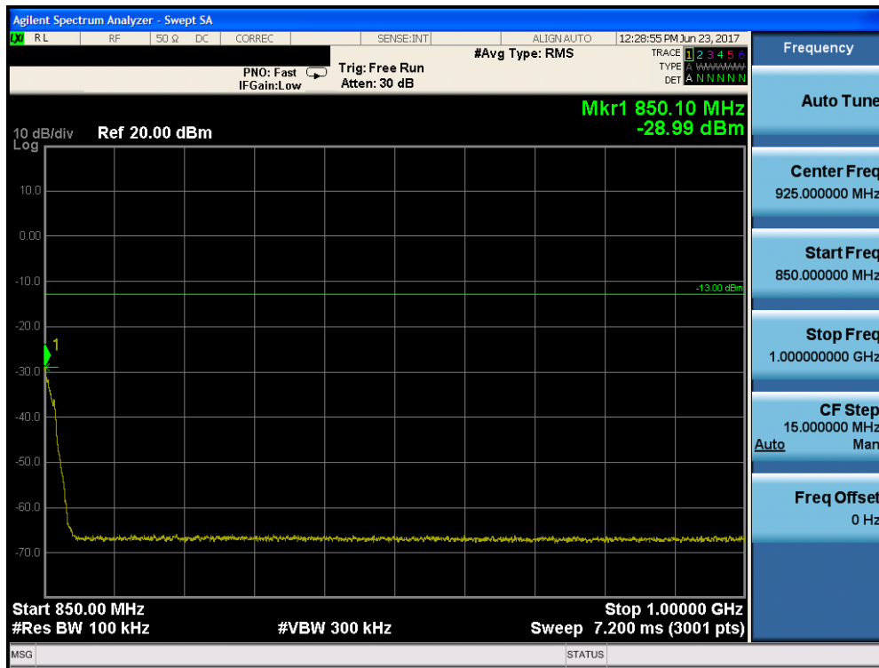
Plot 7-11. Conducted Spurious Plot (Cellular WCDMA Mode – Ch. 4233)
