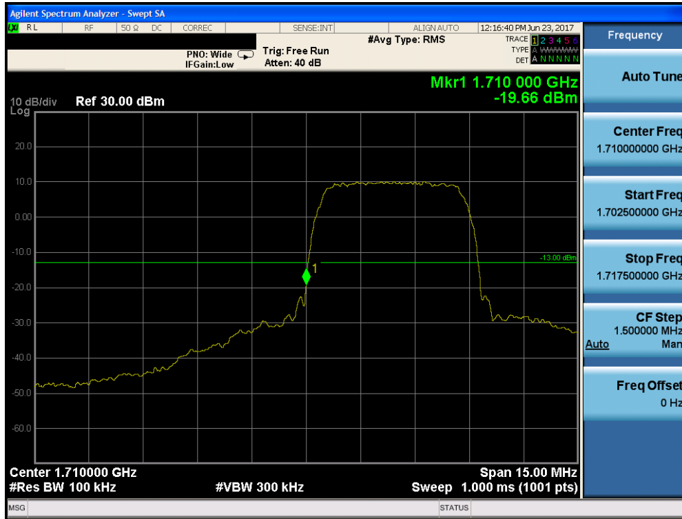
Plot 7-33. Band Edge Plot (AWS WCDMA Mode – Ch. 1312)
