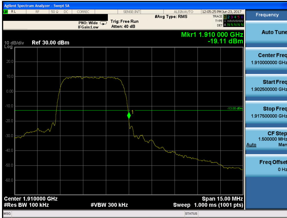
Plot 7-39. Band Edge Plot (PCS WCDMA Mode – Ch. 9538)
