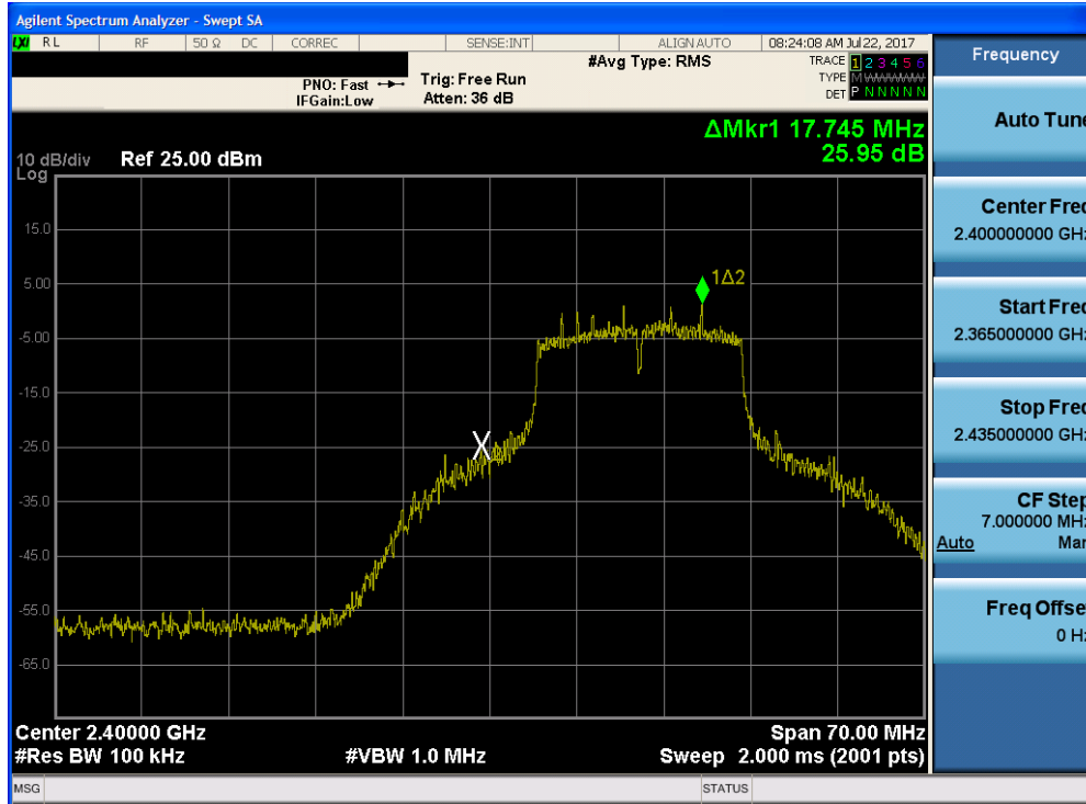
Plot 7-23. Band Edge Plot (802.11g– Ch. 1)
