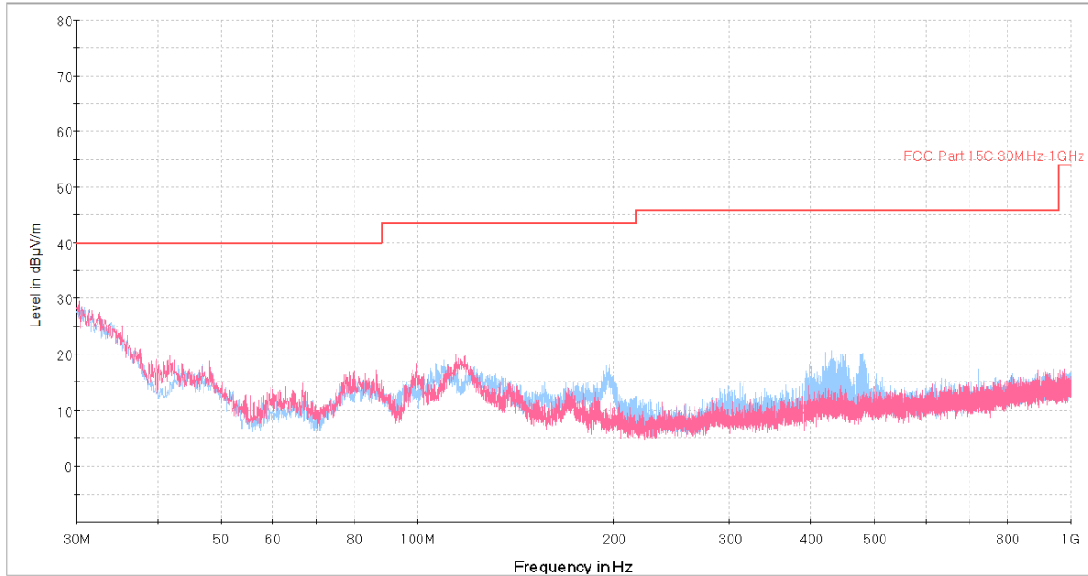
Plot 7-50. Radiated Spurious Plot below 1GHz (Pol. H & V)
