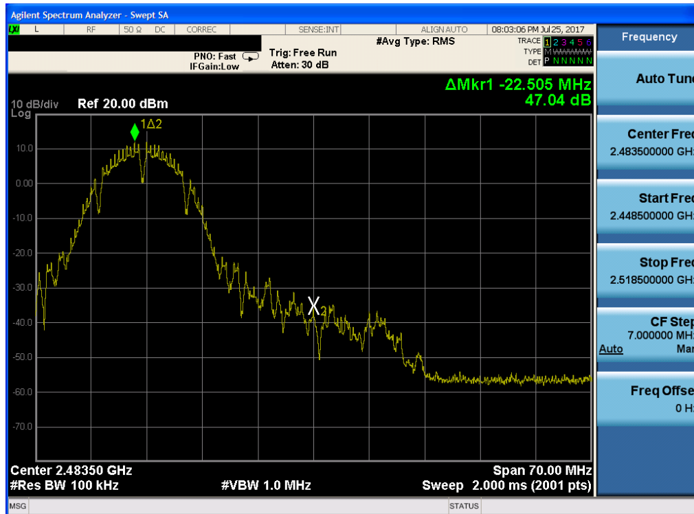
Plot 7-20. Band Edge Plot (802.11b – Ch. 11)
