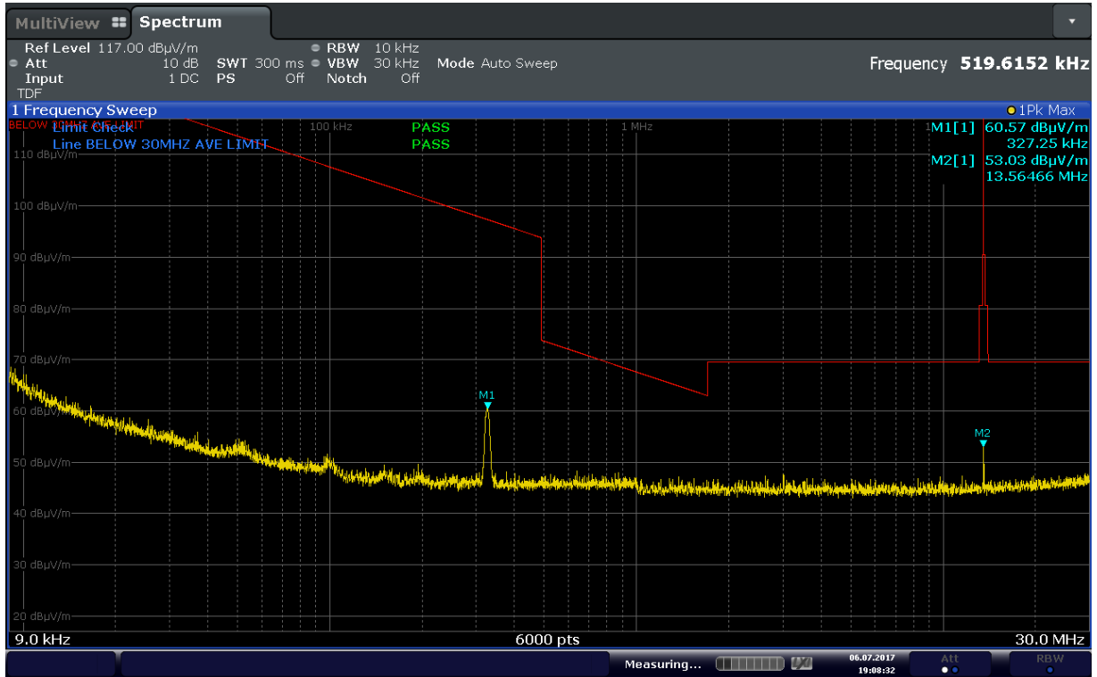
Plot 7-1. Radiated Spurious Plot 9kHz – 30MHz (Pol. X)
