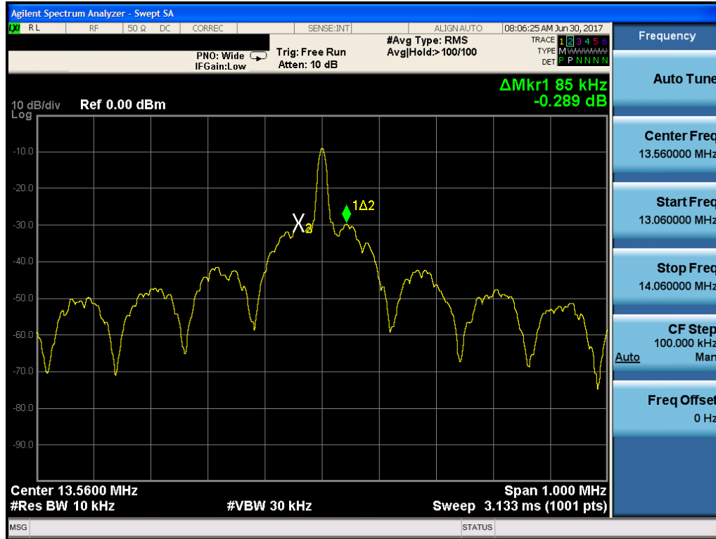
Figure 7-6. 20dB Bandwidth Plot (Reader 100% Ask 1 out of 256)
