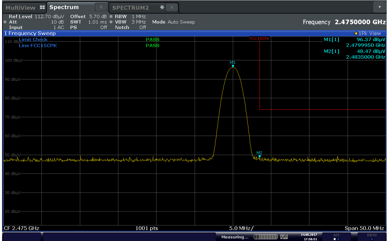
Plot 7-73. Radiated Restricted Upper Band Edge Measurement (Peak)
