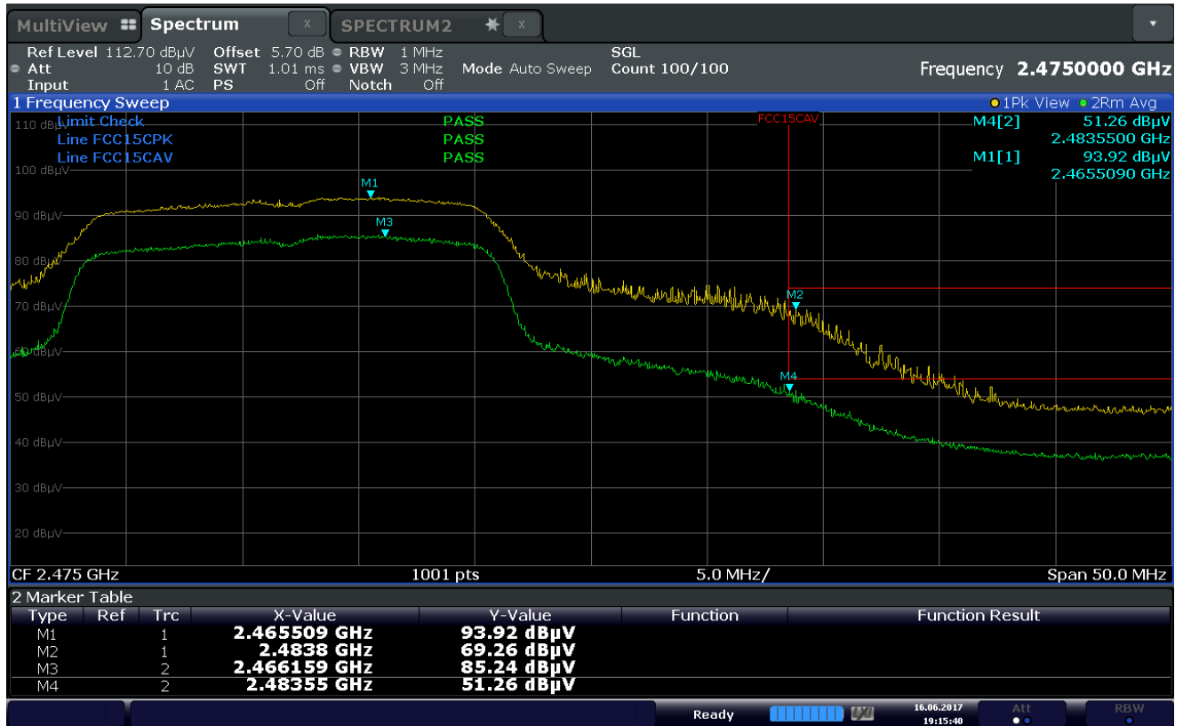
Plot 7-47. Radiated Restricted Upper Band Edge Measurement (Average & Peak)
