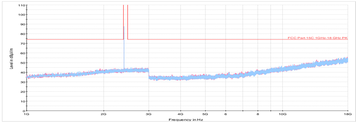
— Preview Result 1V-PK+ FCC Part 15C 1GHz-18 GHz PK ◆ Preview Result 1H-PK+ Final_Result PK+ ◆ Critical_Freqs PK+ Final_Result AVG Plot 7-29. Radiated Spurious Plot above 1GHz (GFSK ePA – Ch. 0, Ant. Pol. H & V)
