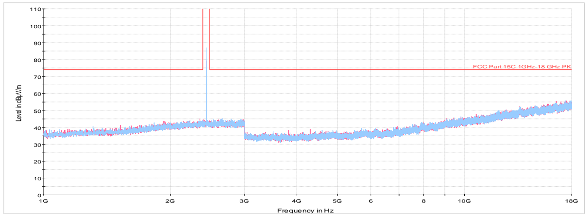
— Preview Result 1V-PK+ FCC Part 15C 1GHz-18 GHz PK ◆ Preview Result 1H-PK+ Final_Result PK+ ◆ Critical_Freqs PK+ Final_Result AVG Plot 7-30. Radiated Spurious Plot above 1GHz (GFSK ePA – Ch. 39, Ant. Pol. H & V)
