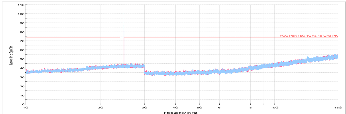
— Preview Result 1V-PK+ FCC Part 15C 1GHz-18 GHz PK ◆ Preview Result 1H-PK+ Final_Result PK+ ◆ Critical_Freqs PK+ Final_Result AVG Plot 7-31. Radiated Spurious Plot above 1GHz (GFSK ePA – Ch. 78, Ant. Pol. H & V)
