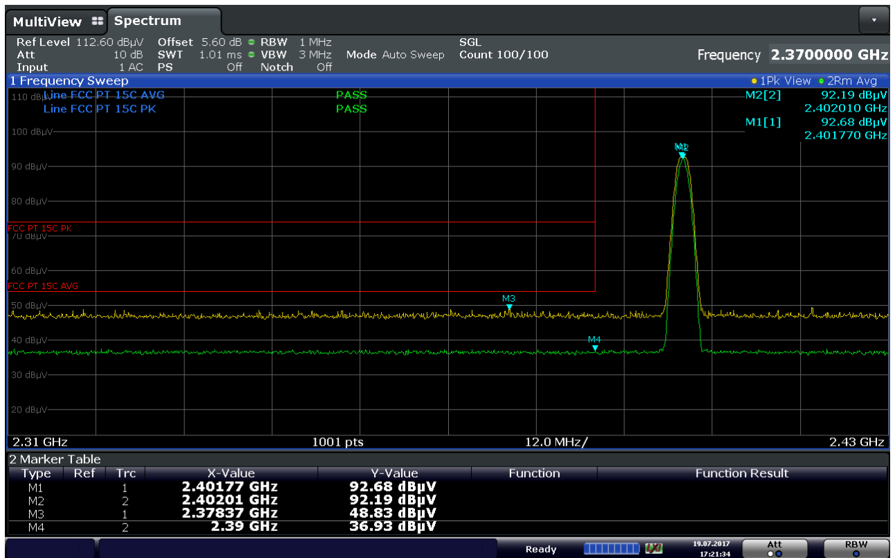
Plot 7-35. Radiated Restricted Lower Band Edge Measurement (Average & Peak)
