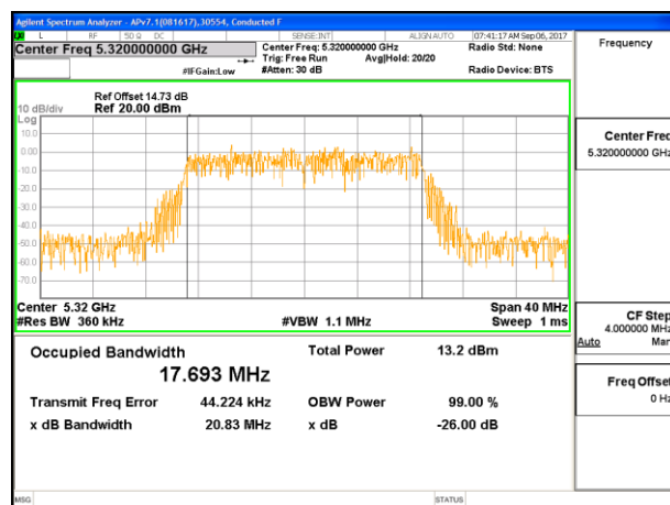
HIGH CHANNEL ANT B
